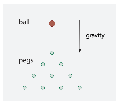
FIGURE 68 A system showing probabilistic behaviour: ball falling through an array of pegs.
