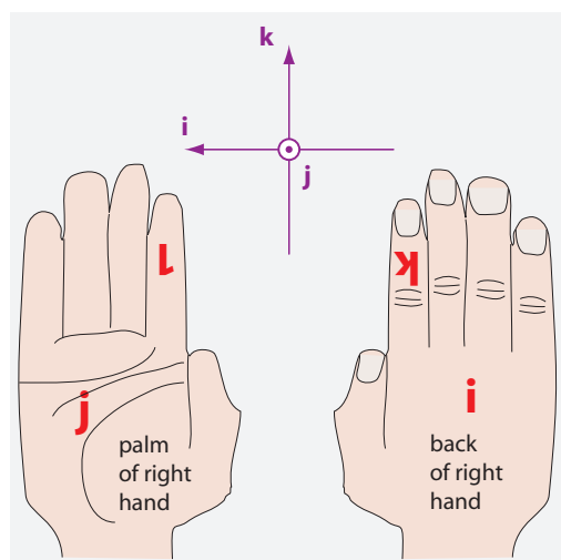
FIGURE 80 The top and back of the right hand, and the quaternions.
