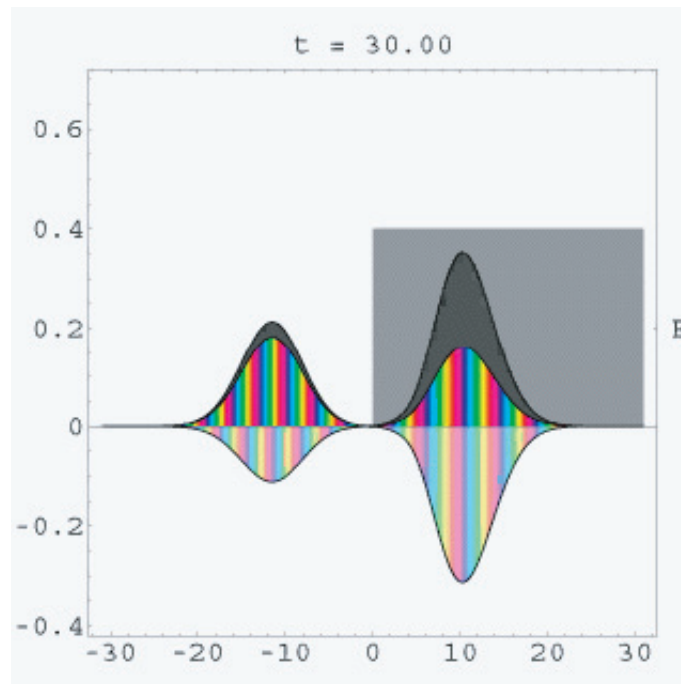
FIGURE 76 Klein's paradox: the motion of a relativistic wave function that encounters a very steep potential. Part of the wave function is transmitted; this part is antimatter, as the larger lower component shows. (QuickTime film © Bernd Thaller).
