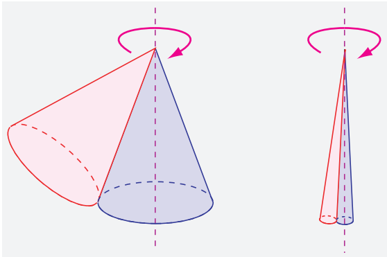
FIGURE 56 An argument showing why rotations by 4\pi are equivalent to no rotation at all.
