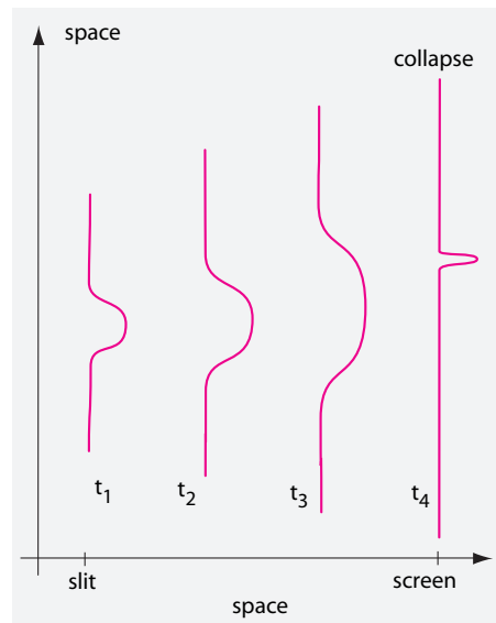
FIGURE 66 Quantum mechanical motion: an electron wave function (actually its module squared) from the moment it passes a slit until it hits a screen.
