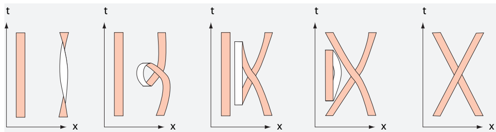
FIGURE 64 Belts in space-time: rotation and antiparticles.
