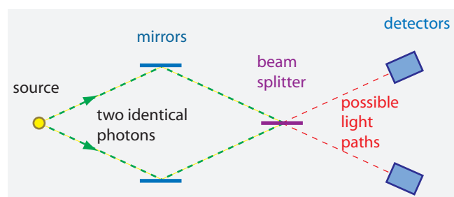
FIGURE 53 Two-photon emission and interference: both photons are always found arriving together, at the same detector.
