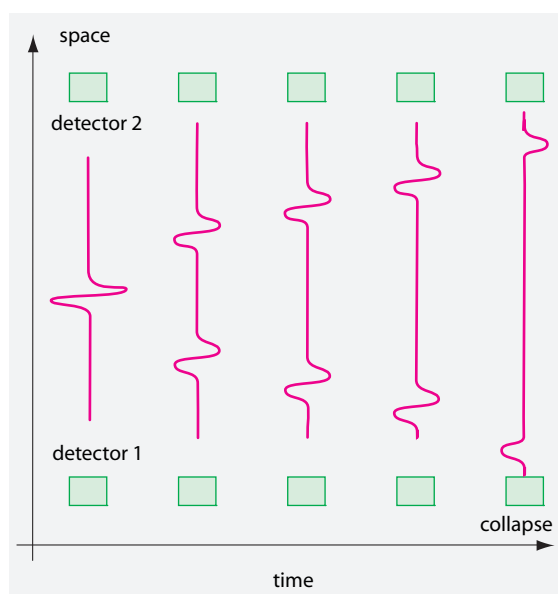
FIGURE 67 Bohm's Gedanken experiment.
