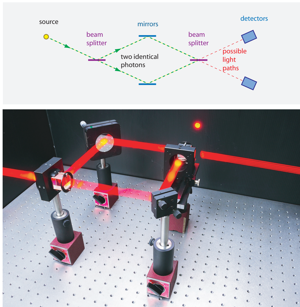
FIGURE 22 The Mach-Zehnder interferometer and a practical realization, about 0.5 m in size (© Félix Dieu and Gaël Osowiecki).
