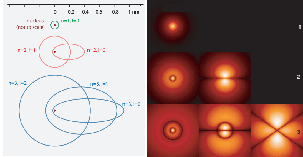
FIGURE 73 The imagined, but not existing and thus false electron orbits of the Bohr–Sommerfeld model of the hydrogen atom (left) and the correct description, using the probability density of the electron in the various states (right) (© Wikimedia).
