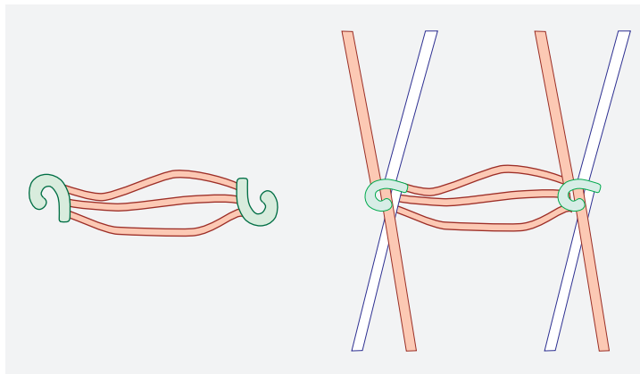
FIGURE 61 Extended belt models for two spin 1/2 particles.
