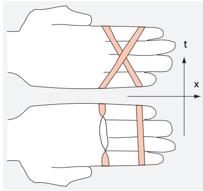
FIGURE 63 Equivalence of exchange and rotation in space-time.
