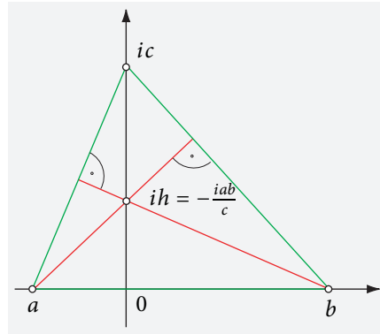
FIGURE 78 A property of triangles easily provable with complex numbers.
