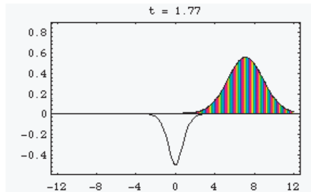
FIGURE 50 A special potential well that does not disturb a wave function. Colour indicates phase. (QuickTime film © Bernd Thaller).
