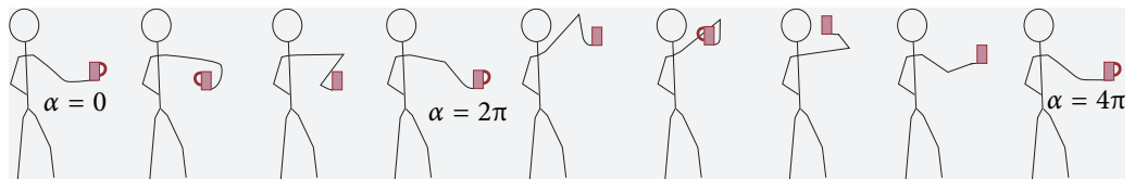
FIGURE 59 The human arm as spin 1/2 model.
