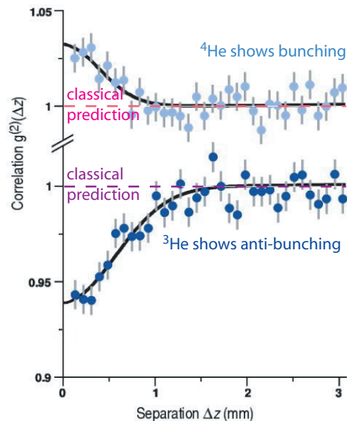
FIGURE 54 Bunching and antibunching of ^3\text{He} and ^4\text{He} helium atoms: the measurement result, the detector and the experiment (from atomoptic.iota.u-psud.fr/research/helium/helium.html , photo © Denis Boiron, Jerome Chatin).
