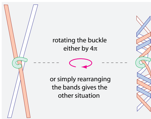
FIGURE 60 The extended belt trick, modelling the rotation behaviour of a spin 1/2 particle: independently of the number of bands or tubes or strings attached, the two situations can be transformed into each other, either by rotating the central object by 4\pi or by keeping the central object fixed and moving the bands around it.
