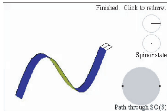
FIGURE 58 The belt trick: a double rotation of the belt buckle is equivalent to no rotation (QuickTime film © Greg Egan).
