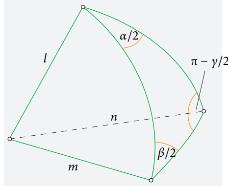
FIGURE 79 Combinations of rotations.
