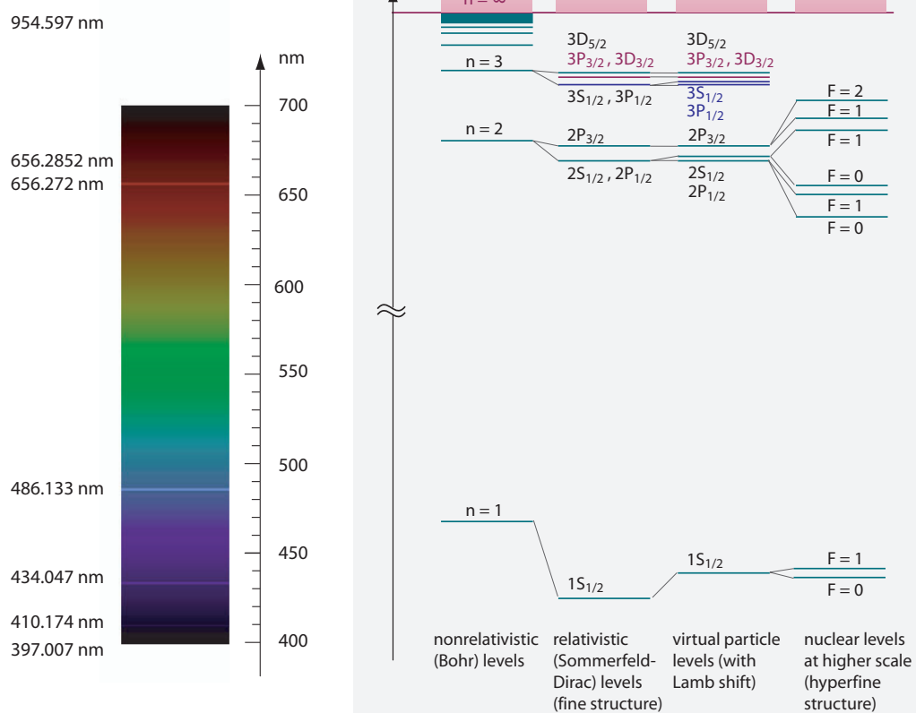
FIGURE 72 Atomic hydrogen: the visible spectrum of hydrogen (NASA) and its calculated energy levels, in four approximations of increasing precision. Can you associate the visible lines to the correct level transitions?
