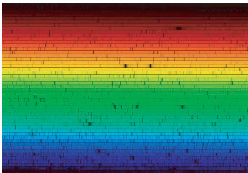
FIGURE 70 The spectrum of daylight: a stacked image of an extended rainbow, showing its Fraunhofer lines (© Nigel Sharp, NOAO, FTS, NSO, KPNO, AURA, NSF).
