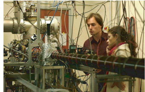
FIGURE 54 Bunching and antibunching of ^3\text{He} and ^4\text{He} helium atoms: the measurement result, the detector and the experiment (from atomoptic.iota.u-psud.fr/research/helium/helium.html , photo © Denis Boiron, Jerome Chatin).
