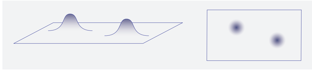
FIGURE 55 Picturing particles as localized excitations (left) or clouds (right).
