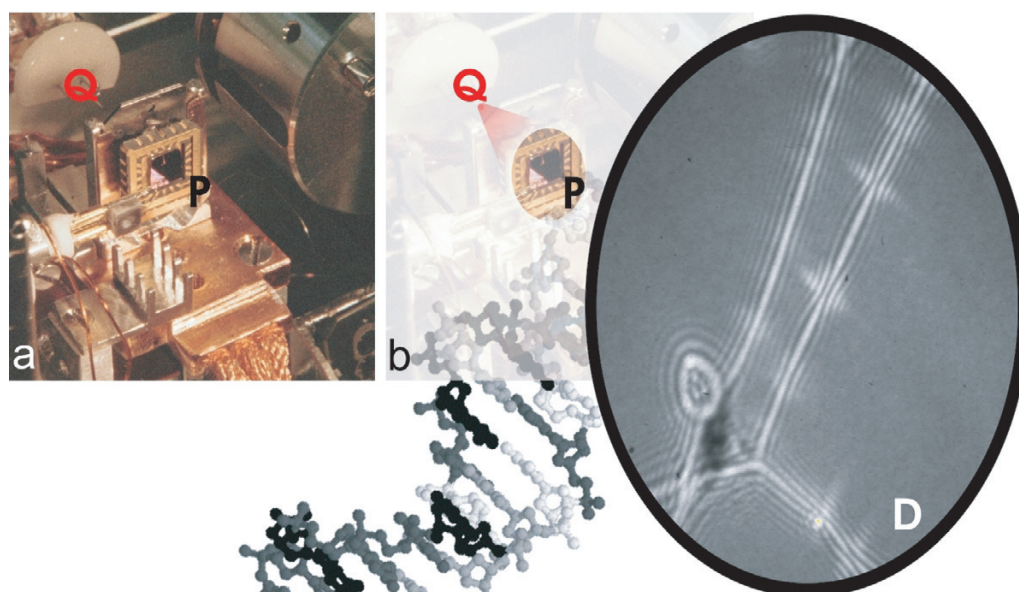
FIGURE 49 An electron hologram of DNA molecules (© Hans-Werner Fink/Wiley VCH).
