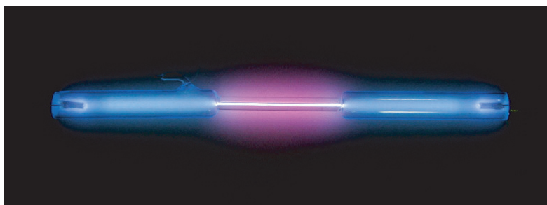
FIGURE 71 A low-pressure hydrogen discharge in a 20 cm long glass tube (© Jürgen Bauer at www.smart-elements.com ).
