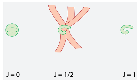
FIGURE 62 Some visualizations of spin representations.
