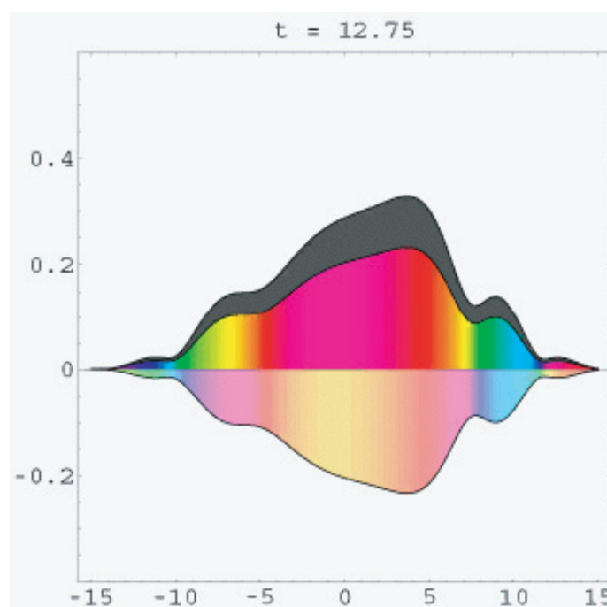
FIGURE 75 The famous Zitterbewegung: the superposition of positive and negative energy states leads to an oscillation around a mean value. Colour indicates phase; two coloured curves are shown, as the Dirac equation in one dimension has only two components (not four); the grey curve is the probability density. (QuickTime film © Bernd Thaller).
