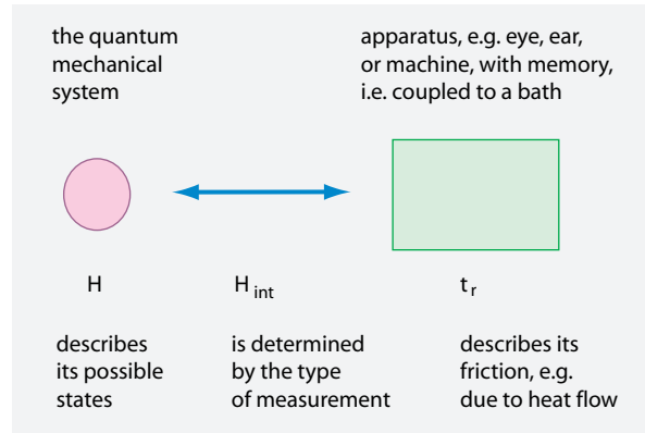
FIGURE 69 The concepts used in the description of measurements.
