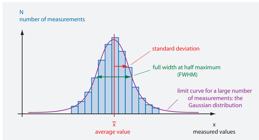
FIGURE 77 A precision experiment and its measurement distribution. The precision is high if the width of the distribution is narrow; the accuracy is high if the centre of the distribution agrees with the actual value.
