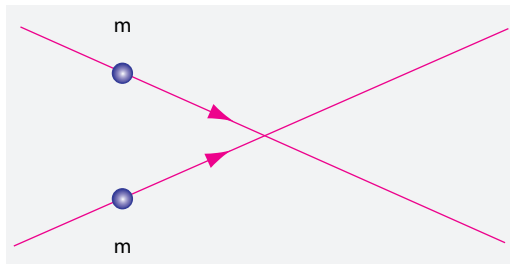
FIGURE 52 Identical objects with crossing paths.
