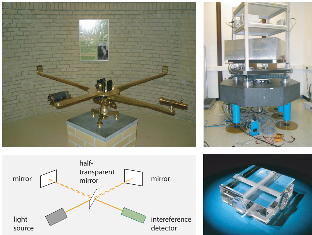
FIGURE 20 Testing the invariance of the speed of light on the motion of the observer: the reconstructed set-up of the first experiment by Albert Michelson in Potsdam, performed in 1881, and a modern high-precision, laser-based set-up that keeps the mirror distances constant to less than a proton radius and constantly rotates the whole experiment around a vertical axis (© Astrophysikalisches Institut Potsdam, Stephan Schiller).
