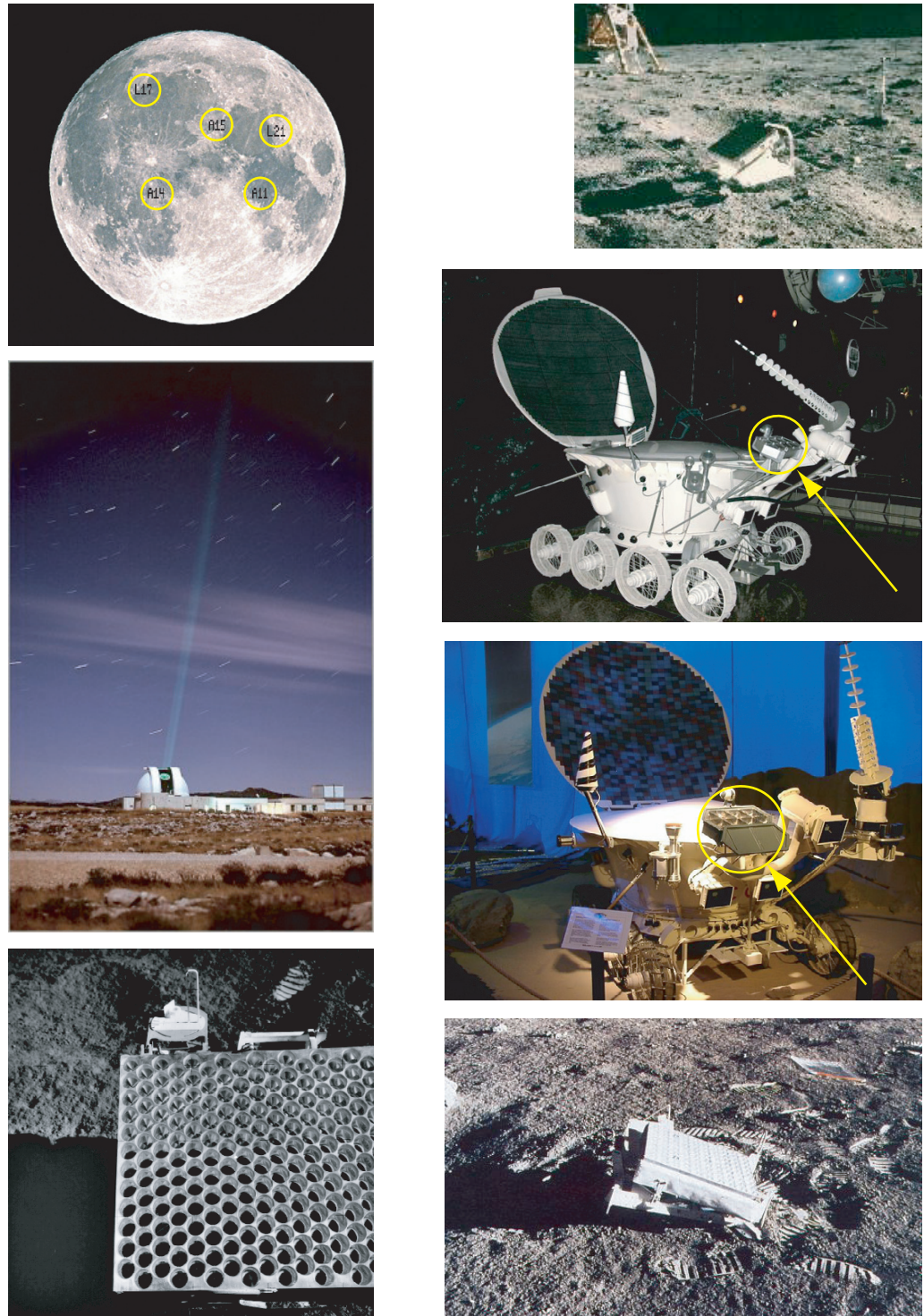
FIGURE 77 The lunar retroreflectors deposited by Apollo 11 (top right), the two Lunokhods (right), Apollo 14 (bottom right) and Apollo 15 (bottom left), their locations on the Moon (top left) and a telescope performing a laser distance measurement (© NASA, Observatoire de la Côte d'Azur).
