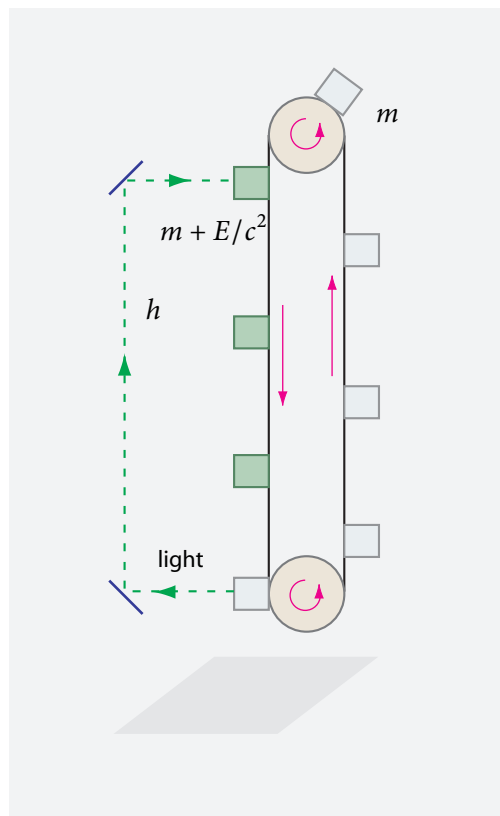
FIGURE 61 The necessity of blue- and red-shift of light: why trees are greener at the bottom.
