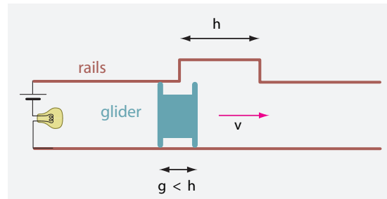
FIGURE 28 Does the conducting glider keep the lamp lit at large speeds?
