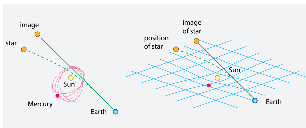
FIGURE 63 The mattress model of space: the path of a light beam and of a satellite near a spherical mass.
