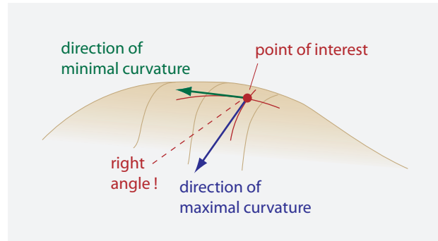
FIGURE 79 The maximum and minimum curvature of a surface are always at a right angle to each other.
