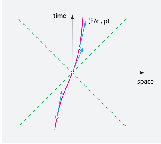
FIGURE 46 Energy-momentum is tangent to the world line.
