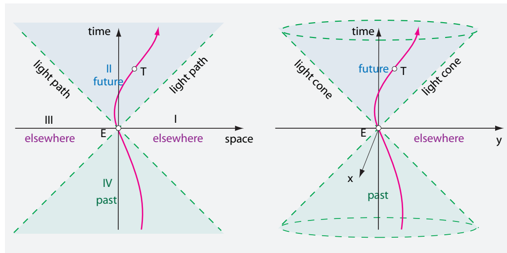
FIGURE 23 A space-time diagram for a moving object T seen from an inertial observer O in the case of one and two spatial dimensions; the slope of the world-line at a point is the speed at that point, and thus is never steeper than that of light.
