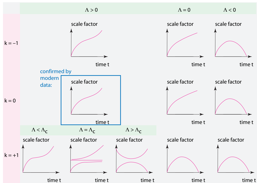
FIGURE 99 The long-term evolution of the universe's scale factor a for various parameters.
