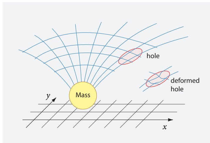
FIGURE 114 A 'hole' in space in a schematic view.
