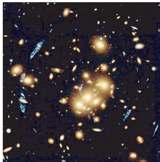
FIGURE 106 Multiple blue images of a galaxy formed by the yellow cluster CL0024+1654 (NASA).
