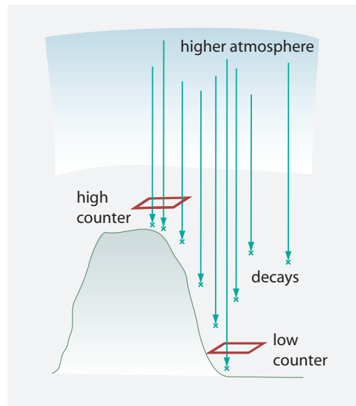
FIGURE 25 More muons than expected arrive at the ground because fast travel keeps them young.
