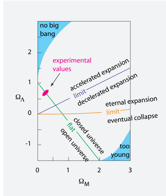
FIGURE 97 The ranges for the \Omega parameters and their consequences.
