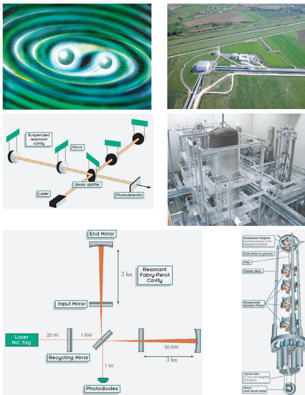
FIGURE 72 Detection of gravitational waves: an illustration of the merger of two black holes emitting such waves (top left). The other images show the VIRGO detector in Cascina, Italy, with one of its huge mirror suspensions, the mirror suspension details, and two drawings of the laser interferometer (© INFN).
