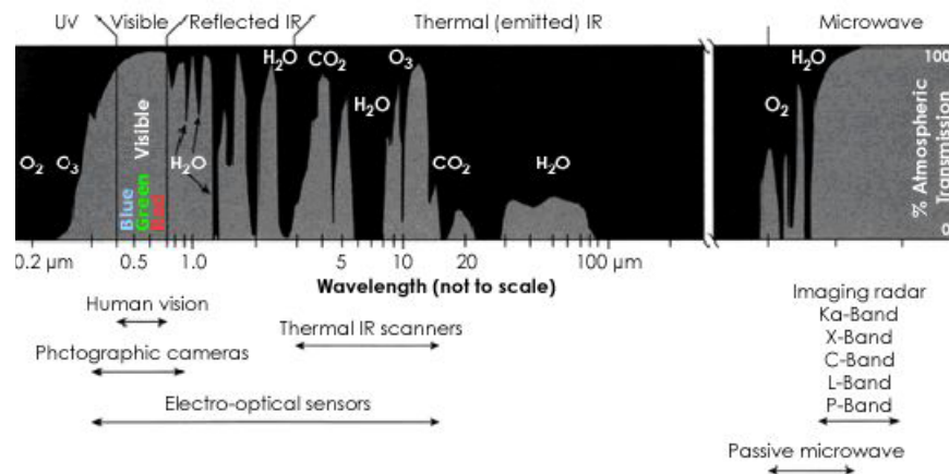
FIGURE 102 The transmittance of the atmosphere (NASA).
