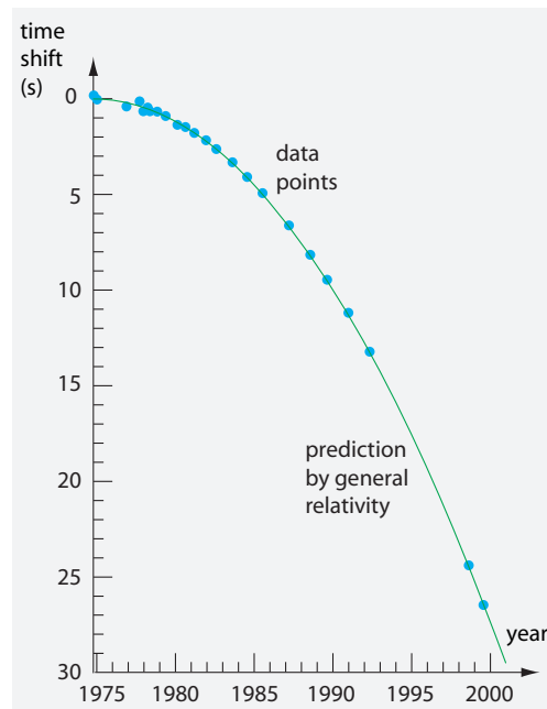
FIGURE 71 Comparison between measured time delay for the periastron of the binary pulsar PSR 1913+16 and the prediction due to energy loss by gravitational radiation.
