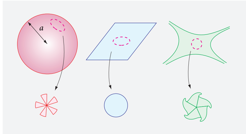
FIGURE 78 Positive, vanishing and negative curvature in two dimensions.
