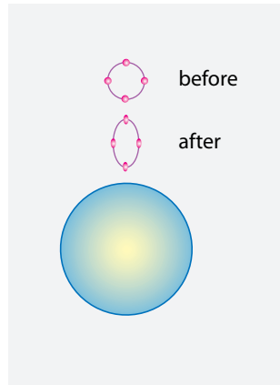
FIGURE 81 Tidal effects measure the curvature of space-time.
