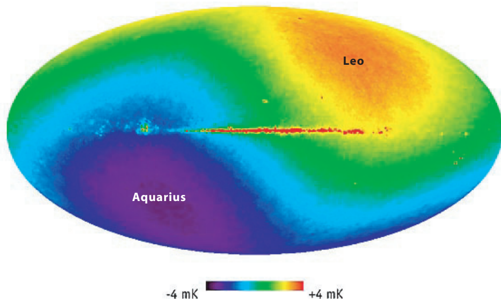
FIGURE 14 The Doppler effect for light from two quasars (left) and the – magnified, false colour – Doppler effect for the almost black colour of the night sky – the cosmic background radiation – due to the Earth travelling through space. In the latter case, the Doppler shift implies a tiny change of the effective temperature of the night sky (© Maurice Gavin, NASA).
