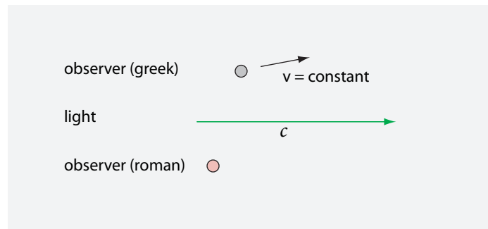
FIGURE 21 Two inertial observers and a beam of light. Both measure the same speed of light c .
