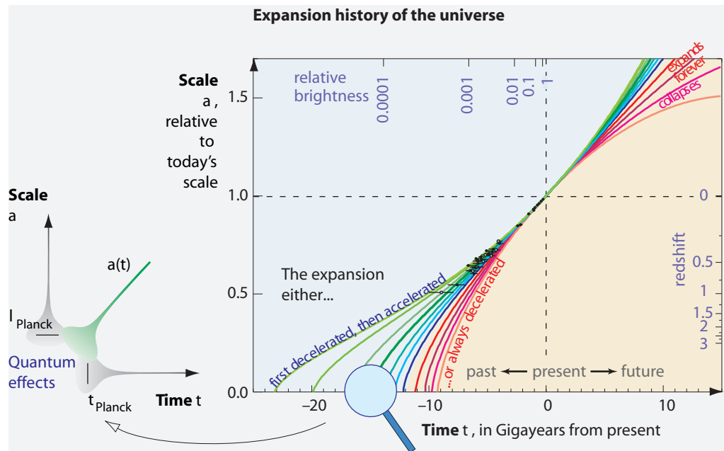
FIGURE 98 The evolution of the universe's scale a for different values of its mass density, as well as the measured data (the graph on the right is courtesy of Saul Perlmutter and the Supernova Cosmology Project).
