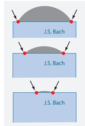
FIGURE 36 Another example of faster-than-light motion.
