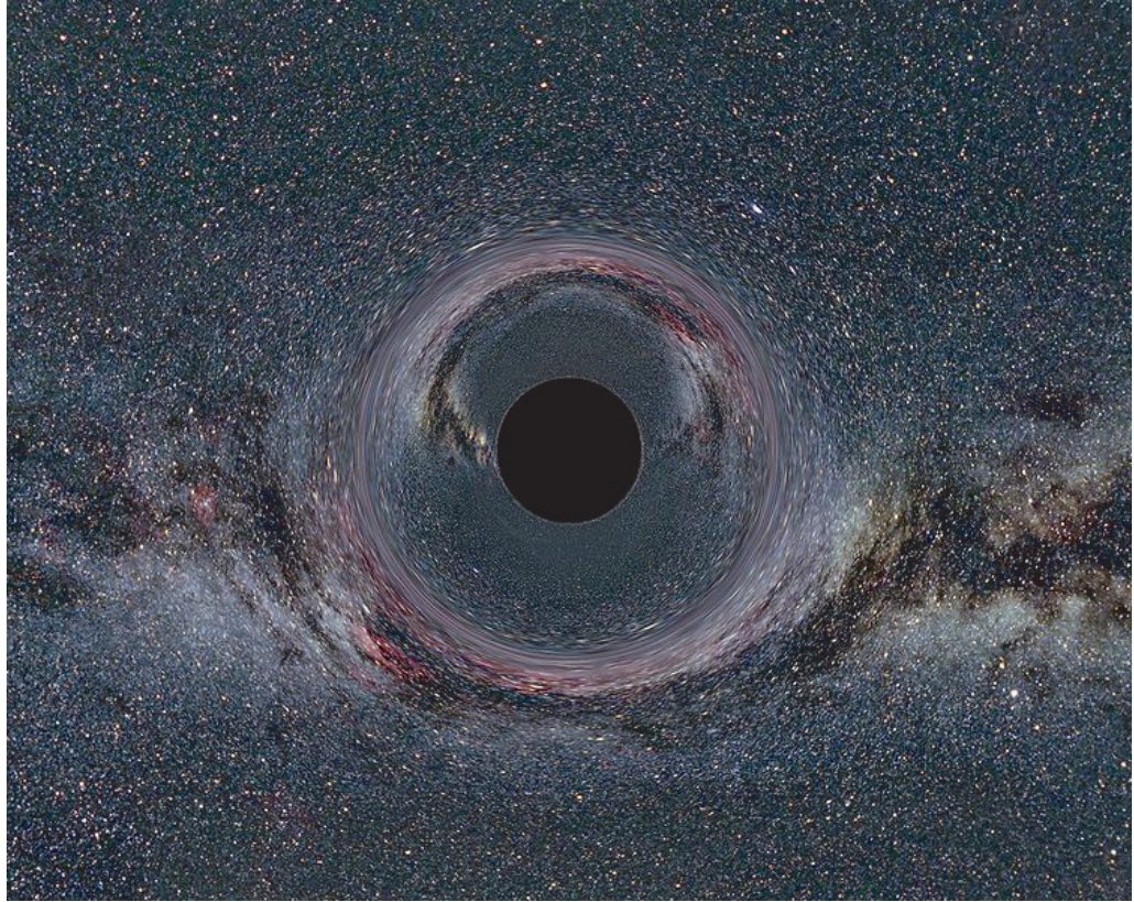
FIGURE 108 A simplified simulated image of how a black hole of ten solar masses, with Schwarzschild radius of 30 km, seen from a constant distance of 600 km, will distort an image of the Milky Way in the background. Note the Zwicky–Einstein ring formed at around twice the black hole radius and the thin bright rim (Image © Ute Kraus at www.tempolimit-lichtgeschwindigkeit.de ).
