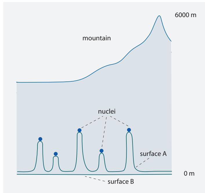
FIGURE 59 The mountain attempt to exceed the maximum mass flow value.
