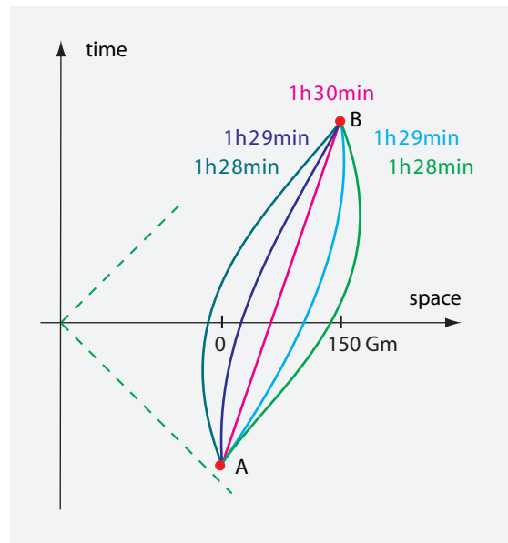
FIGURE 49 The straight motion between two points A and B is the motion that requires the longest proper time.
