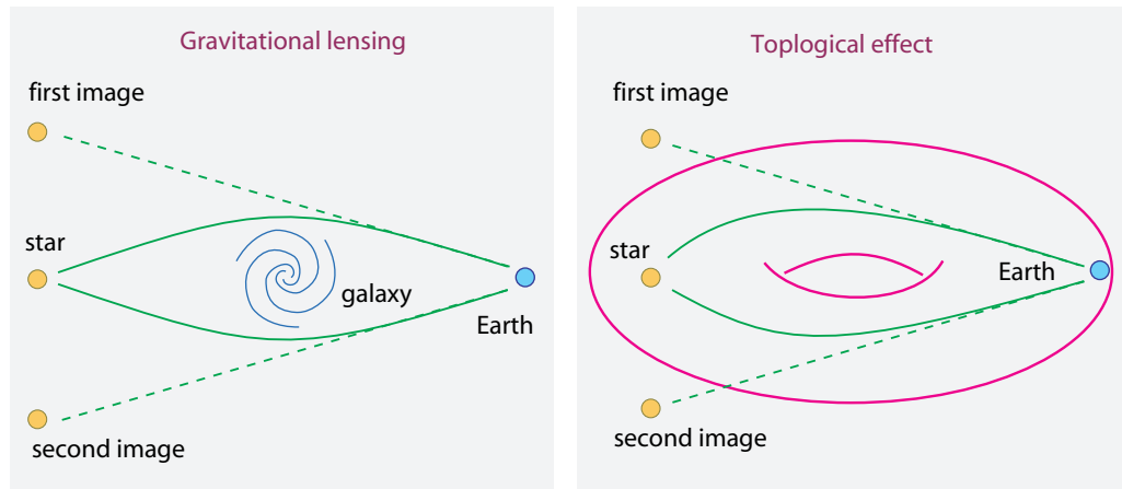
FIGURE 104 Two ways in which a single star can lead to several images.
