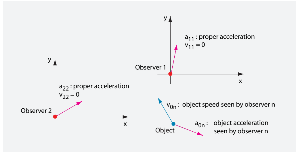
FIGURE 55 The definitions necessary to deduce the composition behaviour of accelerations.
