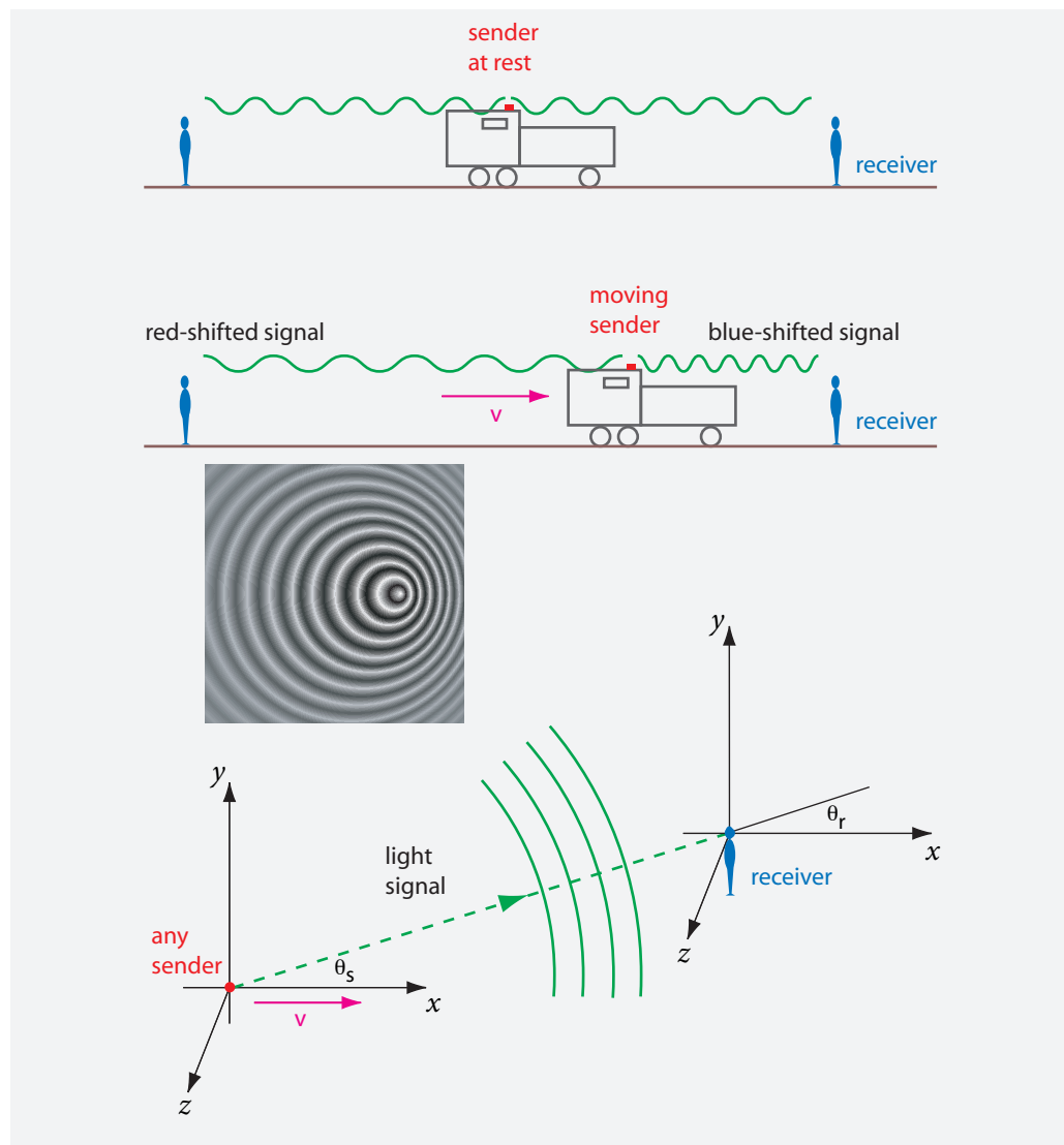
FIGURE 16 The set-up for the observation of the Doppler effect in one and three dimensions: waves emitted by an approaching source arrive with higher frequency and shorter wavelength, in contrast to waves emitted by a departing source (shadow waves courtesy Pbroks13/Wikimedia).
