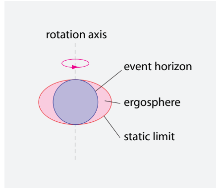
FIGURE 112 The ergosphere of a rotating black hole.
