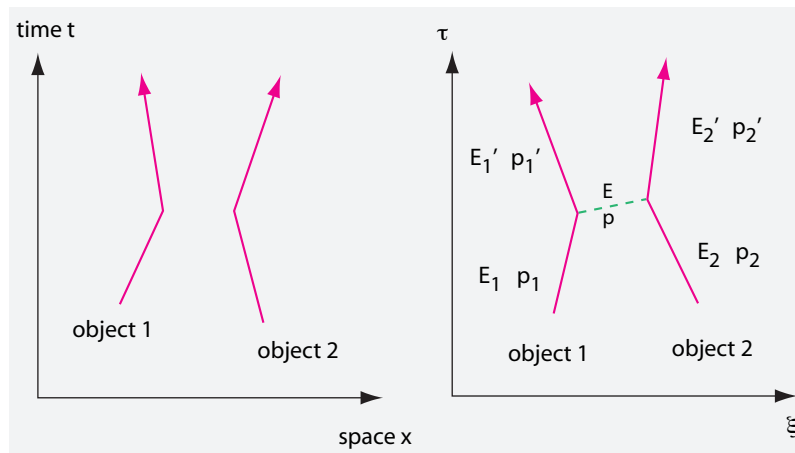
FIGURE 43 Space-time diagrams of the same collision for two different observers.
