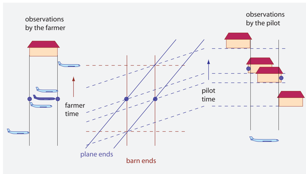
FIGURE 26 The observations of the pilot and the barn owner.
