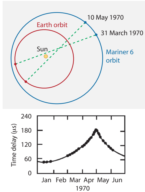
FIGURE 74 Time delay in radio signals – one of the experiments by Irwin Shapiro.
