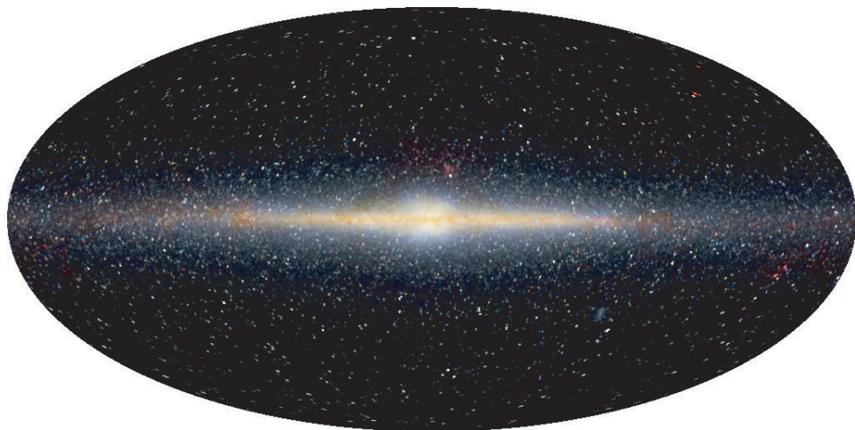
FIGURE 83 How the night sky, and our galaxy in particular, looks in the near infrared (NASA false colour image).
