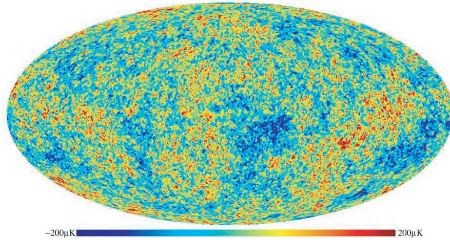
FIGURE 101 A false colour image of the fluctuations of the cosmic background radiation, after the Doppler shift from our local motion and the signals from the Milky Way have been subtracted (WMAP/NASA).
