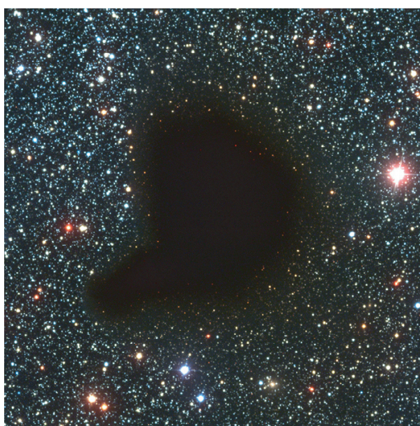
FIGURE 90 The universe contains many clouds; an example is this molecular cloud in Ophiuchus (© ESO).
