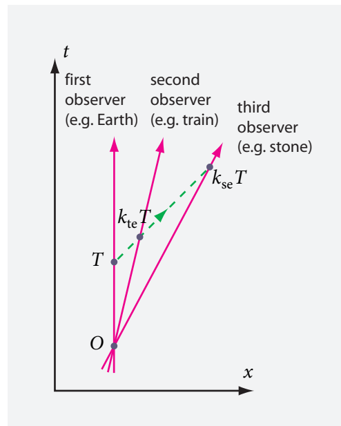
FIGURE 19 How to deduce the composition of velocities.
