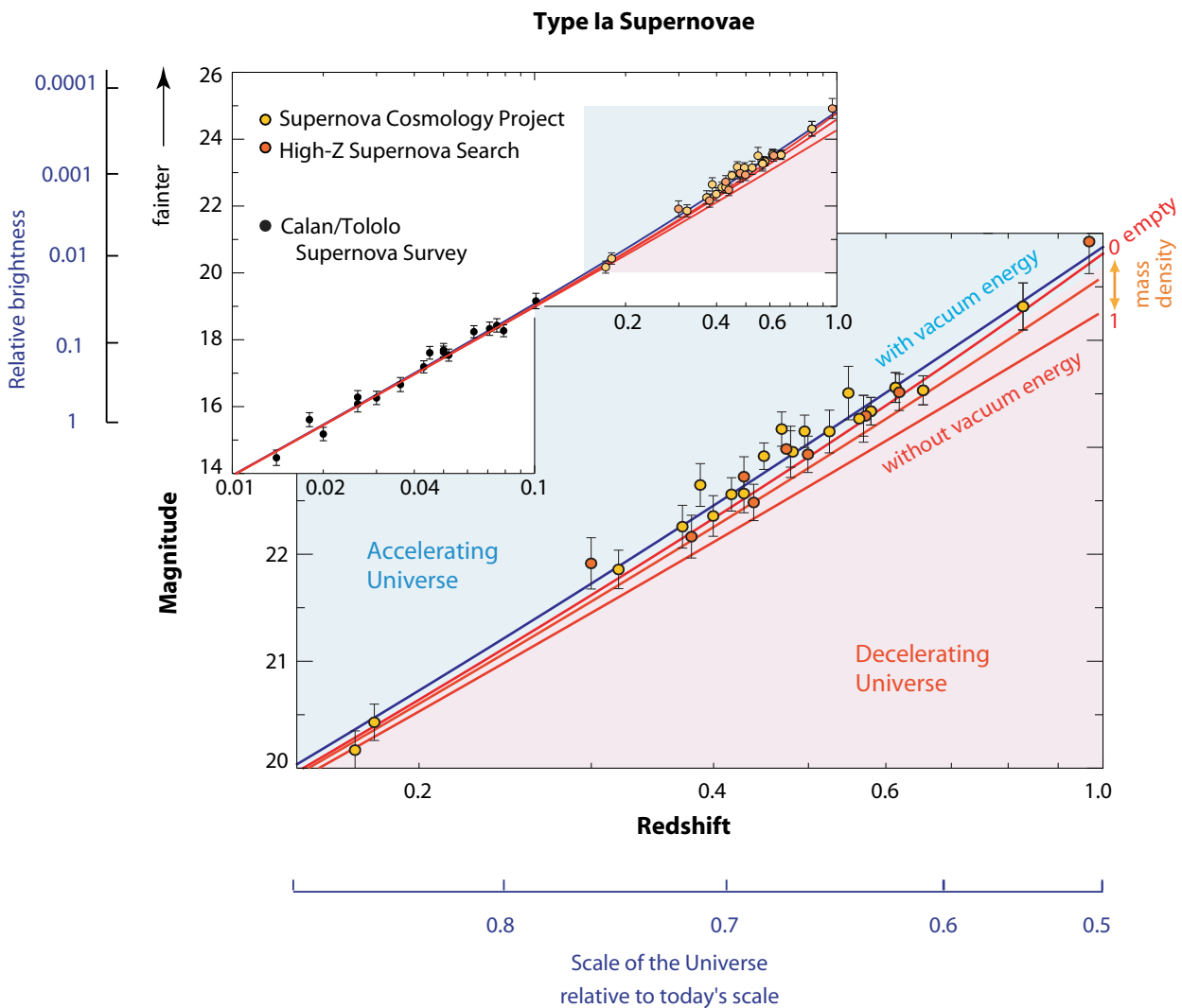
FIGURE 94 The relation between star distance and star velocity (courtesy Saul Perlmutter and the Supernova Cosmology Project).
