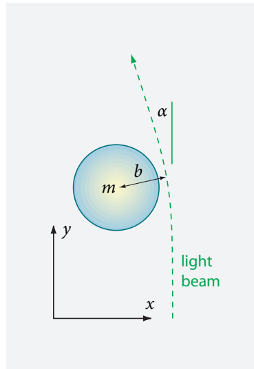
FIGURE 73 Calculating the bending of light by a mass.
