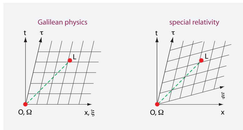
FIGURE 22 Space-time diagrams for light seen from two inertial observers, using coordinates (t, x) and (\tau, \xi) .
