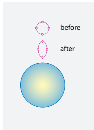
FIGURE 62 Tidal effects: the only effect bodies feel when falling.
