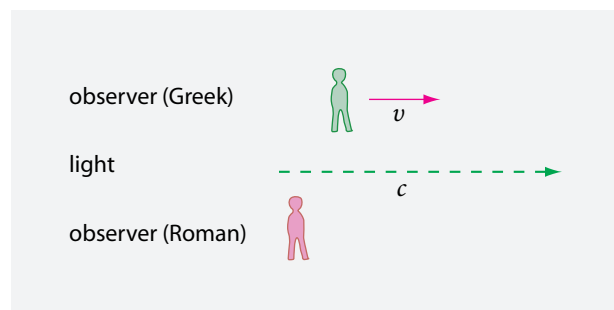
FIGURE 51 The simplest situation for an inertial and an accelerated observer.
