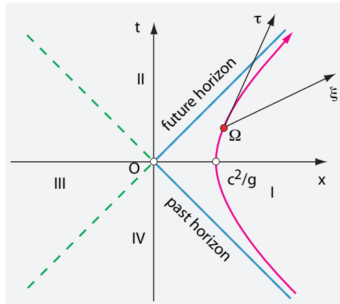
FIGURE 53 The hyperbolic motion of an rectilinearly, uniformly accelerating observer \Omega .
