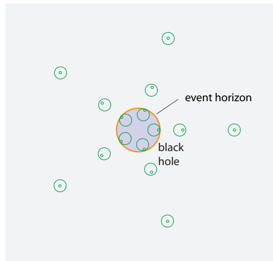
FIGURE 109 The light cones in the equatorial plane around a non-rotating black hole, seen from above the plane.
