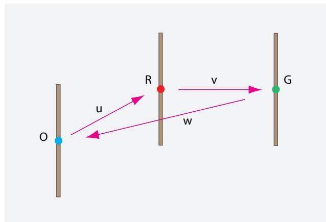
FIGURE 38 If O's stick is parallel to R's and R's is parallel to G's, then O's stick and G's stick are not.
