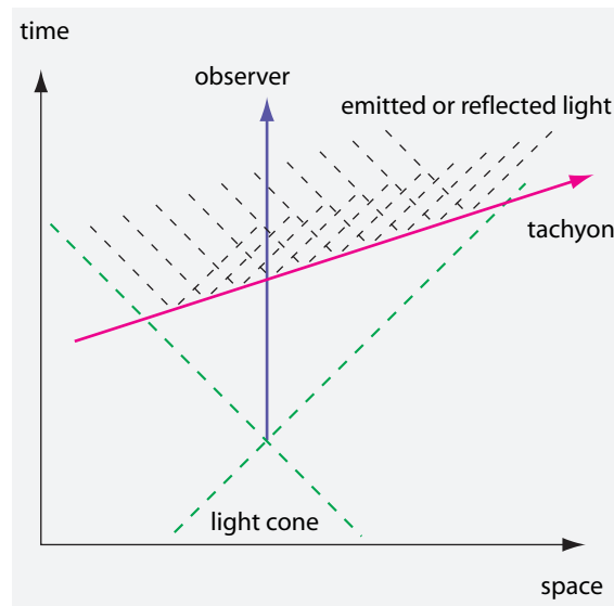
FIGURE 37 Hypothetical space-time diagram for tachyon observation.
