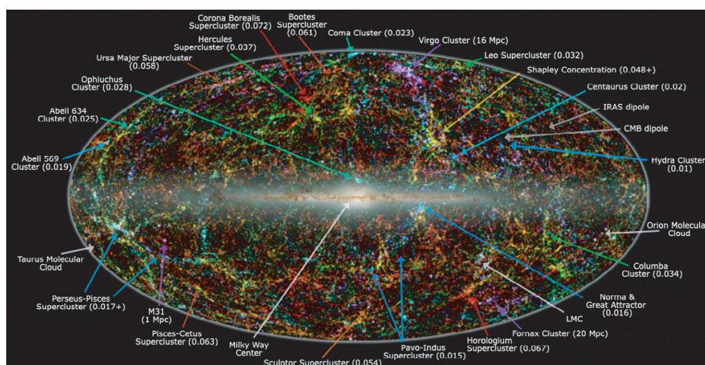
FIGURE 85 A false colour image, composed from infrared data, showing the large-scale structure of the universe around us; the colour of each galaxy represents its distance and the numbers in parentheses specify the redshift; an infrared image of the Milky Way is superposed (courtesy Thomas Jarrett/PAC/Caltech).
