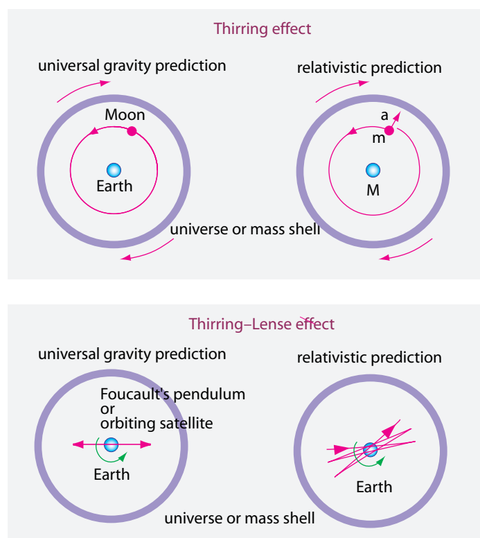
FIGURE 66 The Thirring and the Thirring-Lense effects.
