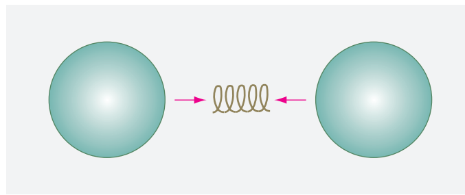
FIGURE 69 A Gedanken experiment showing the necessity of gravity waves.
