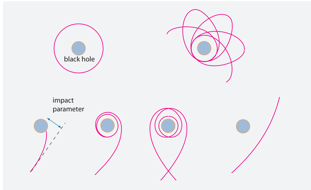
FIGURE 110 Motions of massive objects around a non-rotating black hole – for different impact parameters and initial velocities.
