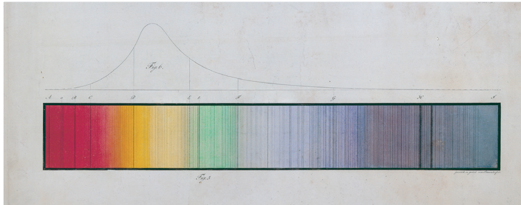
FIGURE 117 The original lines published by Fraunhofer (© Fraunhofer Gesellschaft).
