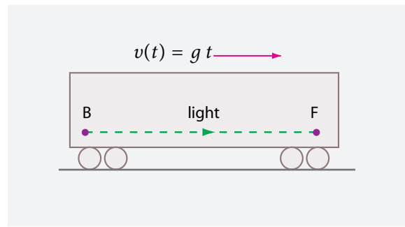
FIGURE 60 Inside an accelerating train or bus.
