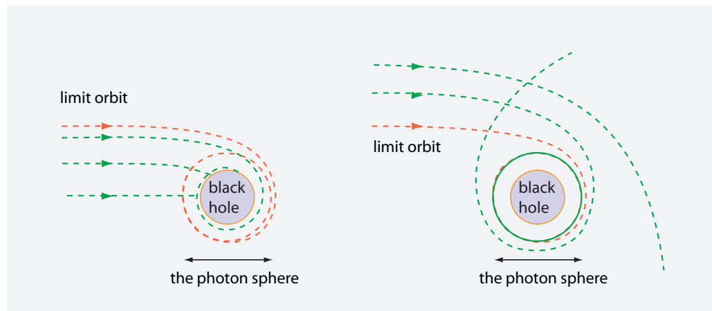
FIGURE 111 Motions of light passing near a non-rotating black hole.
