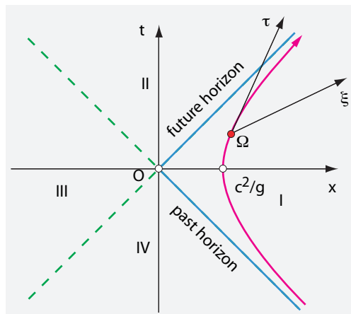
FIGURE 54 Hyperbolic motion and event horizons.
