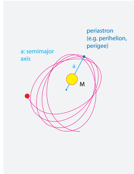
FIGURE 75 The orbit around a central body in general relativity.
