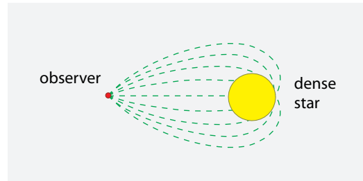
FIGURE 113 Motion of some light rays from a dense body to an observer.
