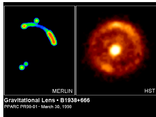
FIGURE 105 The Zwicky-Einstein ring B1938+666, seen in the radio spectrum (left) and in the optical domain (right) (NASA).
