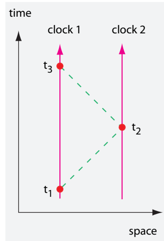
FIGURE 56 Clocks and the measurement of the speed of light as two-way velocity.
