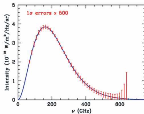
FIGURE 95 The measured spectrum of the cosmic background radiation, with the error bars multiplied by 500, compared to the calculated Planck spectrum for 2.728 K (NASA).
