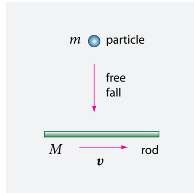
FIGURE 68 The reality of gravitomagnetism.
