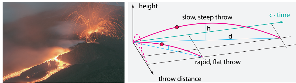
FIGURE 64 All paths of flying stones, independently of their speed and angle, have the same curvature in space-time (photograph © Marco Fulle).
