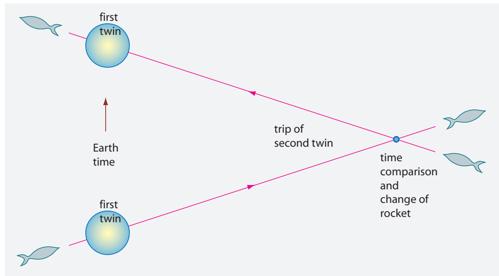
FIGURE 24 The twin paradox.
