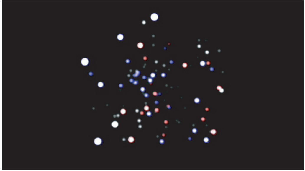
FIGURE 107 A time-lapse film, taken over a period of 16 years, of the orbits of the stars near the centre of our Galaxy. The invisible central object is so massive and small that it is almost surely a black hole (QuickTime film © ESO).
