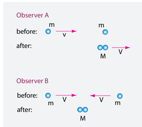
FIGURE 39 An inelastic collision of two identical particles seen from two different inertial frames of reference.
