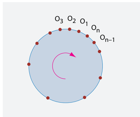
FIGURE 48 Observers on a rotating object.
