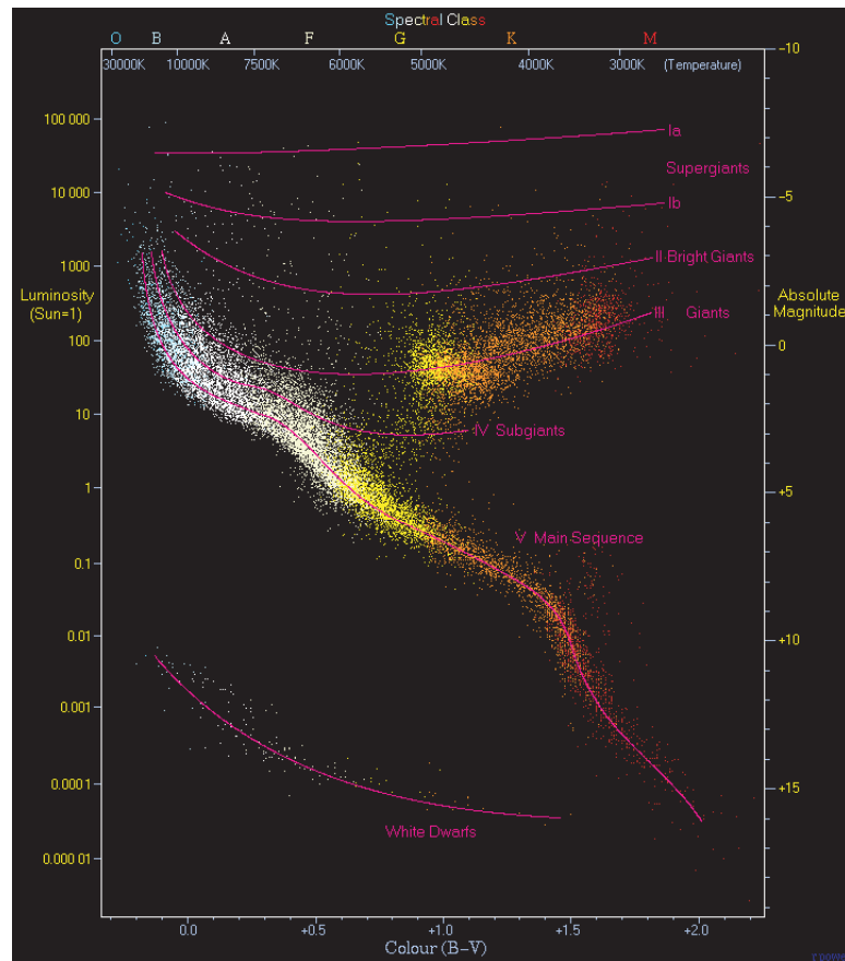
FIGURE 96 The Hertzsprung-Russell diagram (© Richard Powell).
