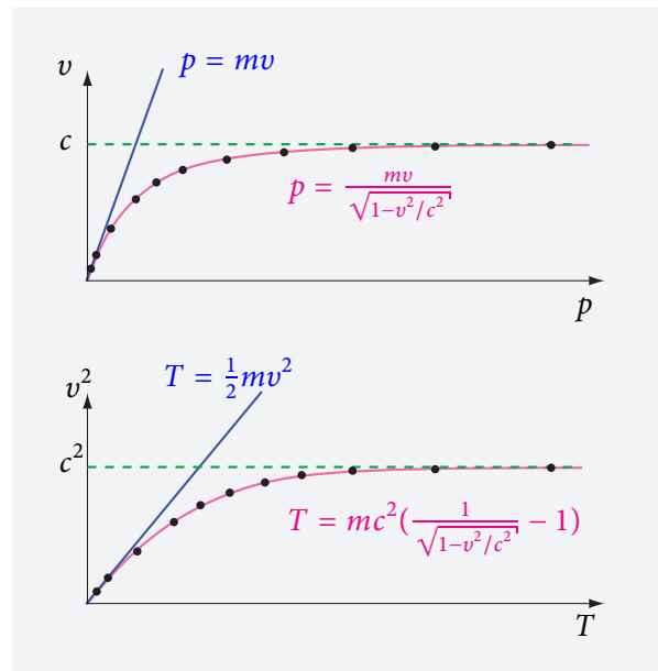
FIGURE 18 Experimental values (black dots) for the electron velocity v as function of their momentum p and as function of their kinetic energy T . The predictions of Galilean physics (blue) and the predictions of special relativity (red) are also shown.
