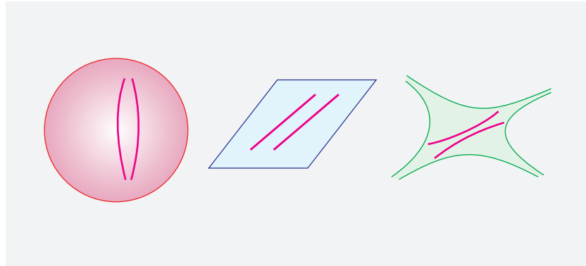
FIGURE 80 Positive, vanishing and negative curvature (in two dimensions) illustrated with the corresponding geodesic behaviour.
