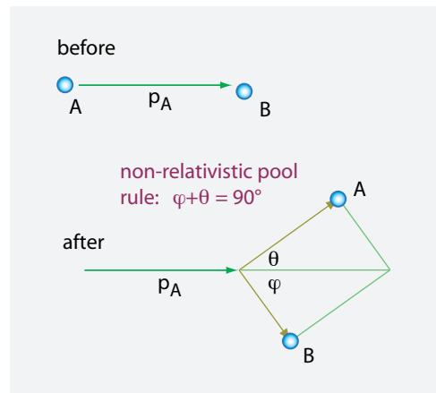
FIGURE 40 A useful rule for playing non-relativistic snooker.
