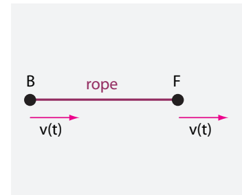
FIGURE 29 What happens to the rope?
