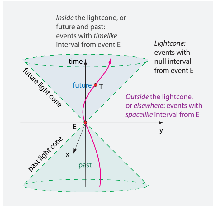
FIGURE 45 The space-time diagram of a moving object T , with one spatial dimension missing.
