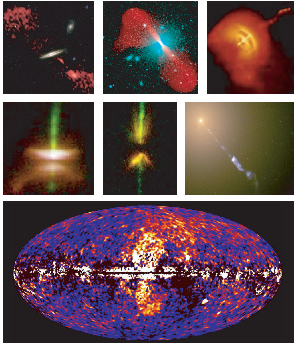
FIGURE 91 Rotating clouds emitting jets along their axis; top row: a composite image (visible and infrared) of the galaxy 0313-192, the galaxy 3C296, and the Vela pulsar; middle row: the star in formation HH30, the star in formation DG Tauri B, and a black hole jet from the galaxy M87; bottom row: the discovery of jets in our own galaxy (all NASA).
