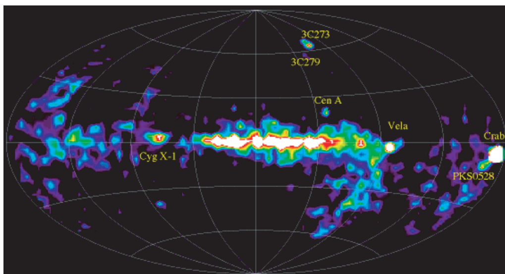
FIGURE 84 The X-rays observed in the night sky, for energies between 1 and 30 MeV (NASA).
