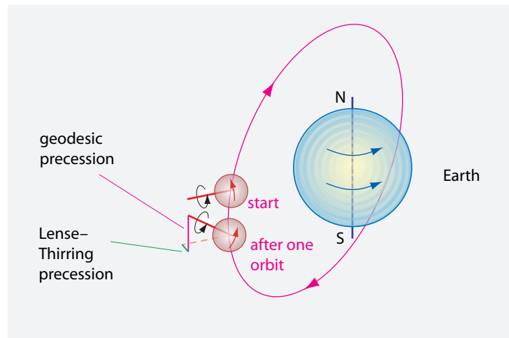
FIGURE 76 The geodesic effect.
