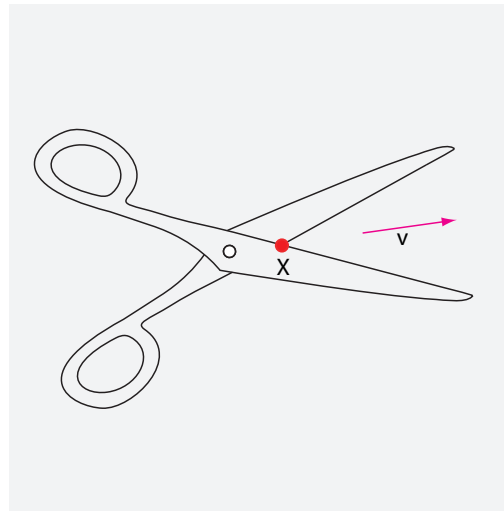
FIGURE 35 A simple example of motion that can be faster than light.
