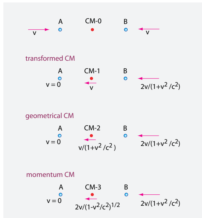
FIGURE 44 There is no consistent way to define a relativistic centre of mass.
