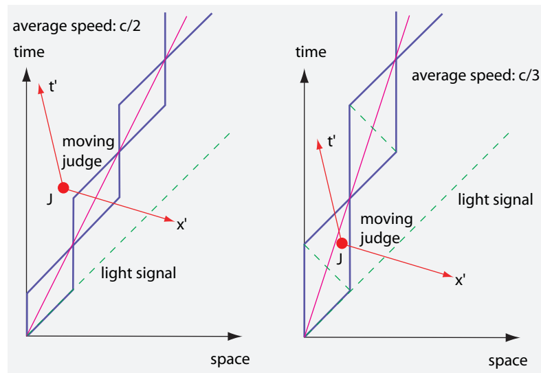
FIGURE 34 For the athlete on the left, the competition judge moving in the opposite direction sees both feet off the ground at certain times, but not for the athlete on the right.
