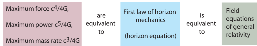
FIGURE 58 Showing the equivalence of the maximum force or power with the field equations of general relativity.
