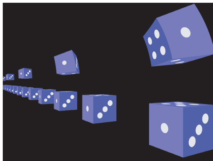
FIGURE 32 What a researcher standing and one running rapidly through a corridor observe (ignoring colour and brightness effects) (© Daniel Weiskopf).
