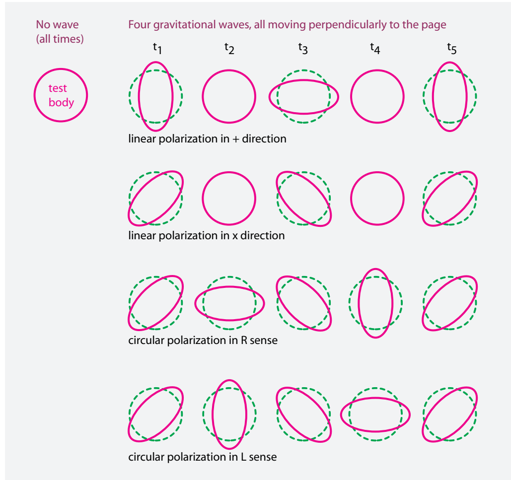
FIGURE 70 Effects on a circular or spherical body due to a plane gravitational wave moving in a direction perpendicular to the page.
