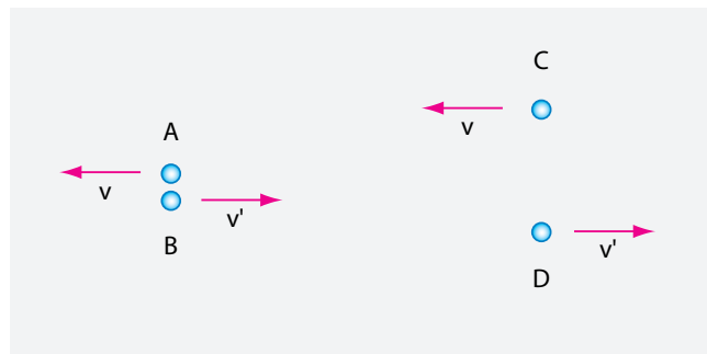
FIGURE 47 On the definition of relative velocity (see text).
