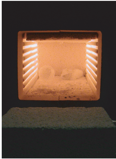
FIGURE 103 A hot red oven shows that at high temperature, objects and their environment cannot be distinguished from each other.
