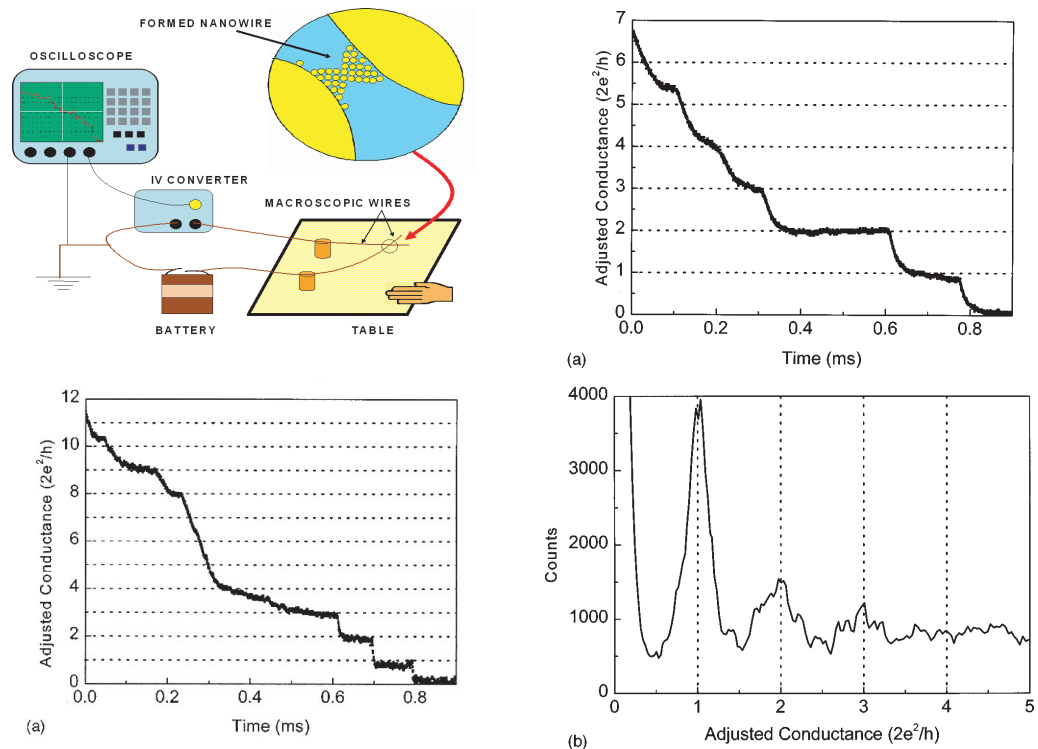
FIGURE 37 Steps in the flow of electricity in metal wire crossings: the set-up, the nanowires at the basis of the effect, and three measurement results (© José Costa-Krämer, AAPT from Ref. 39).
