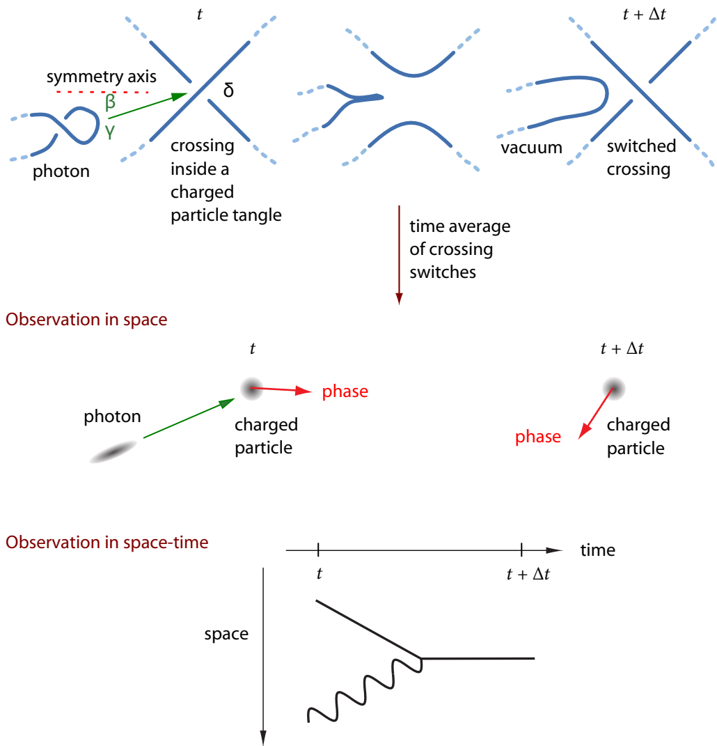
FIGURE 125 The geometric details of the basic process of quantum electrodynamics (QED). Top: the absorption of a photon by a tangle region carrying the charge e/3 , viewed along the shortest distance of the crossing. Centre: the corresponding observation at usual experimental scales. Bottom: the basic Feynman diagram of QED. In short: twist transfer generates minimal coupling and determines the electromagnetic gauge coupling strength, thus the fine structure constant.
