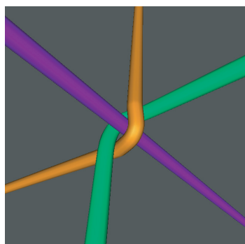
FIGURE 108 A discarded candidate tangle for the W boson.
