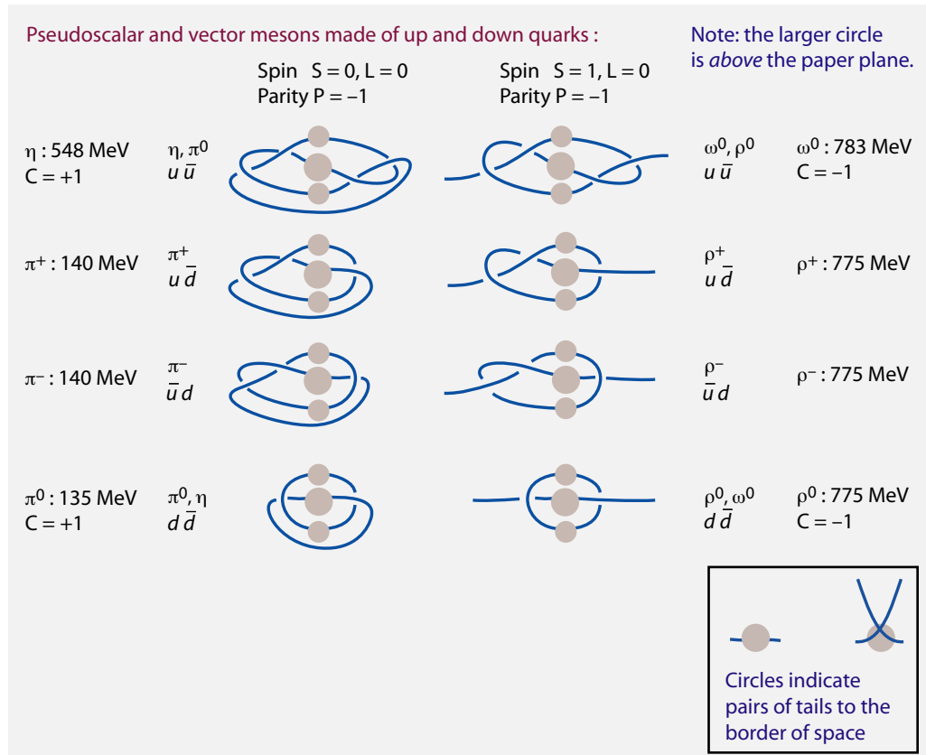
FIGURE 96 The simplest strand models for the light pseudoscalar and vector mesons (circles indicate crossed tail pairs to the border of space), with the observed mass values.
