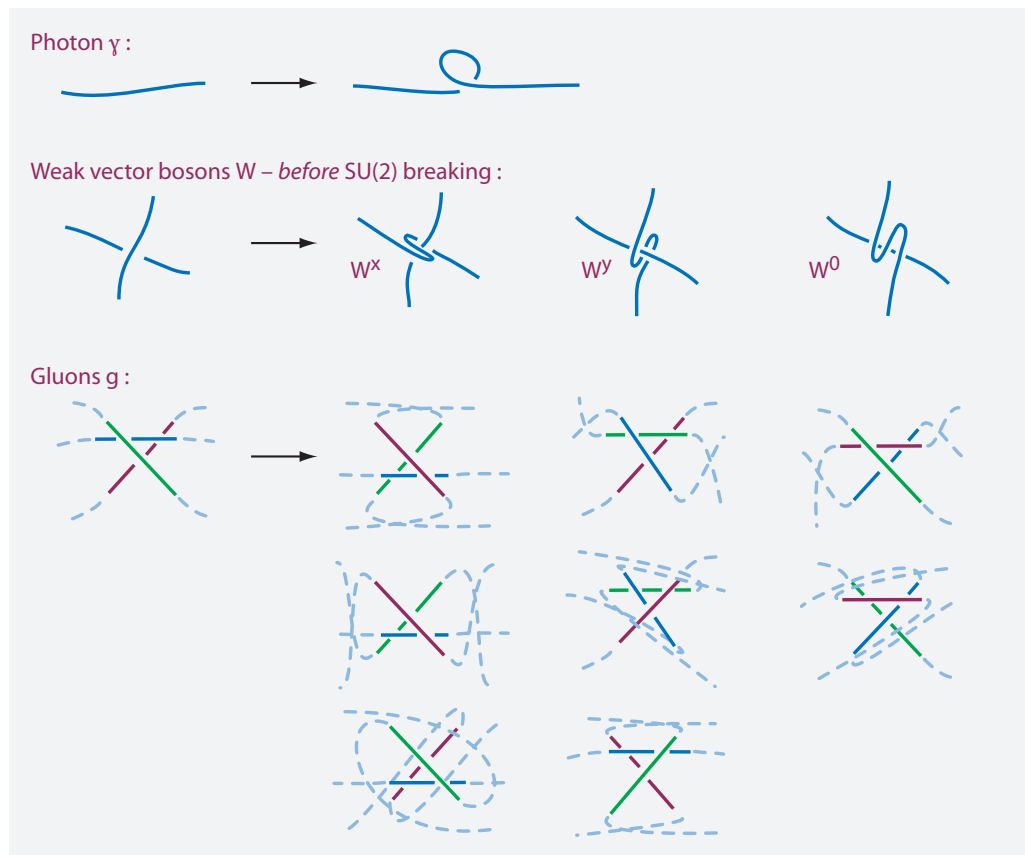
FIGURE 83 The gauge bosons in the strand model. All differ from vacuum by one curved strand – though, for clarity, the gluons are shown here using their complementary two-strand moves.
