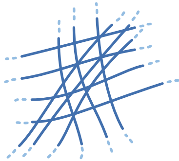
FIGURE 130 An illustration of the strand conjecture for a flat vacuum: for sufficiently long time scales, the lack of crossing switches leads to a vanishing energy density; for short time scales, particle–antiparticle pairs, i.e., rational tangle–antitangle pairs, arise.
