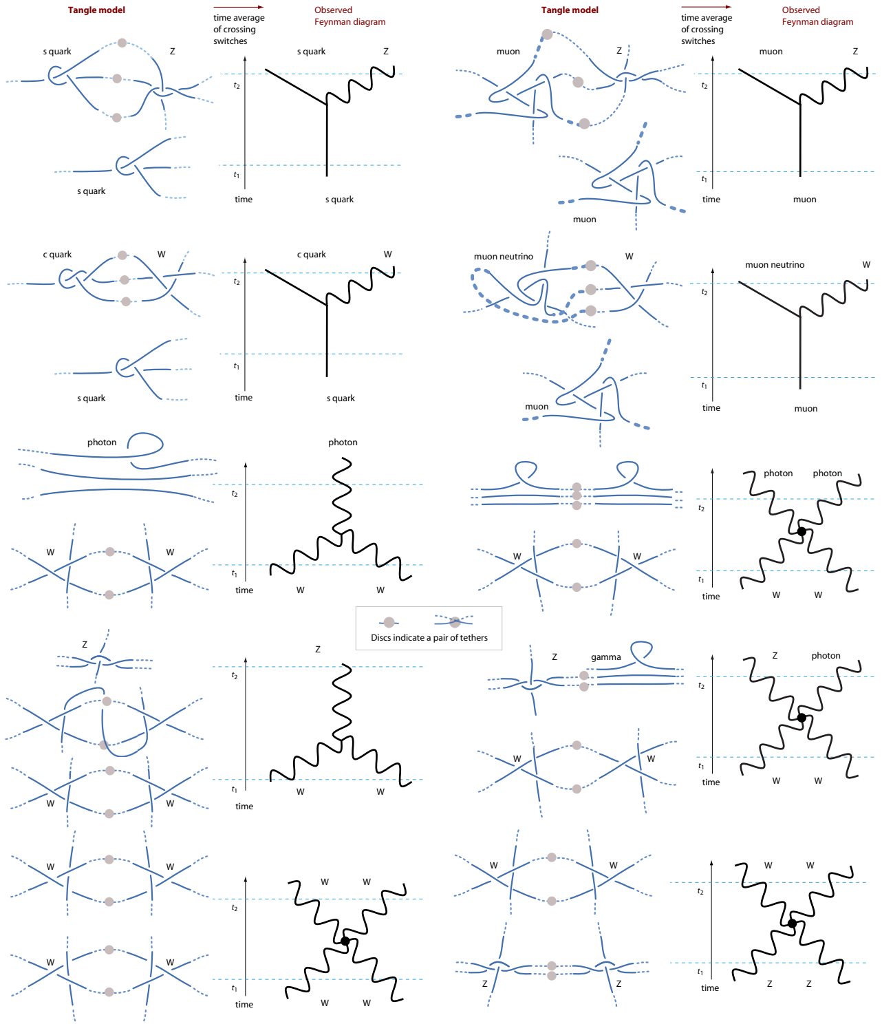
FIGURE 128 The vertices in Feynman diagrams allowed by the topology of the fermion and boson tangles (part one).
