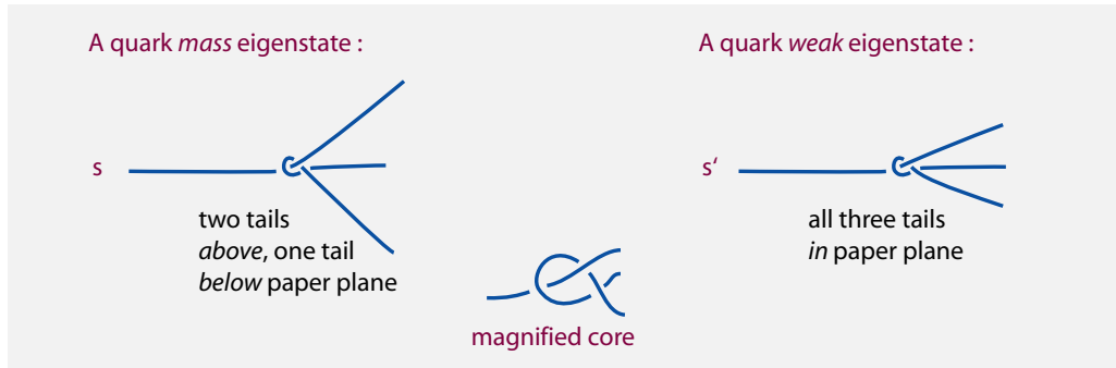
FIGURE 116 Tail shifting leads to quark mixing: mass eigenstates and weak eigenstates differ.
