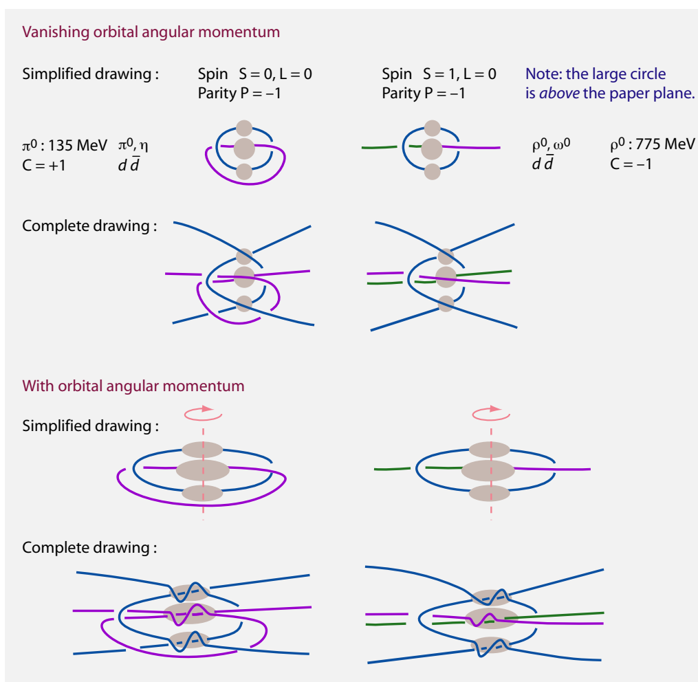
FIGURE 100 The strand model for mesons without (top) and with (bottom) orbital angular momentum.
