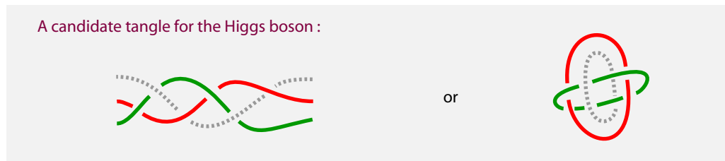
FIGURE 93 A candidate tangle for the Higgs boson in the strand model: the open version (left) and the corresponding closed version (right). For the left version, the tails approach the six coordinate axes at infinity.
