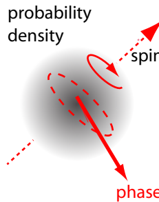
FIGURE 122 In the strand conjecture, the wave function and the probability density are due, respectively, to crossings and to crossing switches at the Planck scale. The wave function arises as time average of crossings in fluctuating tangled strands; a Hilbert space also arises. The probability density arises as time average of the crossing switches in a tangle. The tethers – connections that continue up to large spatial distances – generate spin 1/2 behaviour under rotations and fermion behaviour under particle exchange. The tangle model ensures that fermions are massive and move slower than light.
