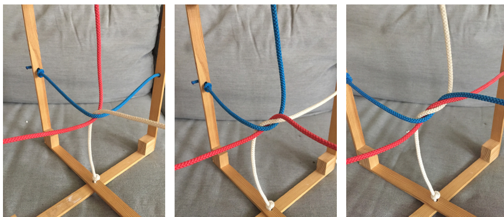
FIGURE 118 An alternative candidate assignment for the three neutrino tangles that generates large mixing between neighbouring generations and strong preference for one handedness.
