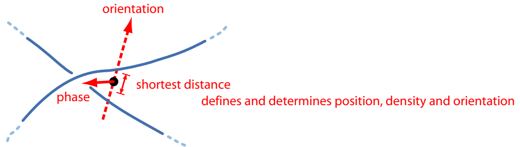
FIGURE 121 The geometry of a (skew) strand crossing suggests a relation to wave functions. In both cases, absolute phase around the orientation axis can be chosen freely. In contrast, phase differences due to rotations around that axis are always uniquely defined.
