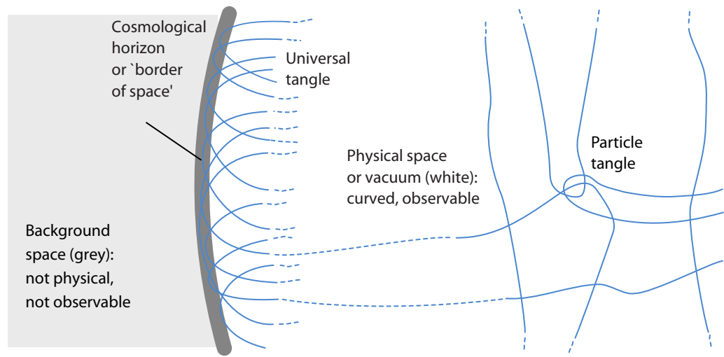
FIGURE 135 In the strand conjecture, the universe is limited by a cosmological (particle) horizon, as schematically illustrated here. Physical space (white) matches background space (grey) only inside the horizon. Physical space thus only exists inside the cosmic horizon.
