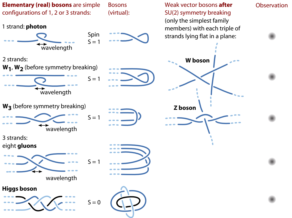
FIGURE 126 The tangle models for the elementary bosons. These tangles determine the spin values, the corresponding propagators, and ensure that the massless photons and gluons move with the speed of light. Apart from the graviton, no additional elementary boson appears to be possible. The tangle structure determines masses and the weak mixing angle.
