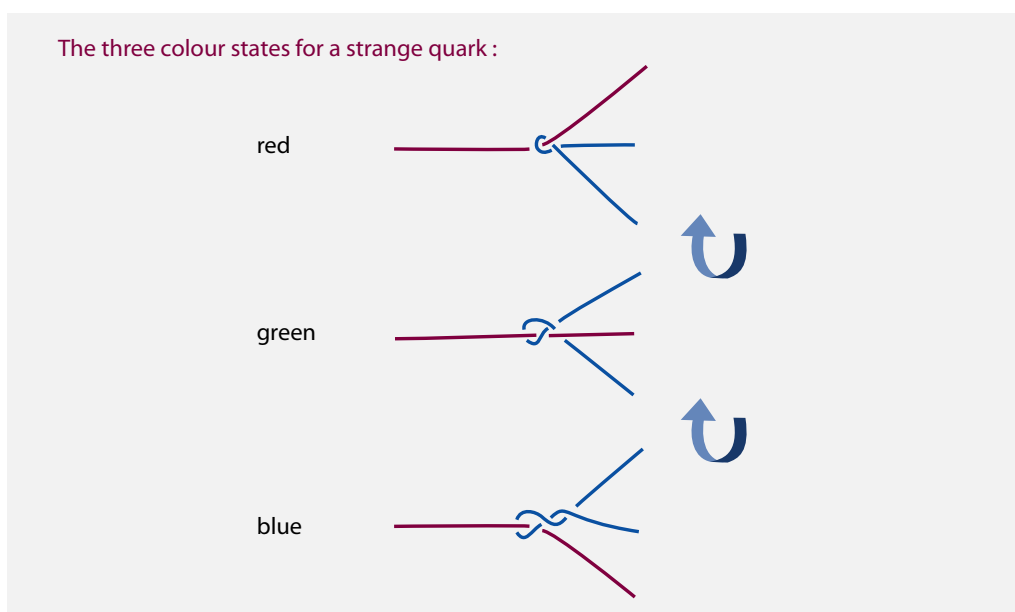
FIGURE 86 The three colour charges correspond to the three possible spatial orientations; the centre tail on the right is always above the paper plane, the other two tails on the right are below the paper plane.
