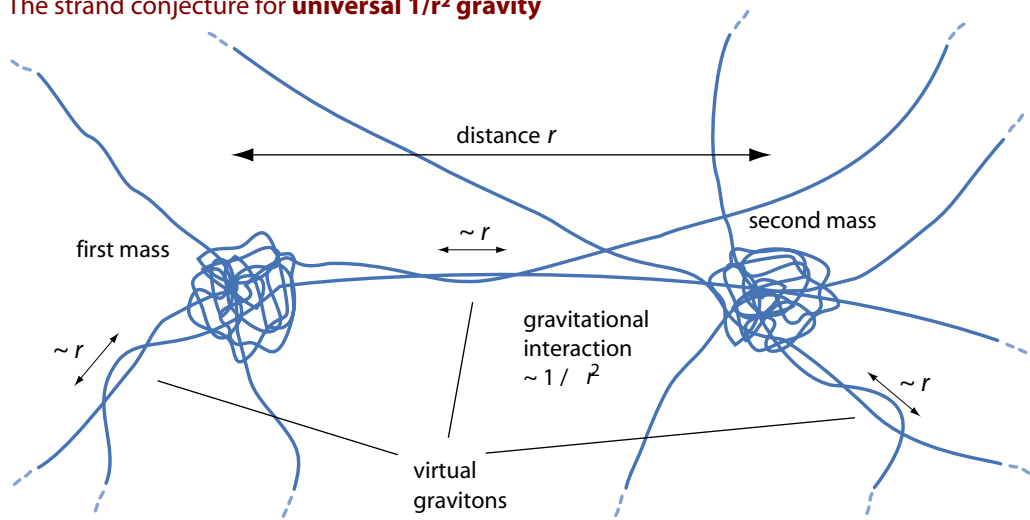
FIGURE 133 Gravitational attraction results from strands. For low speeds and negligible curvature, twisted tether pairs (virtual gravitons) from a mass lead to a 1/r^2 attraction. The average length of twisted tether pairs scales with r and yields a 1/r^3 decay of curvature. These conclusions are valid for infinite space without cosmological horizon.
