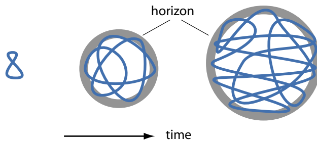
FIGURE 136 In the strand conjecture for the early universe, the universe increases in complexity over time and thereby forms a boundary: the cosmological horizon.
