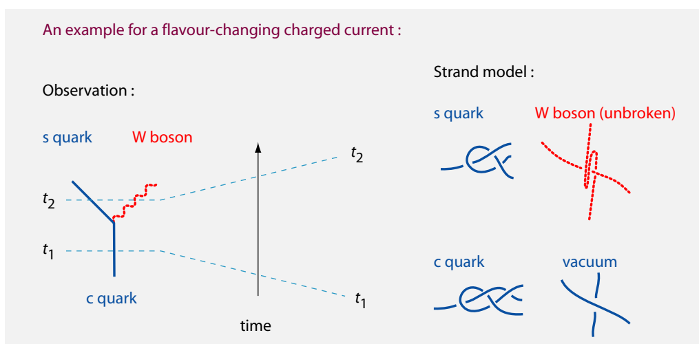
FIGURE 87 Absorption or emission of a W boson changes quark flavour.
