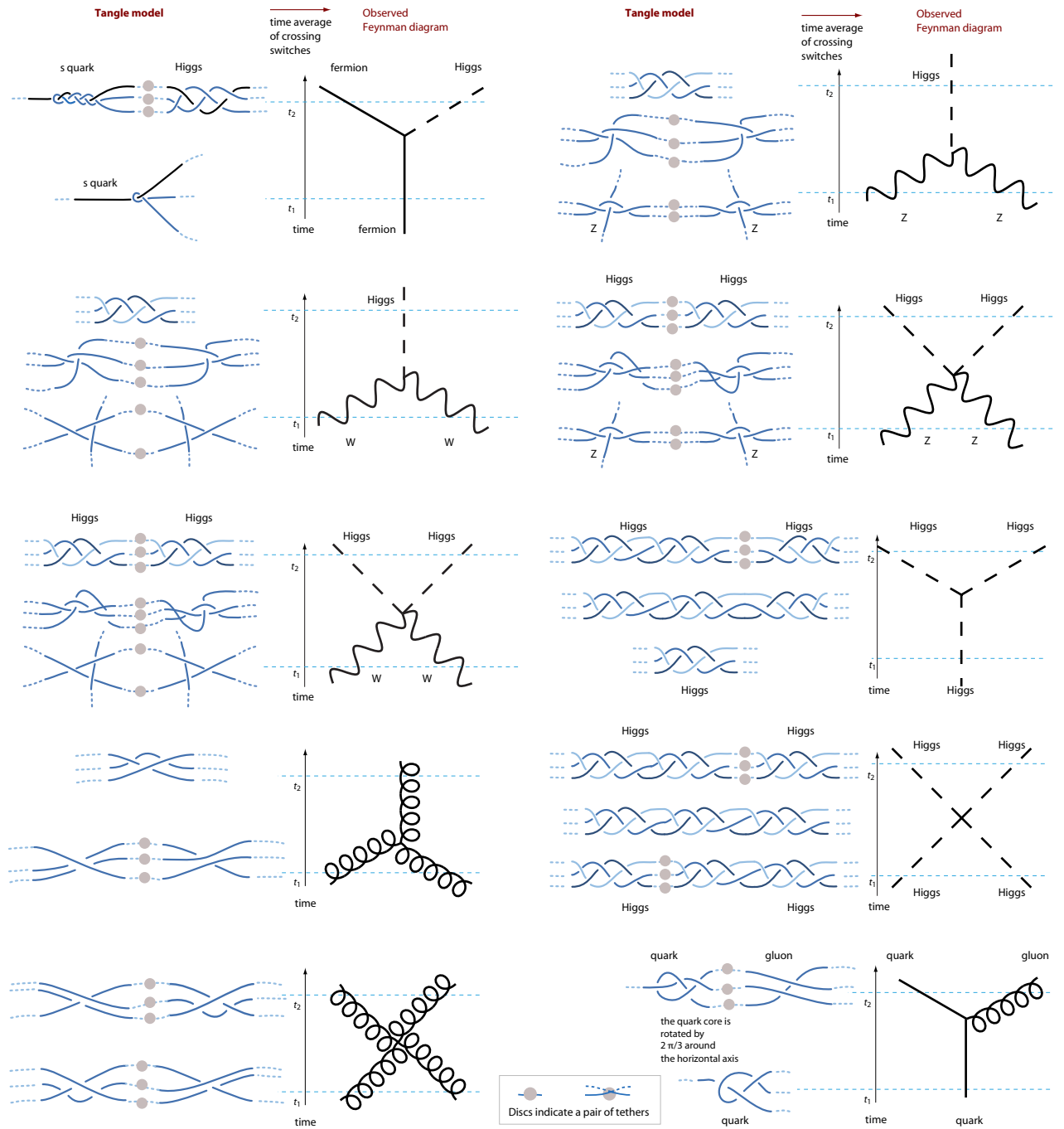
FIGURE 129 The vertices in Feynman diagrams allowed by the topology of the fermion and boson tangles (part two).
