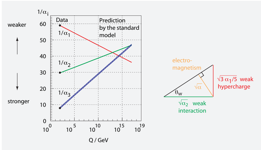
FIGURE 119 Left: How the three coupling constants (squared) change with energy, as predicted by the standard model of particle physics; the graph shows the constant \alpha_1 = \frac{5}{3}\alpha / \cos^2 \theta_W for the weak hypercharge coupling (related to the electromagnetic fine structure constant \alpha through the weak mixing angle \theta_W and a historical factor 5/3 that is useful in grand unification), the coupling constant \alpha_2 = \alpha_w = \alpha / \sin^2 \theta_W for the weak interaction, and the coupling constant \alpha_3 = \alpha_s for the strong interaction. The three black points are measurement points; at lower and slightly higher energies, data and calculation match within experimental errors. (Courtesy Wim de Boer) Right: The relation between the coupling constants \alpha for the electromagnetic U(1)_{EM} , \alpha_2 = \alpha_w for the weak SU(2) , \alpha_1 for the weak hypercharge U(1)_Y gauge groups and the weak mixing angle \theta_W .
