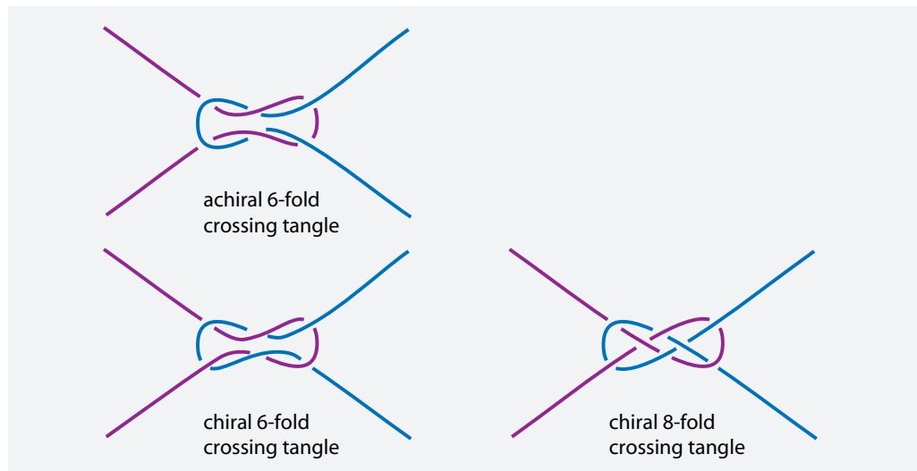
FIGURE 90 Which particle states are described by these tangles?
