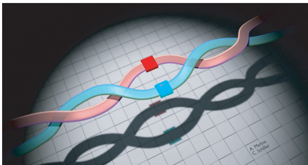
FIGURE 28 Assume that the belts cannot be observed, but the square objects can, and that they represent particles. We know from above that belted buckles behave as spin 1/2 particles. The animation shows that two such particles return to the original situation if they are switched in position twice (but not once). Such particles thus fulfil the defining property of fermions . (For the opposite case, that of bosons, a simple exchange would lead to the identical situation.) You can repeat the trick at home using paper strips. The equivalence is shown here with two belts per particle, but the trick works with any positive number of belts attached to each buckle. This animation is the essential part of the proof that spin 1/2 particles are fermions. This is called the spin-statistics theorem . (QuickTime film © Antonio Martos)
