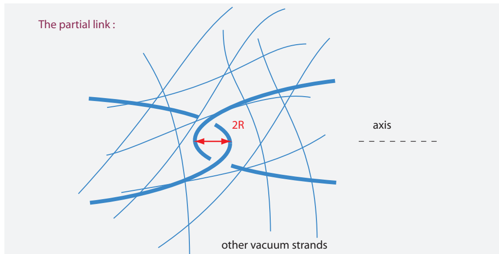
FIGURE 75 A schematic model of the fundamental defect, and thus the fundamental type of curvature: the partial link .
