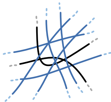
FIGURE 131 An illustration of the strand conjecture for a curved vacuum. The strand configuration is half way between that of a horizon and that of a flat vacuum. The black strands differ in their configuration from those in a flat vacuum.
