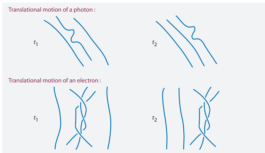
FIGURE 107 Motion of photons and electrons through strand hopping.
