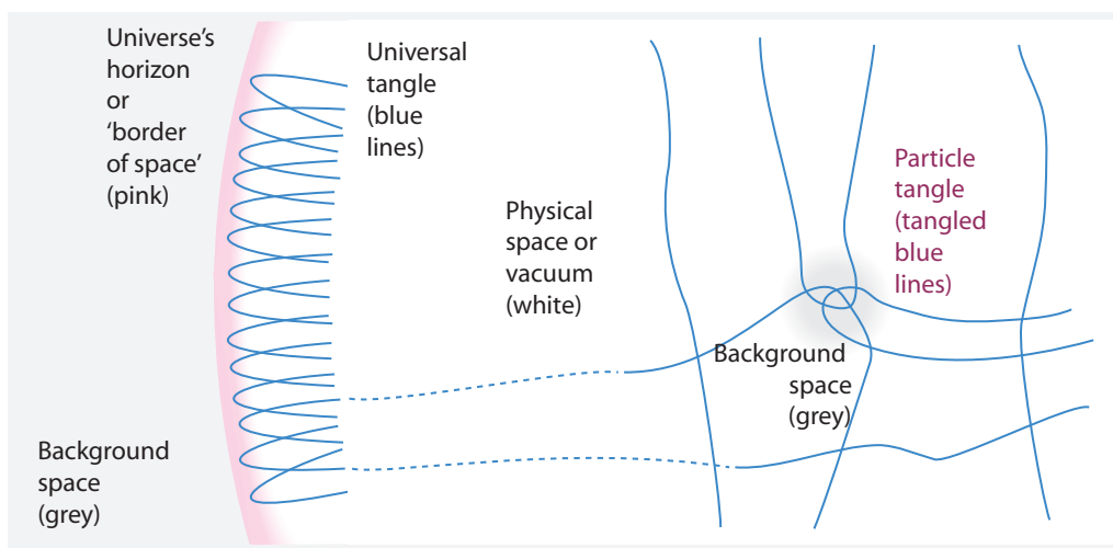
FIGURE 80 In the strand model, the universe is limited by a horizon, as schematically illustrated here. Physical space (white) matches background space (grey) only inside the horizon. Physical space thus only exists inside the cosmic horizon.
