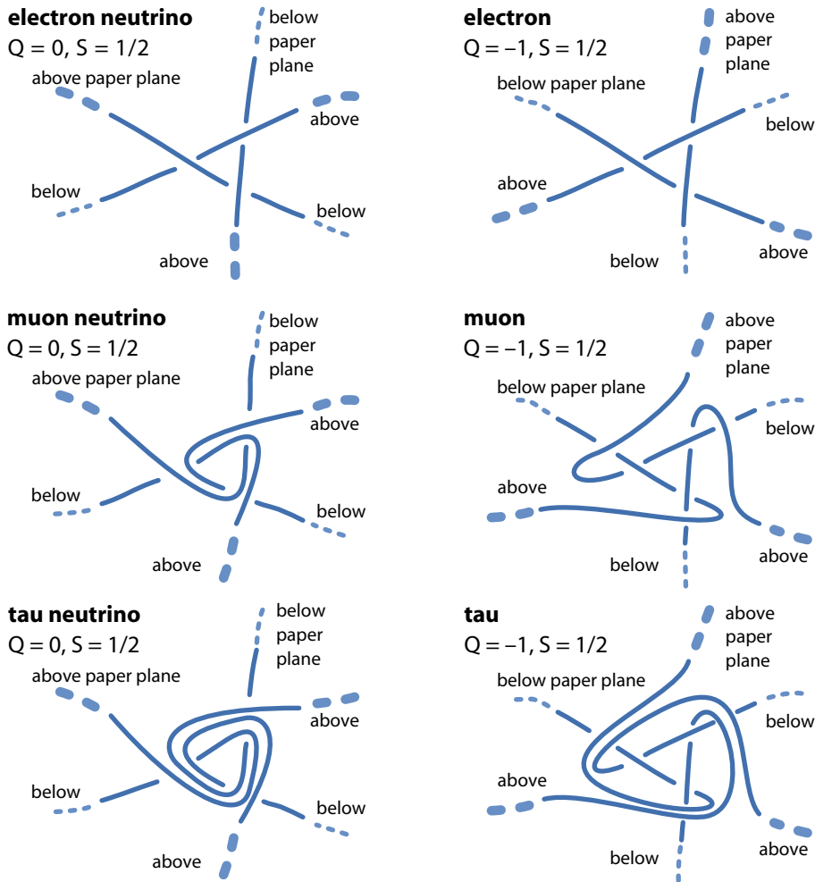
FIGURE 114 Presently proposed tangles for the leptons. Antileptons are mirror tangles. Feynman diagrams are reproduced correctly. The handedness of neutrinos is apparent. Mass sequences are as observed. The experimental mass values are also listed. At present, estimated mass values are within a few orders of magnitude.
