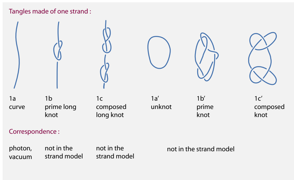
FIGURE 82 Examples for each class of tangles made of one strand.
