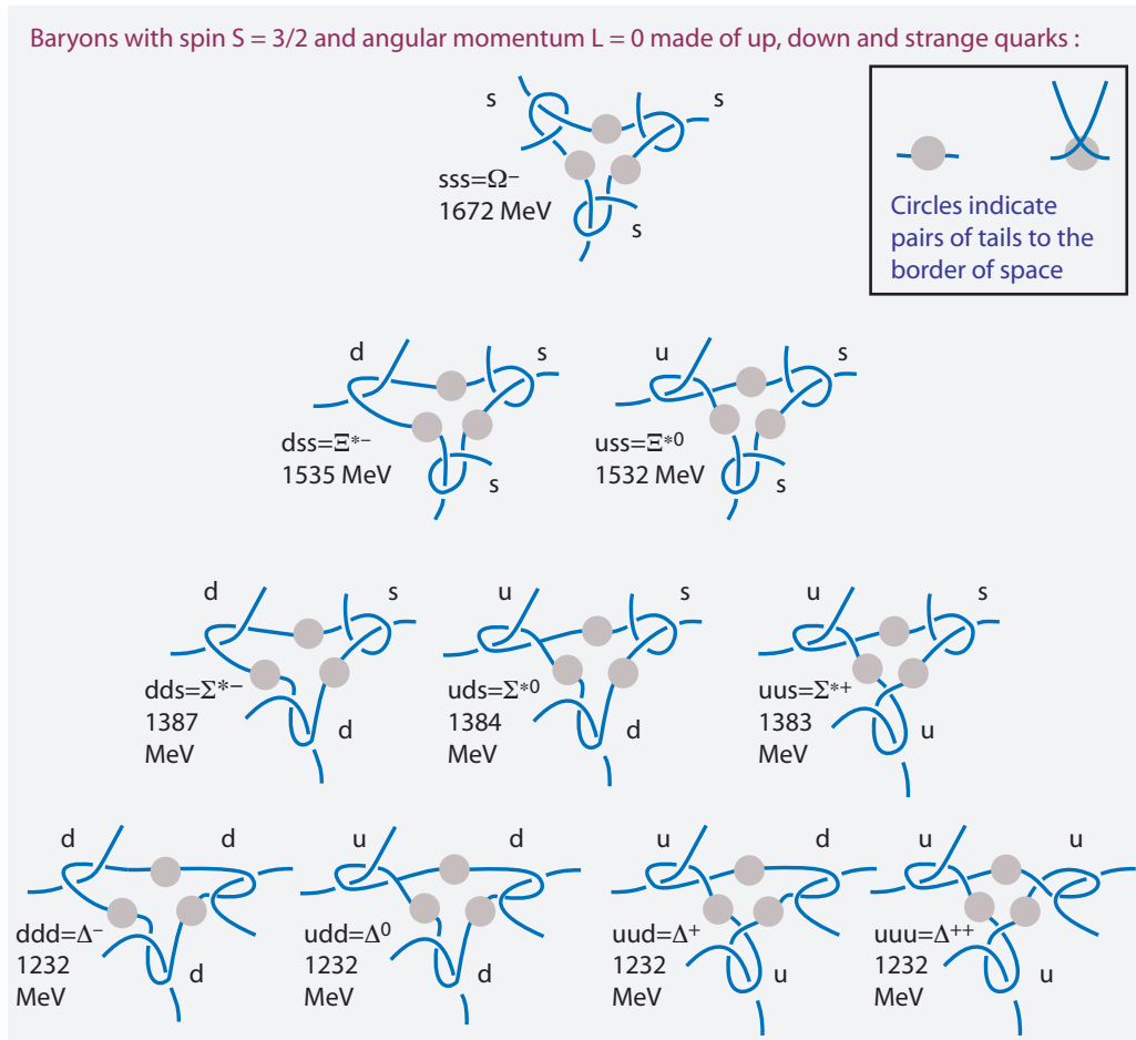
FIGURE 103 One tangle for each baryon in the lowest J=3/2 baryon decuplet (circles indicate linked tail pairs to the border of space), together with the measured mass values.
