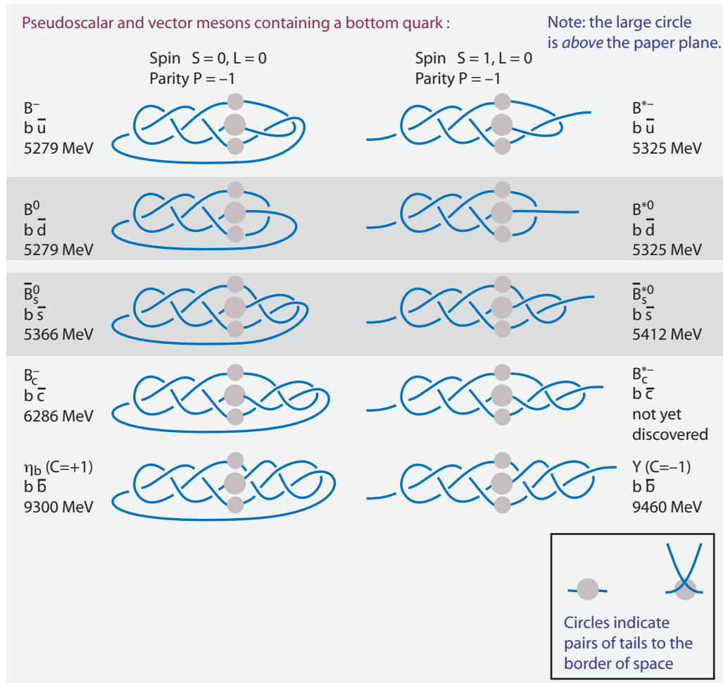
FIGURE 99 The simplest strand models for some heavy pseudoscalar and vector mesons, together with their experimental mass values. Antiparticles are not drawn; their tangles are mirrors of the particle tangles. Circles indicate crossed tail pairs to the border of space; grey boxes indicate tangles that mix with their antiparticles and which are thus predicted to show CP violation.
