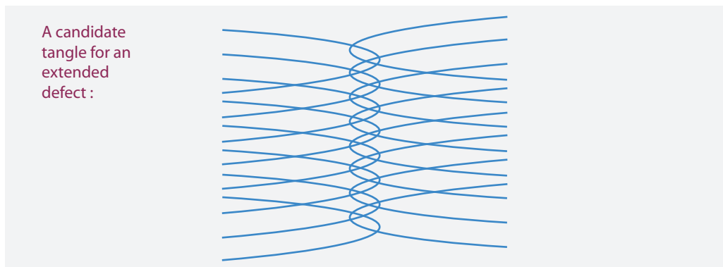
FIGURE 79 A speculative, highly schematic model for a cosmic string, a one-dimensional defect in space-time
