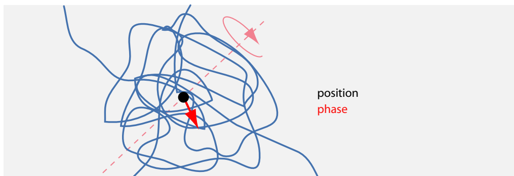
FIGURE 48 A magnified tangle core shows that the phase can also change due to core deformations ; such core deformations lead to gauge interactions .
