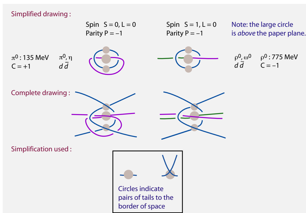
FIGURE 97 The meaning of the circles used in the tangle graphs of mesons and baryons.
