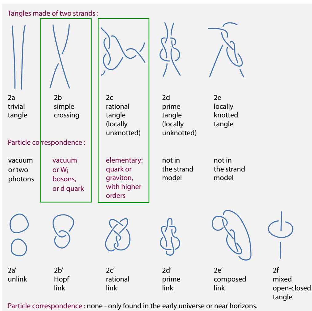
FIGURE 84 Possible tangles made of two strands.
