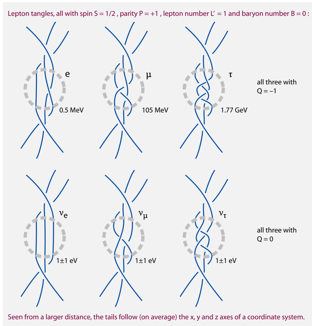
FIGURE 92 The simplest tangles of the leptons, with the experimental mass values. Antileptons are mirror tangles.
