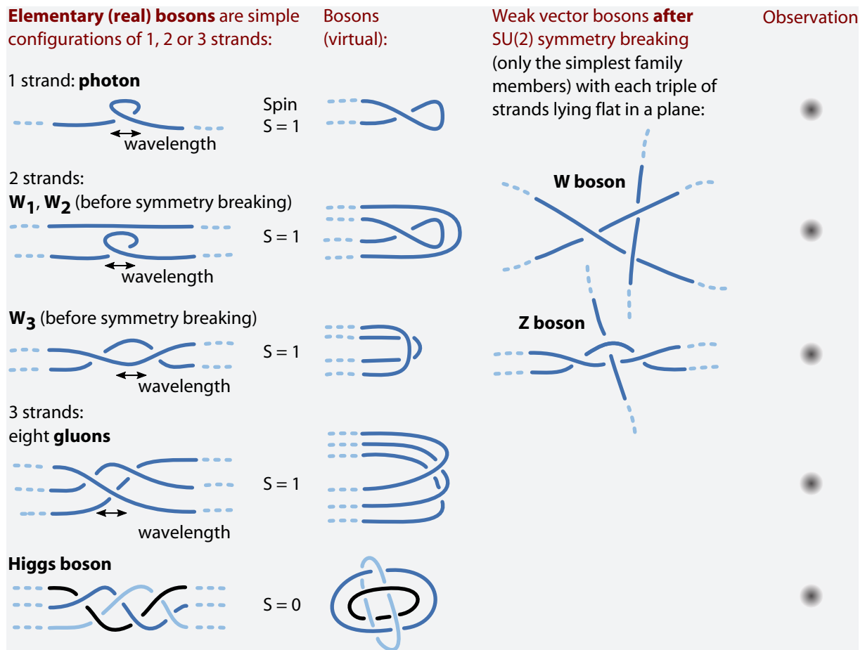
FIGURE 109 The tangle models for the elementary bosons. These tangles determine the spin values, the corresponding propagators, and ensure that the massless photons and gluons move with the speed of light. No additional elementary bosons appear to be possible.
