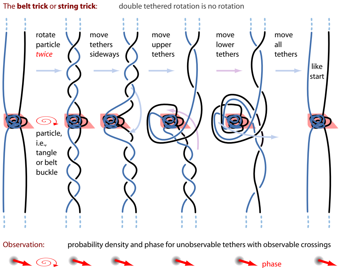
FIGURE 123 The belt trick or string trick : a rotation by 4\pi of a tethered particle, such as a belt buckle or a tangle, is equivalent to no rotation – when the tethers are allowed to fluctuate and untangle as shown. This equivalence allows the tethered particle to rotate forever. Untangling is impossible after a rotation by 2\pi only. This illustrates spin 1/2 .
