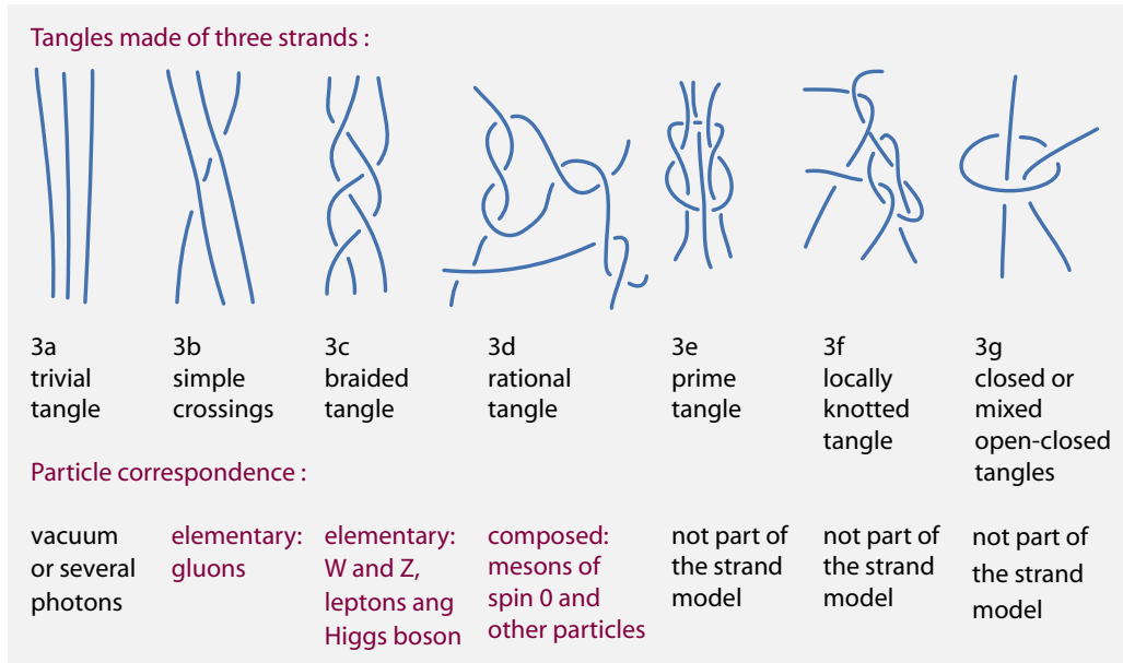
FIGURE 91 Examples for all the classes of tangles made of three strands.
