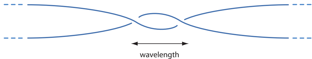
FIGURE 132 The strand conjecture for the graviton: a twisted pair of strands has spin 2, boson behaviour and vanishing mass.
