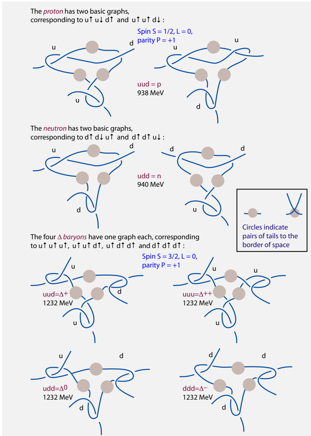
FIGURE 101 The simplest strand models for the lightest baryons made of up and down quarks (circles indicate linked tail pairs to the border of space), together with the measured mass values.
