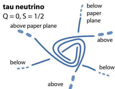
FIGURE 127 The simplest tangle models for the elementary fermions. Elementary fermions are described by rational, i.e., unknotted tangles. Their structures lead to coupling to the Higgs, as illustrated in Figure 129, produce positive mass values, and limit the number of generations to 3. Each fermion is represented by a tangle family, consisting of the simplest member and of tangles with added Higgs braids. The tangles determine the specific fermion propagators, including the values of masses and mixing angles. The tethers of the quark tangles follow the axes of a tetrahedron. The neutrino cores are simpler when seen in three dimensions: they are twisted triples of strands. The tethers of all lepton tangles approach the three coordinate axes at large distances from the core. No additional elementary fermions appear to be possible.
