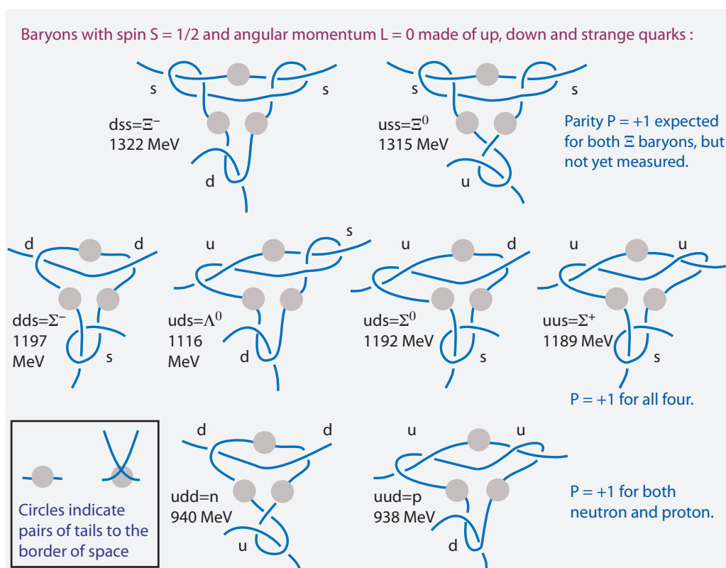
FIGURE 102 One tangle (only) for each baryon in the lowest J=L+S=1/2 baryon octet (circles indicate linked tail pairs to the border of space), together with the measured mass values.
