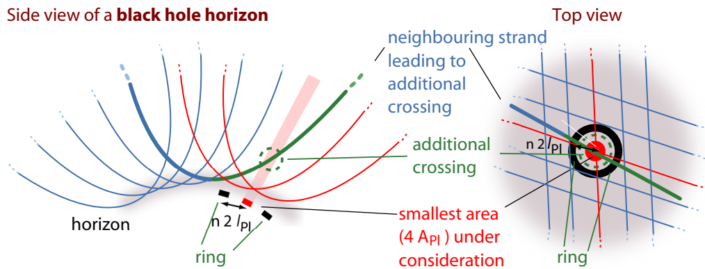
FIGURE 134 The strand conjecture for a Schwarzschild black hole: the black hole horizon is a cloudy or fuzzy surface produced by the crossing switches of the strands woven into it. Due to the additional crossings on the side of the observer, the number of micro-states per smallest area is larger than 2.
