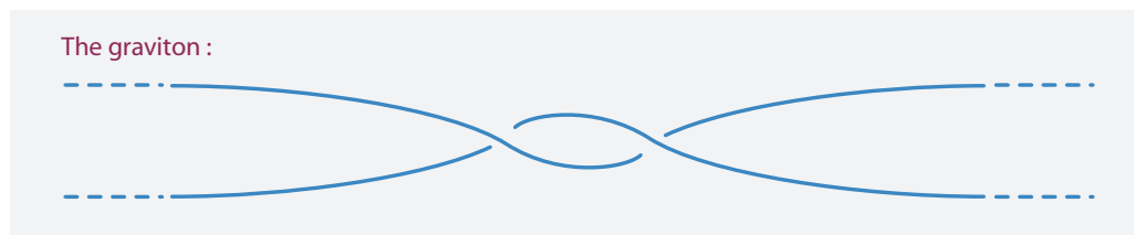
FIGURE 78 The graviton in the strand model: a twist in a pair of tethers.
