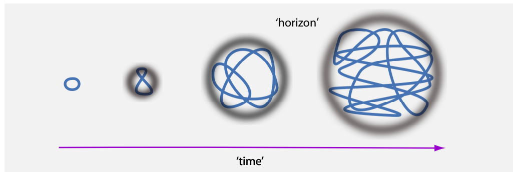
FIGURE 81 An extremely simplified view of how the universe evolved near the big bang. In this evolution, physical time, space and the surrounding horizon are in the process of getting defined.
