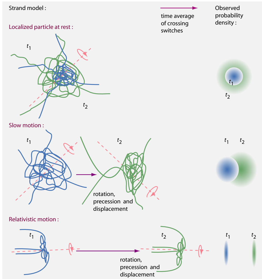
FIGURE 44 Tangles at rest, at low speed and at relativistic speed.
