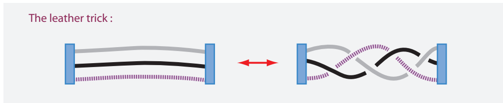
FIGURE 88 The leather trick is the deformation process that changes these two structures into each other. The leather trick limits structures made of three-stranded braids to six basic types.
