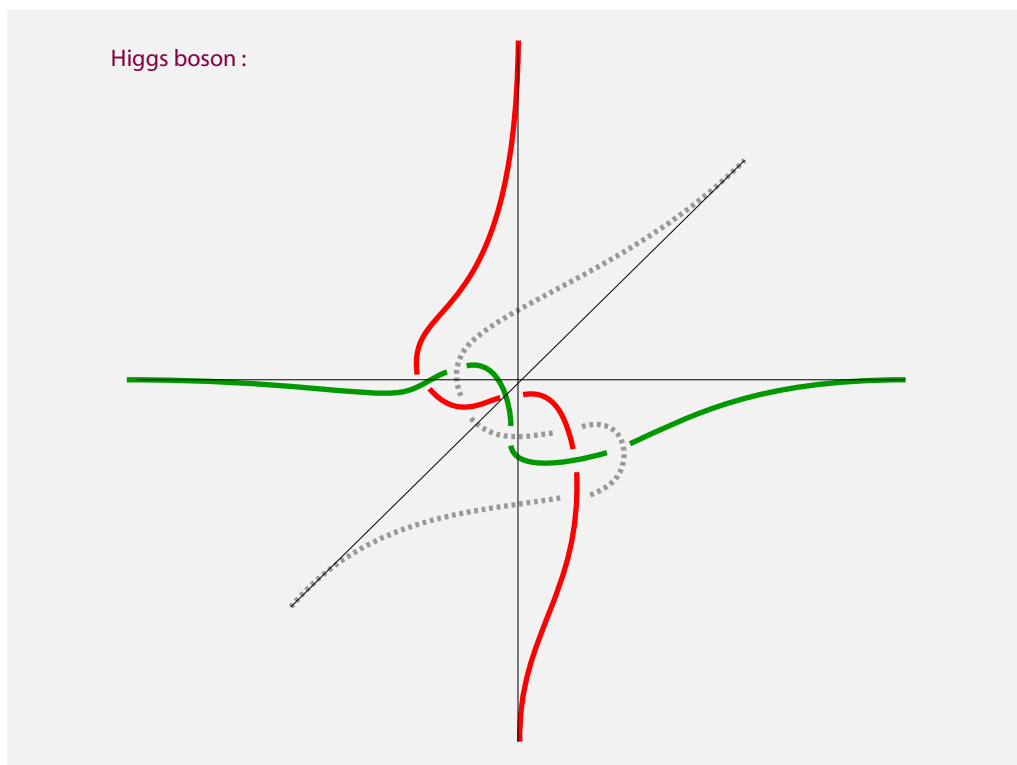
FIGURE 95 The tangle of the Higgs boson in the strand model. Spin 0 appears because the braid can be oriented in different directions, so that the time average has spherical symmetry. The tangle has 9 crossings: 3 crossings appear already in the vacuum configuration of three strands, and the additional 6 crossings (see Figure 93 ) are due to the Higgs boson.
