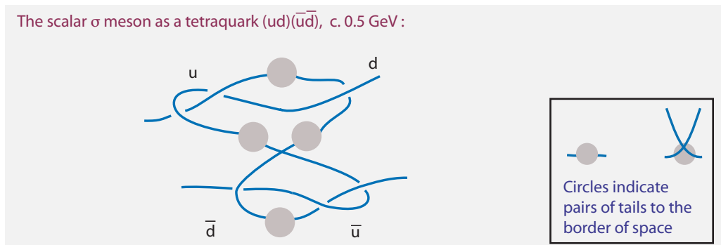
FIGURE 104 The strand model for a specific tetraquark (circles indicate linked tail pairs to the border of space).
