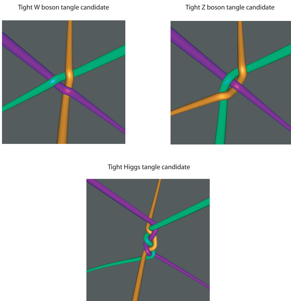
FIGURE 111 Tight tangle candidates (of 2015/2016) for the simplest tangles of the W, the Z and the Higgs bosons. In contrast to the pictures, the W and Z tails lie in a plane.
