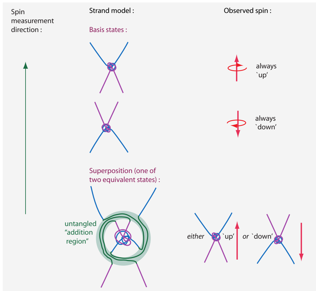
FIGURE 40 Measurement of a spin superposition: the addition region disappears either outwards or inwards.
