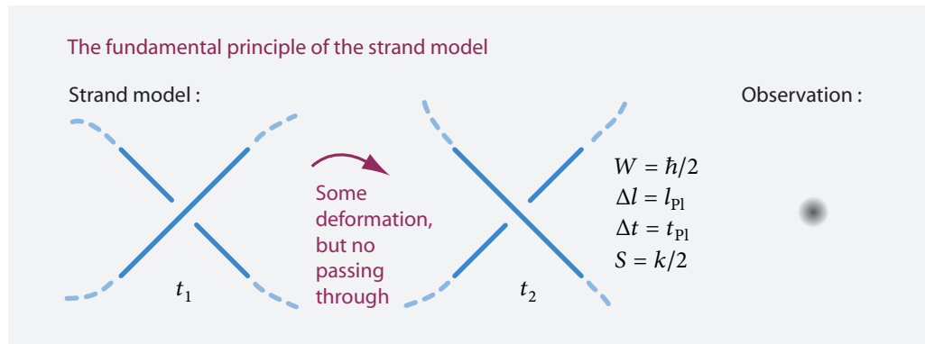
FIGURE 137 The fundamental principle of the strand model: Planck units are defined by a crossing switch in three spatial dimensions. With this principle, as shown in the previous chapters, the fundamental principle implies general relativity and the standard model of particle physics.
