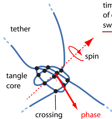
FIGURE 122 In the strand conjecture, the wave function and the probability density are due, respectively, to crossings and to crossing switches at the Planck scale. The wave function arises as time average of crossings in fluctuating tangled strands; a Hilbert space also arises. The probability density arises as time average of the crossing switches in a tangle. The tethers – connections that continue up to large spatial distances – generate spin 1/2 behaviour under rotations and fermion behaviour under particle exchange. The tangle model ensures that fermions are massive and move slower than light.
