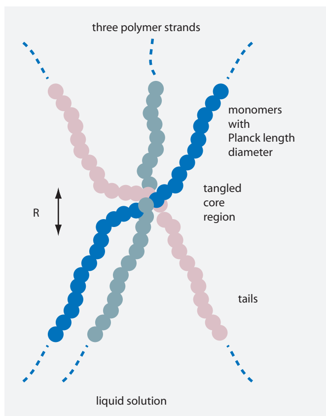
FIGURE 115 Determining lepton mass values with the help of a polymer analogy of strands. After rescaling, the probability of crossing switches around the tangle core yields an estimate for the mass of the elementary particle with that tangle.
