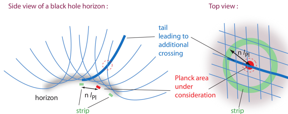
FIGURE 77 The entropy of black holes results from the number of possible crossing states above a Planck area.
