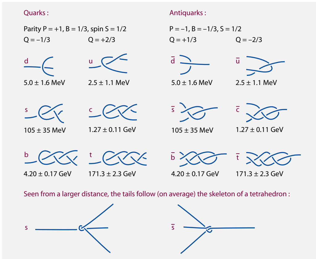
FIGURE 112 The simplest tangles assigned to the quarks and antiquarks. The experimental mass values are also given. Calculated mass values are still a topic of research.
