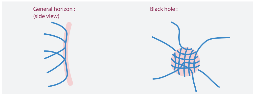
FIGURE 76 A schematic model of a general and a spherical horizon as tight weaves, as pictured by a distant observer. In the strand model there is nothing , no strands and thus no space, behind a horizon.
