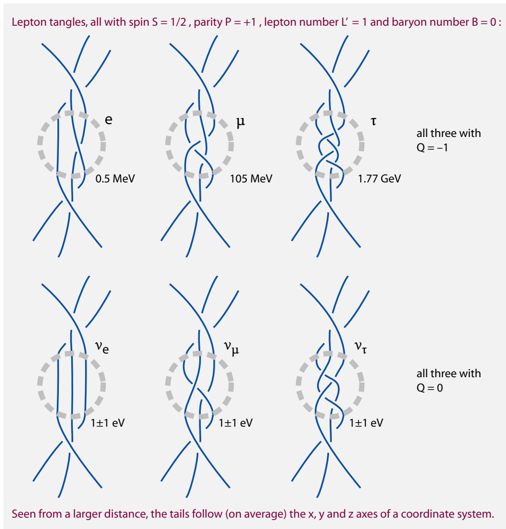
FIGURE 113 Simple – wrong – candidate tangles for the leptons. Antileptons are mirror tangles. The experimental mass values are also given. These wrong tangles yield the wrong mass sequence.
