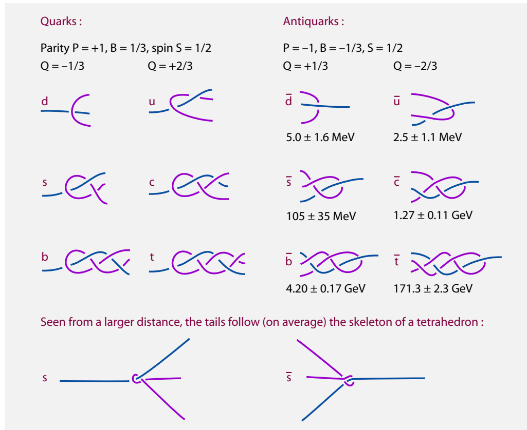
FIGURE 85 The simplest tangles assigned to the quarks and antiquarks. For reference, the experimental mass values are also given.
