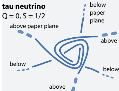
FIGURE 110 Elementary fermions are described by rational, i.e., unknotted tangles. Their structures lead to coupling to the Higgs, as illustrated in Figure 129, produce positive mass values, and limit the number of generations to 3. The tangles determine the specific fermion propagators. The tethers of the quark tangles follow the axes of a tetrahedron. The neutrino cores are simpler when seen in three dimensions: they are simply twisted triples of strands. The tethers of all lepton tangles approach the three coordinate axes at large distances from the core. No additional elementary fermions appear to be possible.
