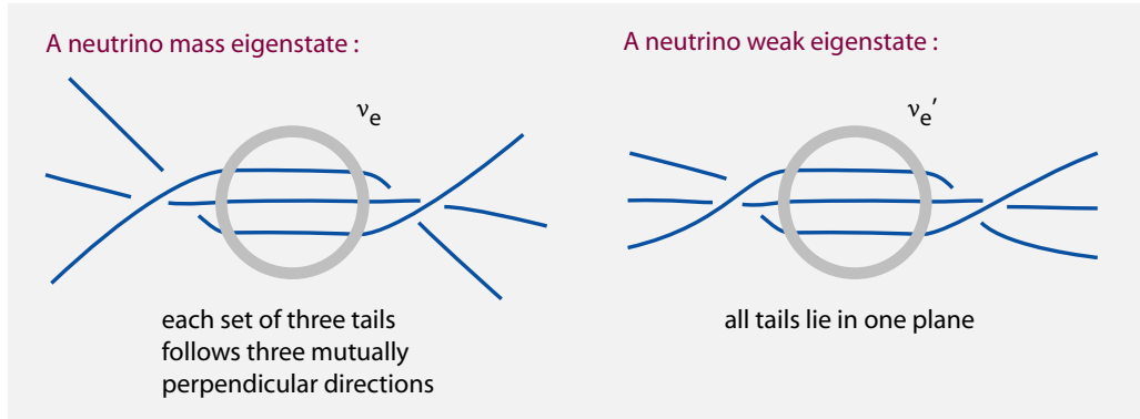
FIGURE 117 Tail shifting leads to neutrino mixing: mass eigenstates and weak eigenstates differ.
