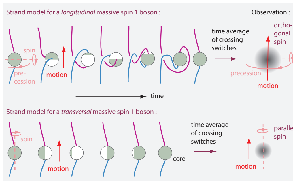
FIGURE 94 In the strand model, transverse and longitudinal W and Z bosons differ. (Note added in 2012: this statement is mistaken.)
