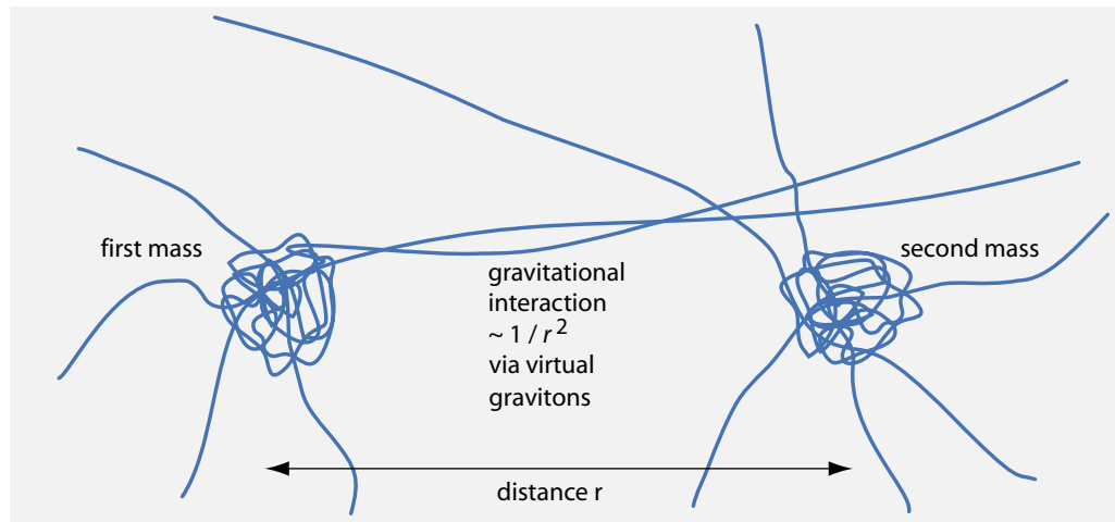
FIGURE 74 Gravitational attraction as result of twisted tail pairs – or twisted tether pairs.
