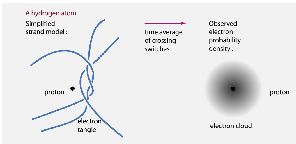
FIGURE 45 A simple, quantum-mechanical view of a hydrogen atom.
