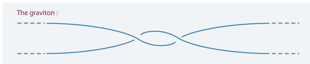
FIGURE 88 The graviton in the strand model.
