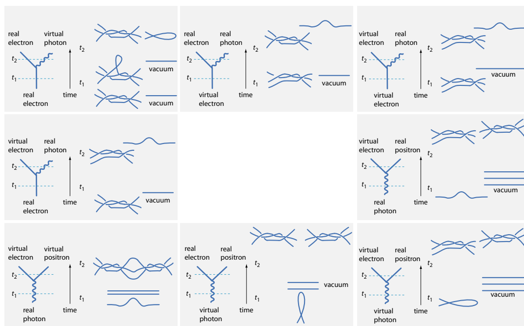
FIGURE 57 The different variations of the fundamental Feynman diagram of QED and their tangle versions.
