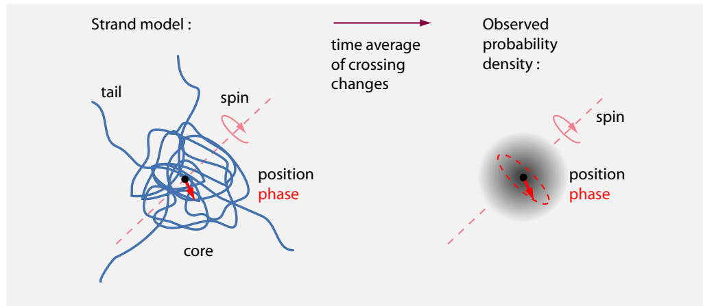
FIGURE 46 In the chapter on quantum theory, the phase was defined assuming a rigidly rotating core ; this approximation was also used in the description of particle translation.
