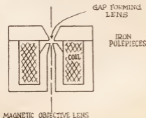
Fig. 6. The actual structure of a magnetic field lens may look like this.
