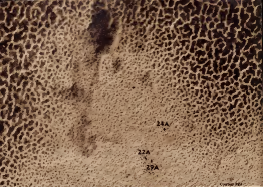
An evaporated gold film. They're slightly less than 200,000 times enlarged, and details less than 1/200th of a light wave long are visible.
