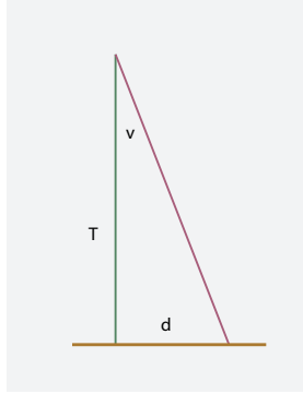
FIGURE 7 Trees and galaxies.
