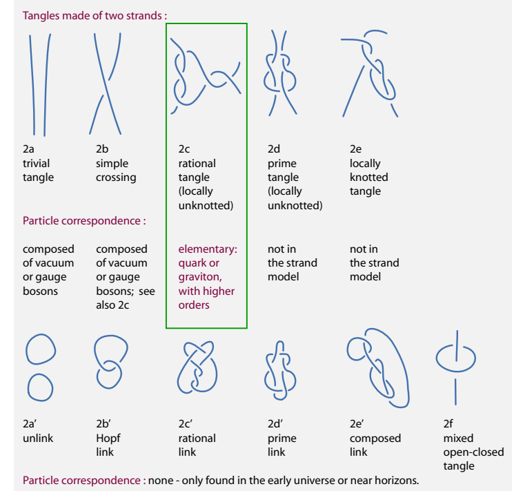
FIGURE 83 Possible tangles made of two strands.
