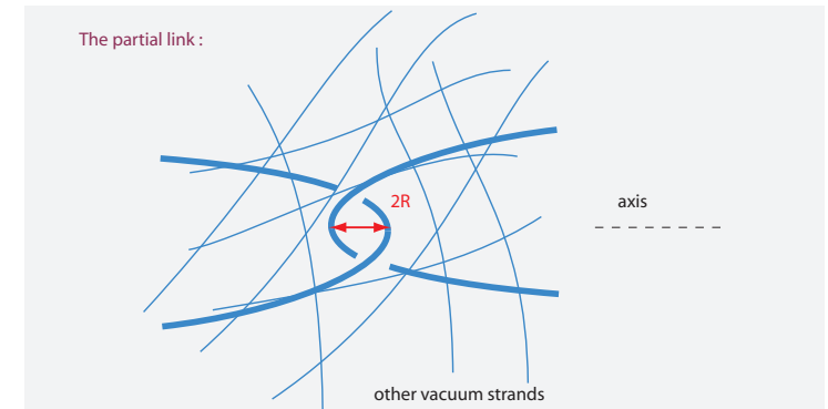
FIGURE 74 A schematic model of the fundamental defect, and thus the fundamental type of curvature: the partial link .
