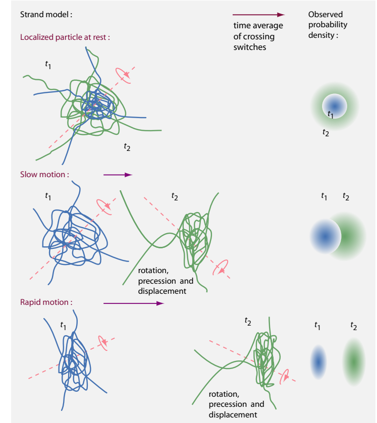
FIGURE 35 Examples of moving tangles of free particles.
