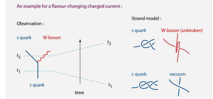
FIGURE 86 Absorption or emission of a W boson changes quark flavour.
