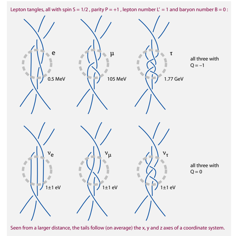
FIGURE 91 The simplest tangles of the leptons, with the experimental mass values. Antileptons are mirror tangles.
