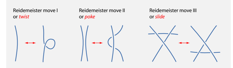
FIGURE 48 The Reidemeister moves: the three types of deformations that induce crossing switches – if the moves are properly defined in three dimensions.
