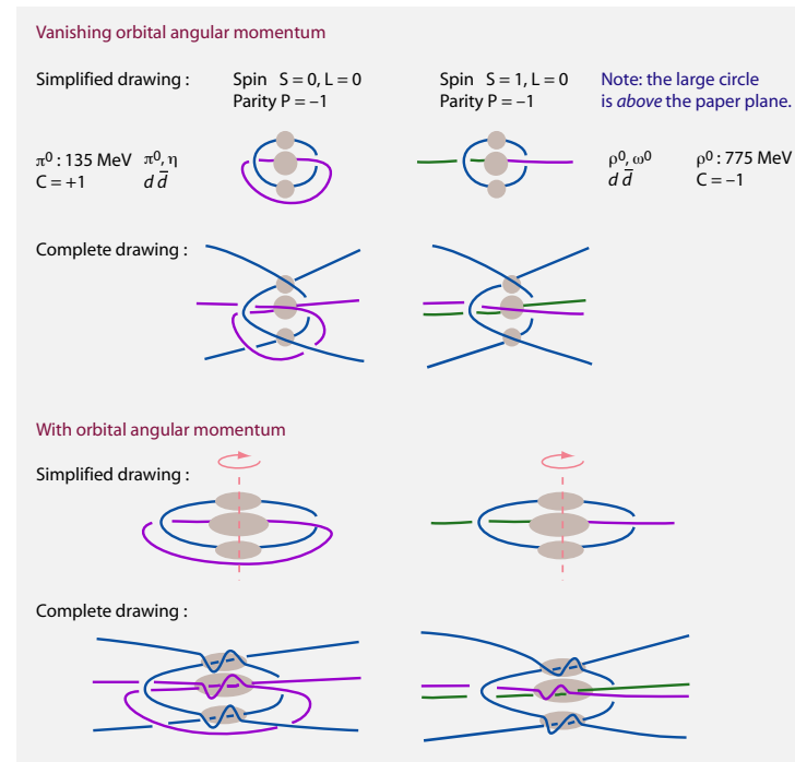
FIGURE 99 The strand model for mesons without (top) and with (bottom) orbital angular momentum.
