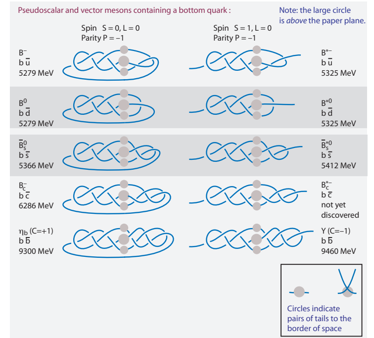
FIGURE 98 The simplest strand models for some heavy pseudoscalar and vector mesons, together with their experimental mass values. Antiparticles are not drawn; their tangles are mirrors of the particle tangles. Circles indicate crossed tail pairs to the border of space; grey boxes indicate tangles that mix with their antiparticles and which are thus predicted to show CP violation.
