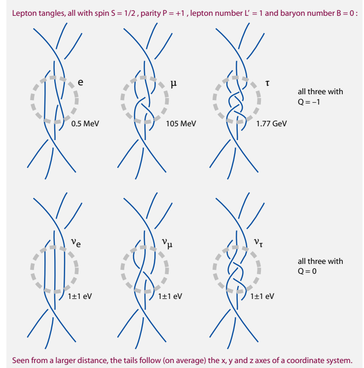
FIGURE 110 Simple candidate tangles for the leptons. Antileptons are mirror tangles. The experimental mass values are also given.
