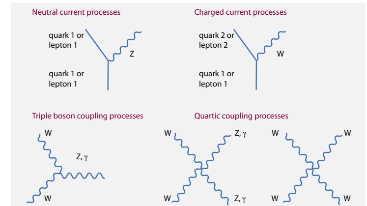
FIGURE 65 The fundamental Feynman diagrams of the weak interaction that do not involve the Higgs boson.
