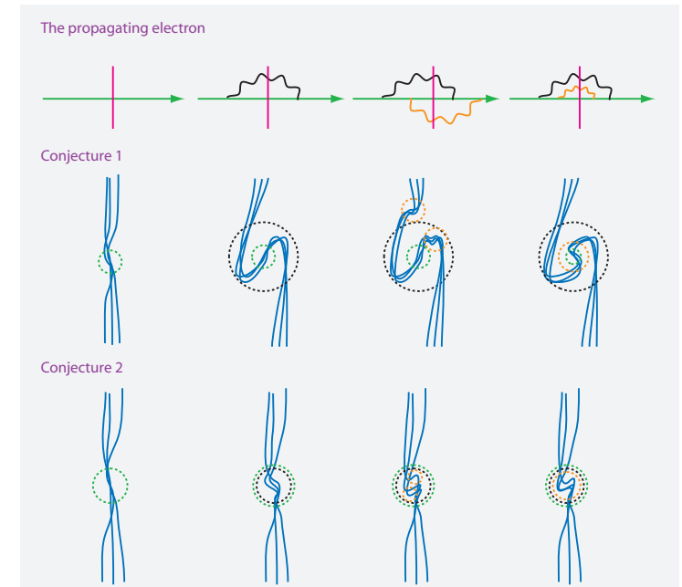
FIGURE 59 Two conjectured correspondences between the Feynman diagrams of quantum electrodynamics and the strand model for a propagating free electron. The lower strand model configurations are shown for a single instant – marked in magenta – of the electron propagator drawn above them. (For simplicity, the external field is not drawn.) In the first conjecture, the loops of the belt trick are conjectured to correspond to the virtual photons in the propagator and to be responsible for the anomalous magnetic moment. In the second conjecture, the deformations of the core correspond to the virtual photons.
