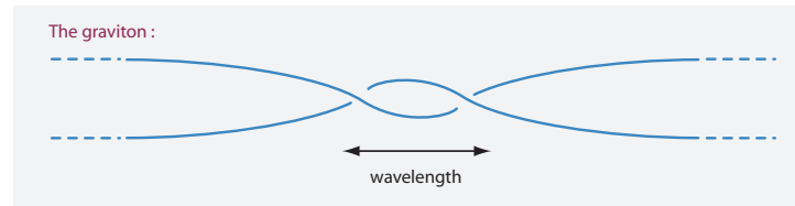
FIGURE 77 The graviton in the strand model.
