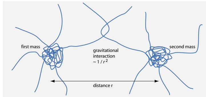
FIGURE 73 Gravitational attraction as result of strands.
