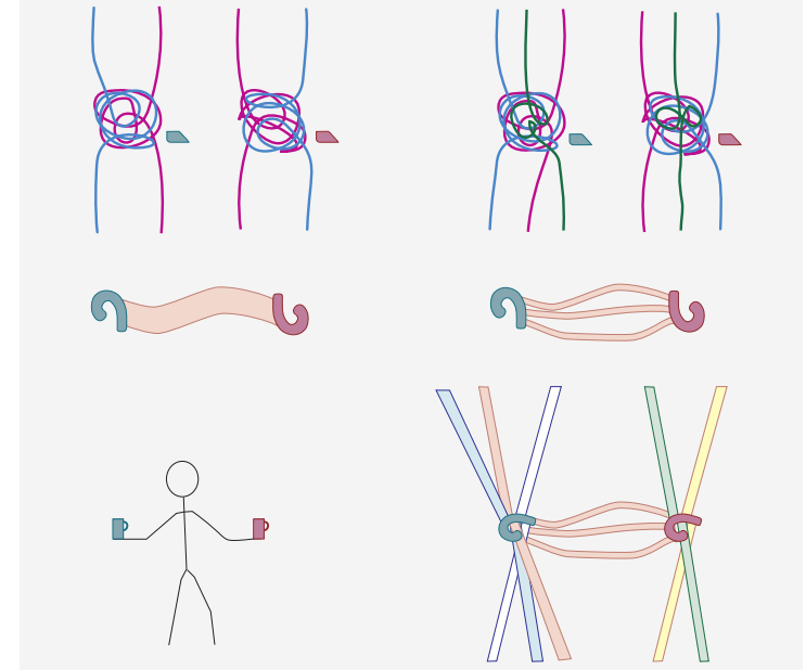
FIGURE 27 When two spin 1/2 tangles each made of several strands or bands, are exchanged twice , it is possible to rearrange their tails to yield the original situation. This is not possible when the tangles are only exchanged once . Spin 1/2 tangles are thus fermions. The figure presents common systems that show this behaviour.
