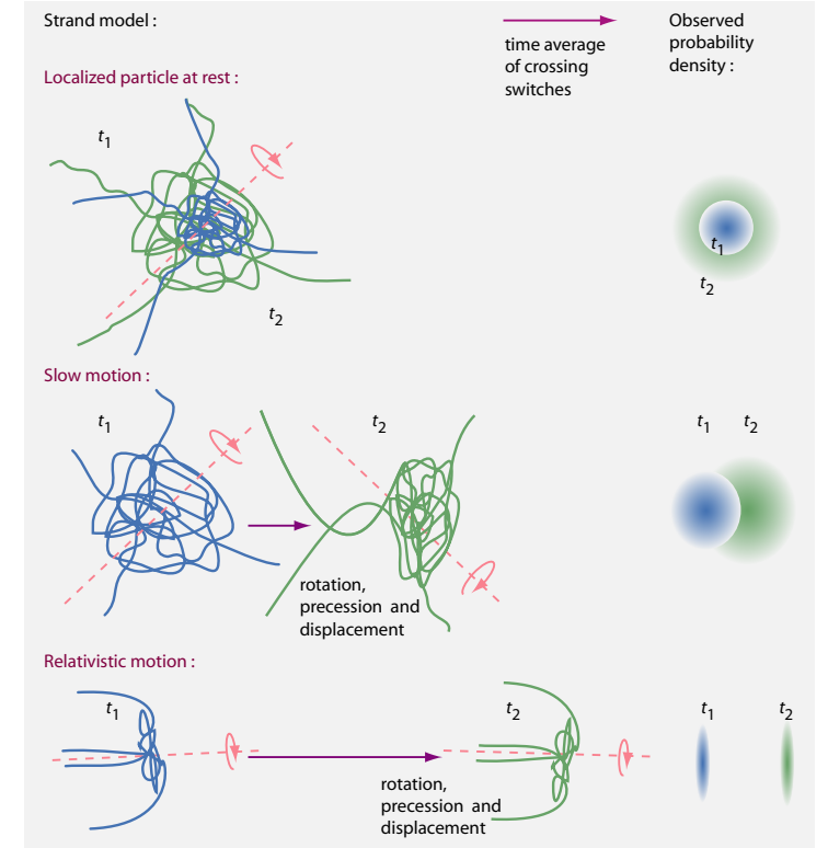
FIGURE 43 Tangles at rest, at low speed and at relativistic speed.
