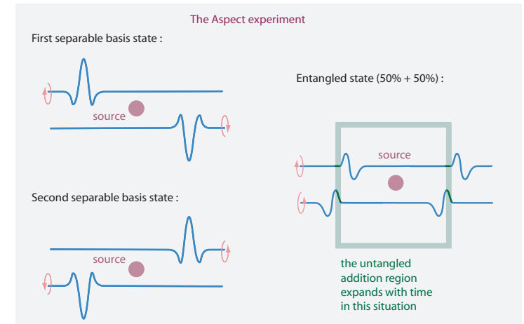
FIGURE 42 The basis states and an entangled state of two distant photons travelling in opposite directions, with total spin 0.
