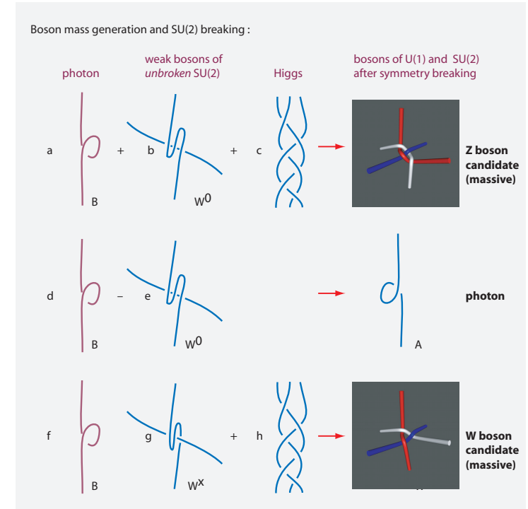
FIGURE 63 Poke-inducing strand motions (left) become massive weak vector tangles (right) through symmetry breaking and tail braiding. Tail braiding is related to the Higgs boson, whose tangle model will be clarified later on.
