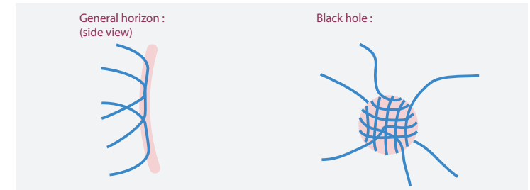
FIGURE 75 A schematic model of a general and a spherical horizon as tight weaves, as pictured by a distant observer. In the strand model there is nothing , no strands and thus no space, behind a horizon.
