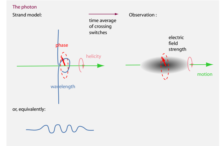
FIGURE 50 The photon in the strand model.
