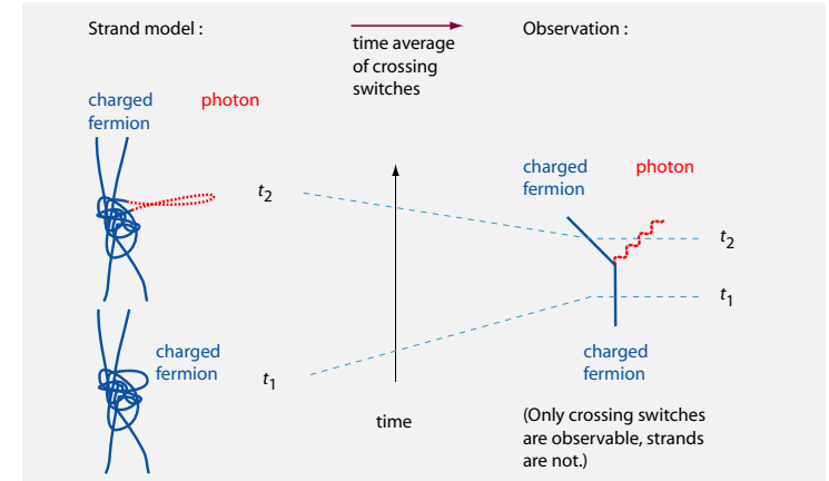
FIGURE 56 The fundamental Feynman diagram of QED and its tangle version.
