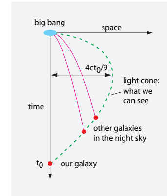
FIGURE 8 The speed and distance of remote galaxies.
