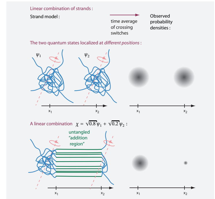
FIGURE 34 A linear combination of strands, in this case for two states representing a particle at two different position in space, visualizing the linear combination of wave functions.
