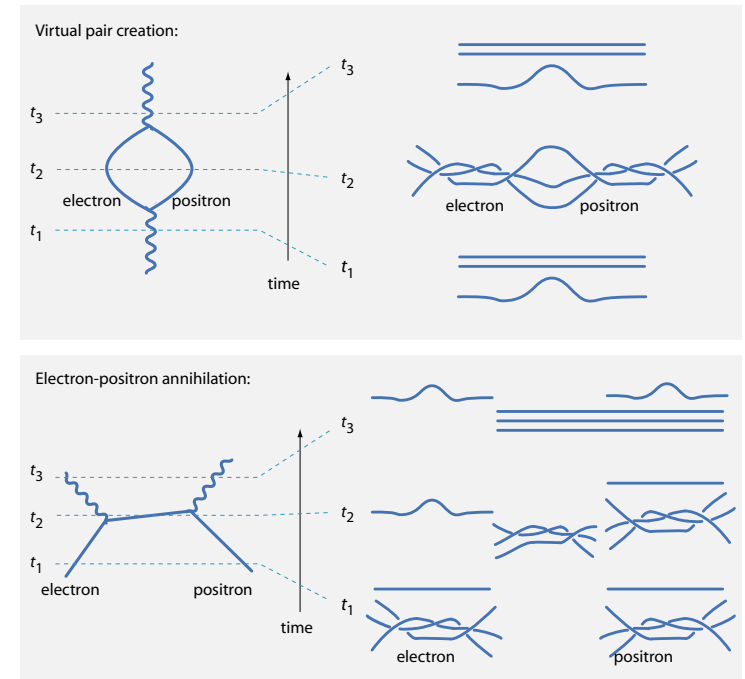
FIGURE 58 Some Feynman diagrams of QED with their tangle versions.
