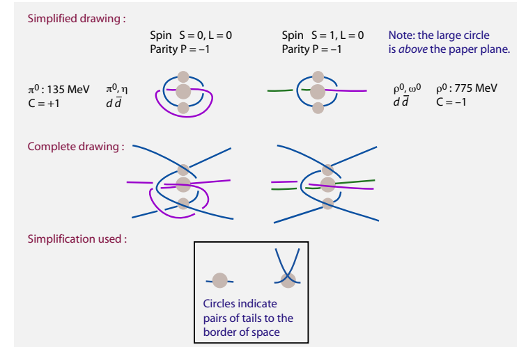
FIGURE 96 The meaning of the circles used in the tangle graphs of mesons and baryons.
