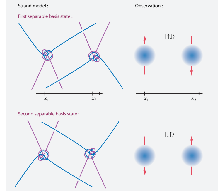
FIGURE 40 Two examples of two distant particles with spin in separable states: observation and strand model.
