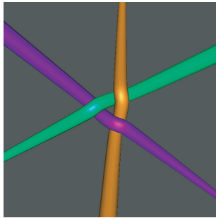
Tight W boson tangle candidate
