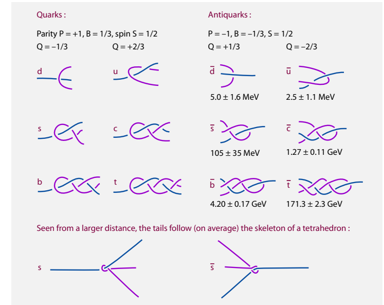
FIGURE 84 The simplest tangles assigned to the quarks and antiquarks. For reference, the experimental mass values are also given.
