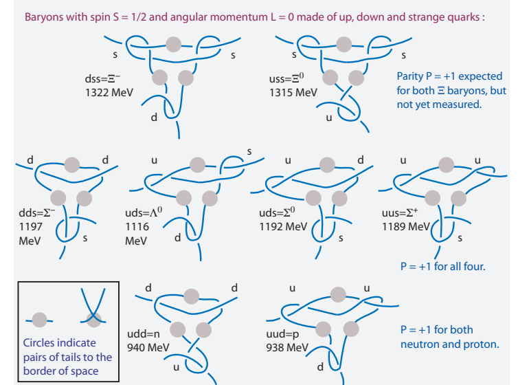
FIGURE 101 One tangle (only) for each baryon in the lowest J=L+S=1/2 baryon octet (circles indicate linked tail pairs to the border of space), together with the measured mass values.
