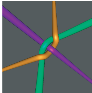
Tight Z boson tangle candidate
