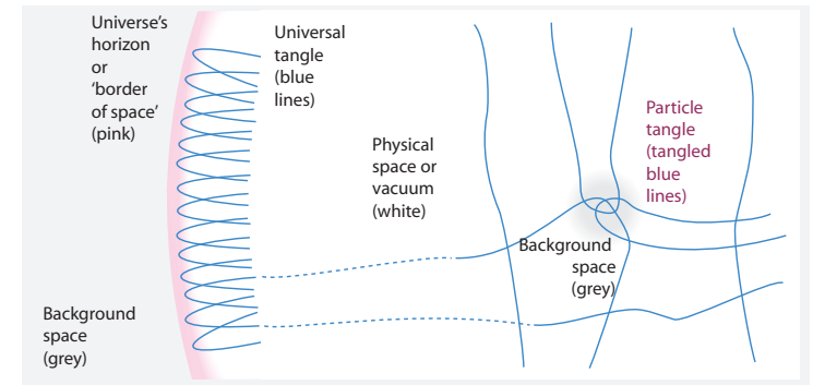
FIGURE 79 In the strand model, the universe is limited by a horizon, as schematically illustrated here. Physical space (white) matches background space (grey) only inside the horizon. Physical space thus only exists inside the cosmic horizon.
