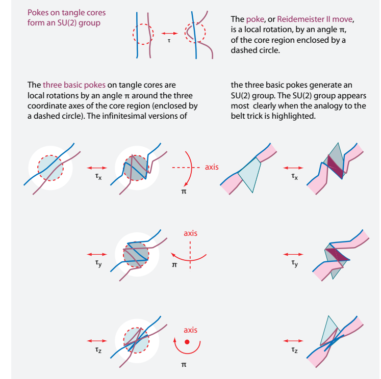
FIGURE 61 How the set of all pokes – the set of all deformations induced on tangle cores by the weak interaction – forms an SU(2) gauge group: the three pokes lead to the belt trick, illustrated here with a pointed buckle and two belts. For clarity, deformations of two strands are shown, instead of the deformation of a single strand.
