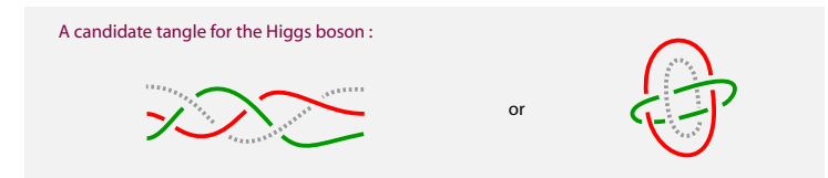
FIGURE 92 A candidate tangle for the Higgs boson in the strand model: the open version (left) and the corresponding closed version (right). For the left version, the tails approach the six coordinate axes at infinity.
