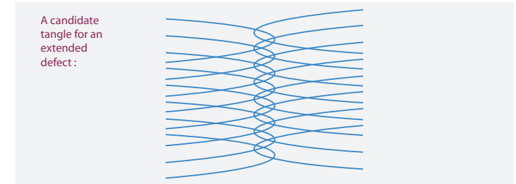
FIGURE 78 A speculative, highly schematic model for a cosmic string, a one-dimensional defect in space-time
