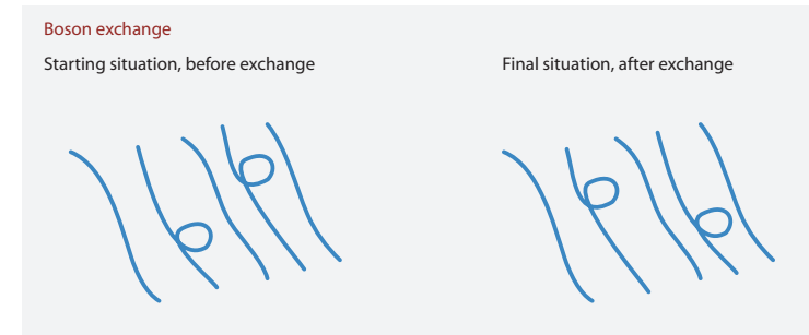
FIGURE 30 In the strand model, unknotted boson tangles can switch states without generating crossings, and thus without changing the sign of the phase.
