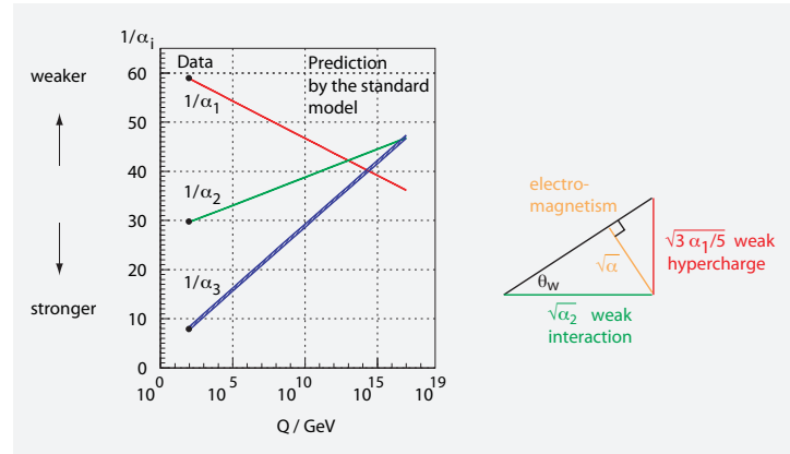
FIGURE 115 Left: How the three coupling constants (squared) change with energy, as predicted by the standard model of particle physics; the graph shows the constant \alpha_1 = \frac{5}{3}\alpha/\cos^2\theta_W for the weak hypercharge coupling (related to the electromagnetic fine structure constant \alpha through the weak mixing angle \theta_W and a historical factor 5/3 that is useful in grand unification), the coupling constant \alpha_2 = \alpha_w = \alpha/\sin^2\theta_W for the weak interaction, and the coupling constant \alpha_3 = \alpha_s for the strong interaction. The three black points are measurement points; at lower and slightly higher energies, data and calculation match within experimental errors. (Courtesy Wim de Boer) Right: The relation between the coupling constants \alpha for the electromagnetic U(1)_{EM} , \alpha_2 = \alpha_w for the weak SU(2) , \alpha_1 for the weak hypercharge U(1)_Y gauge groups and the weak mixing angle \theta_W .
