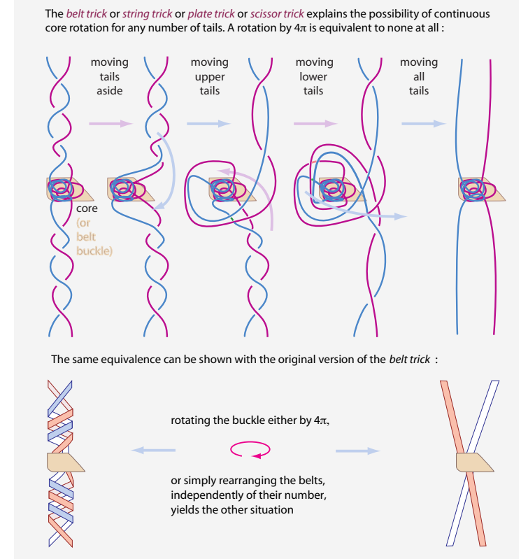
FIGURE 19 The belt trick – or string trick or plate trick or scissor trick – shows that a rotation by 4\pi of a central object with three or more tails (or with one or more ribbons) attached to spatial infinity is equivalent to no rotation at all. This equivalence allows a suspended object, such as a belt buckle or a tangle core, to rotate for ever. The belt trick thus shows that tangle cores made from two or more strands behave as spin 1/2 particles.
