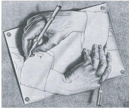
FIGURE 2 'Tekenend' by Maurits Escher, 1948 – a metaphor for the way in which 'particles' and 'space-time' are defined: each with the help of the other (© M.C. Escher Heirs).
