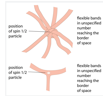
FIGURE 9 Possible models for a spin 1/2 particle.
