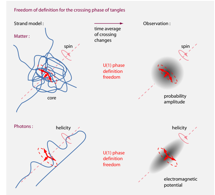
FIGURE 54 The freedom in definition of the phase of crossings leads to the gauge invariance of electrodynamics. Three exemplary choices of phase are shown.
