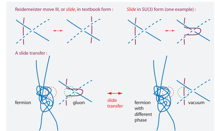
FIGURE 67 A gluon changes the phase of a tangle: slide transfer is the basis of the strong interaction in the strand model. During the interaction, no strand is cut or reglued; the transfer occurs purely through the excluded volume that results from the impenetrability of strands.
