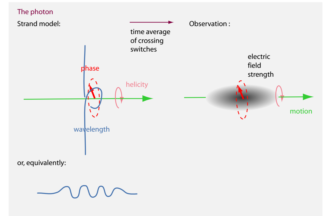
FIGURE 50 The photon in the strand model.
