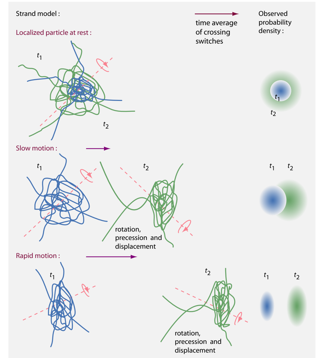
FIGURE 35 Examples of moving tangles of free particles.
