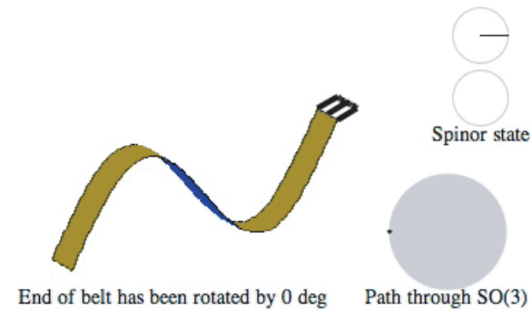
FIGURE 20 The belt trick: a double rotation of the belt buckle is equivalent to no rotation; the animation shows one way in which the belt trick can be performed. Not shown: the belt trick is also possible with any number of belts attached to the buckle. (QuickTime film © Greg Egan)
