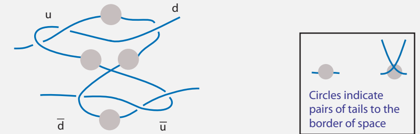
FIGURE 103 The strand model for a specific tetraquark (circles indicate linked tail pairs to the border of space).
