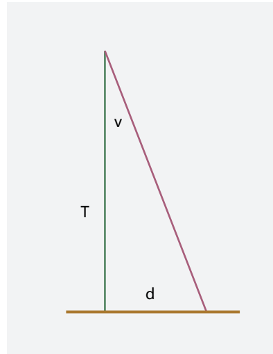
FIGURE 7 Trees and galaxies.
