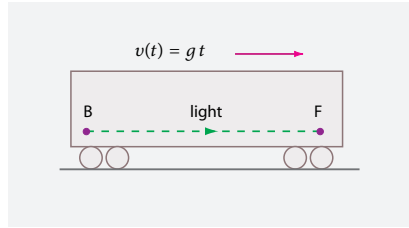
FIGURE 62 Inside an accelerating train or bus.
