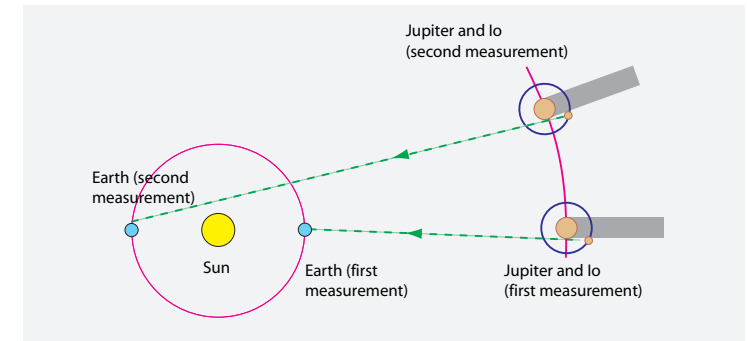
FIGURE 3 Rømer's method of measuring the speed of light.
