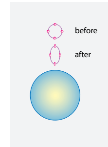
FIGURE 84 Tidal effects measure the curvature of space-time.
