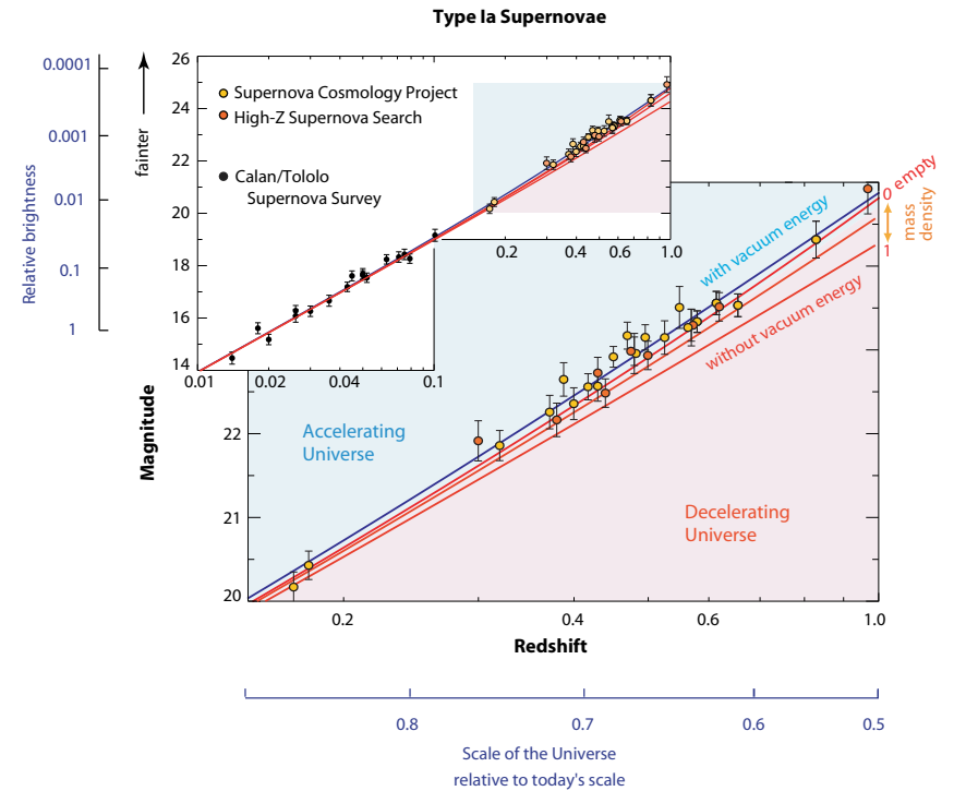
FIGURE 99 The relation between star distance and star velocity (courtesy Saul Perlmutter and the Supernova Cosmology Project).
