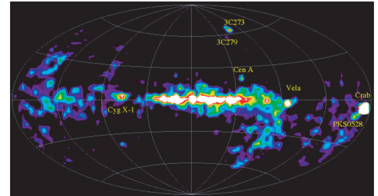
FIGURE 87 A false colour image of the X-ray sources observed in the night sky, for energies between 1 and 30 MeV (courtesy NASA).
