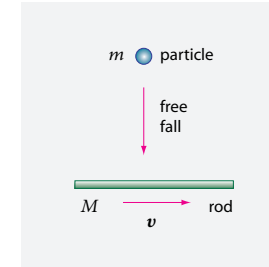
FIGURE 75 The reality of gravitomagnetism.
