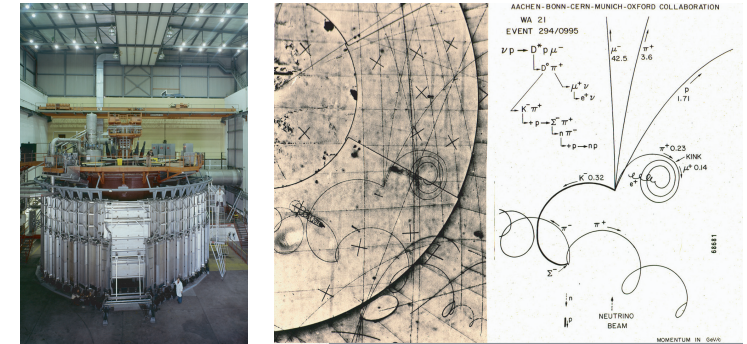
FIGURE 44 The 'Big European Bubble Chamber' and an example of tracks of relativistic particles it produced, with the momentum values deduced from the photograph (© CERN).
