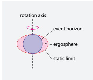
FIGURE 119 The ergosphere of a rotating black hole.
