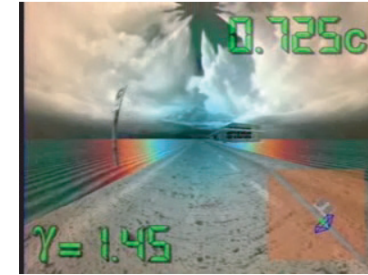
FIGURE 52 The animation shows an observer accelerating down the road in a desert, until he reaches relativistic speeds. The inset shows the position along the road. Note how things seem to recede, despite the advancing motion. (QuickTime film © Anthony Searle and Australian National University, from www.anu.edu.au/Physics/Savage/TEE .)
