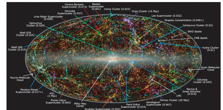
FIGURE 88 A false colour image, composed from infrared data, showing the large-scale structure of the universe around us; the colour of each galaxy represents its distance and the numbers in parentheses specify the red-shift; an infrared image of the Milky Way is superposed (courtesy Thomas Jarret/IPAC/Caltech).
