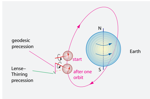
FIGURE 71 The geodesic effect.
