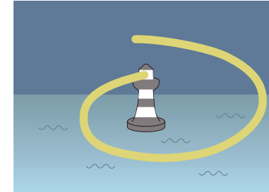
FIGURE 7 A consequence of the finiteness of the speed of light. Watch out for the tricky details – light does travel straight from the source, it does not move along the drawn curved line; the same occurs for water emitted by a rotating water sprinkler.
