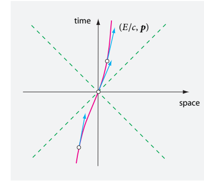
FIGURE 48 Energy–momentum is tangent to the world line.
