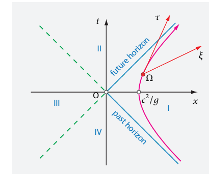
FIGURE 55 The hyperbolic motion of an observer \Omega that accelerates rectilinearly and uniformly with acceleration g .
