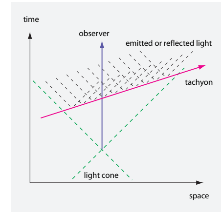
FIGURE 38 Hypothetical space-time diagram for tachyon observation.
