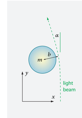
FIGURE 68 Calculating the bending of light by a mass.
