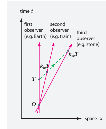
FIGURE 20 How to deduce the composition of velocities.
