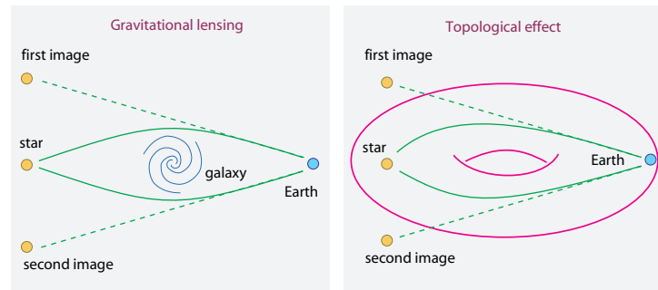
FIGURE 111 Two ways in which a single star can lead to several images.
