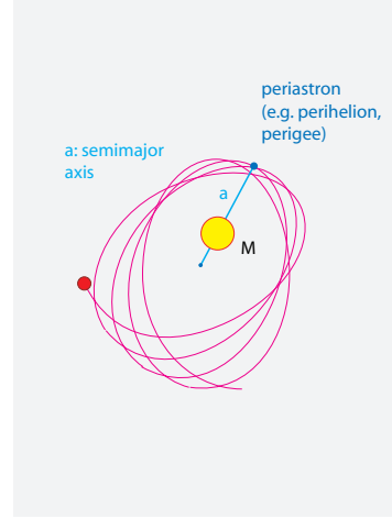
FIGURE 70 The orbit around a central body in general relativity.
