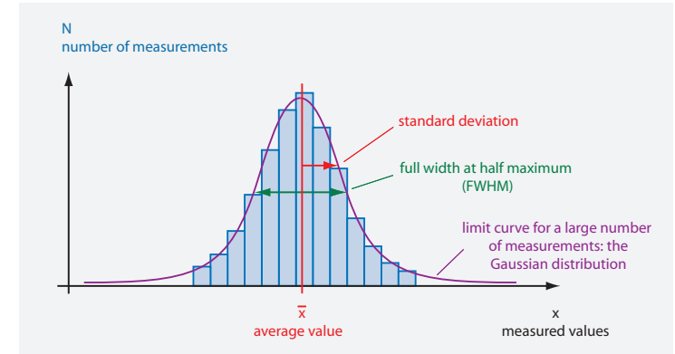
FIGURE 123 A precision experiment and its measurement distribution. The precision is high if the width of the distribution is narrow; the accuracy is high if the centre of the distribution agrees with the actual value.
