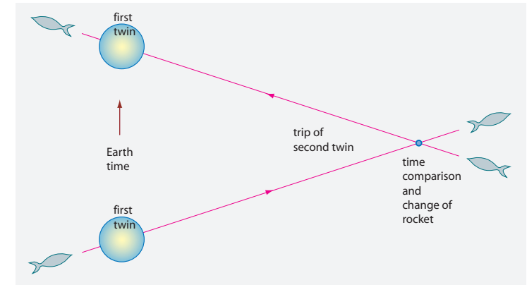
FIGURE 25 The twin paradox.
