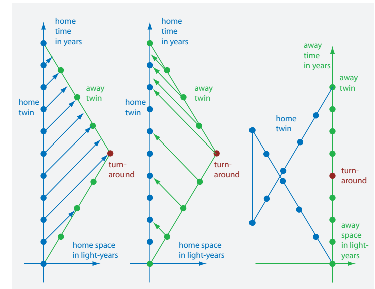
FIGURE 125 The twin paradox: (left and centre) the clock timing for both twins with the signals sent among the twins in the inertial frame of the home twin, and (right) the description by the away twin, in a frame that, however, is not inertial.
