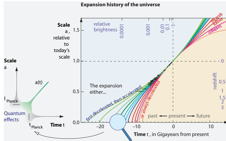
FIGURE 104 The evolution of the universe's scale a for different values of its mass density, as well as the measured data (the graph on the right is courtesy of Saul Perlmutter and the Supernova Cosmology Project).
