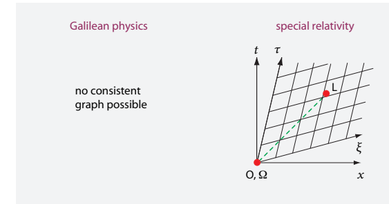
FIGURE 23 The space-time diagram for light seen from two inertial observers, using coordinates (t, x) and (\tau, \xi) .
