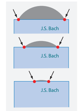
FIGURE 37 Another example of faster-than-light motion.
