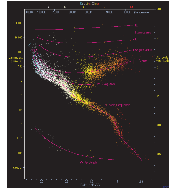
FIGURE 101 The Hertzsprung–Russell diagram (© Richard Powell).
