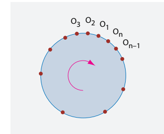
FIGURE 50 Observers on a rotating object.
