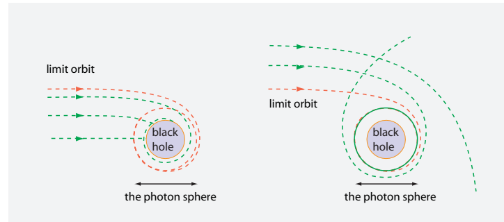
FIGURE 118 Motions of light passing near a non-rotating black hole.
