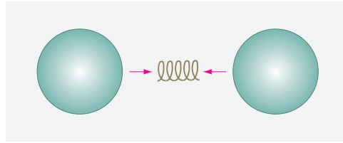
FIGURE 76 A Gedanken experiment showing the necessity of gravitational waves.
