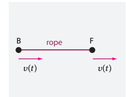
FIGURE 30 What happens to the rope?
