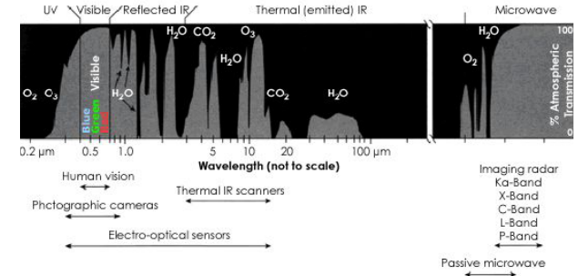
FIGURE 109 The transmittance of the atmosphere (NASA).
