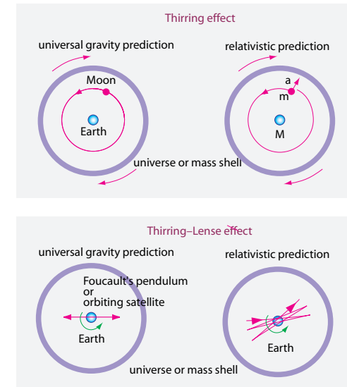
FIGURE 73 The Thirring and the Thirring-Lense effects.
