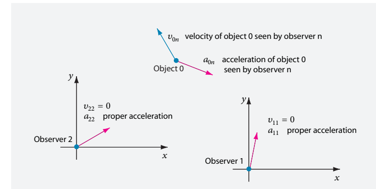
FIGURE 58 The definitions necessary to deduce the composition behaviour of accelerations.
