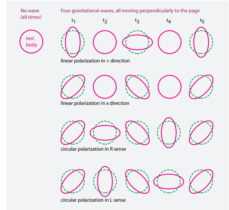
FIGURE 77 Effects on a circular or spherical body due to a plane gravitational wave moving in a direction perpendicular to the page.
