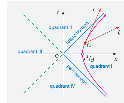
FIGURE 56 Hyperbolic motion and event horizons.
