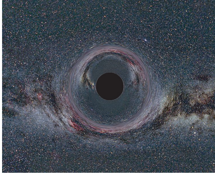
FIGURE 115 A simplified simulated image of how a black hole of ten solar masses, with Schwarzschild radius of 30 km, seen from a constant distance of 600 km, will distort an image of the Milky Way in the background. Note the Zwicky–Einstein ring formed at around twice the black hole radius and the thin bright rim (image © Ute Kraus at www.tempolimit-lichtgeschwindigkeit.de ).
