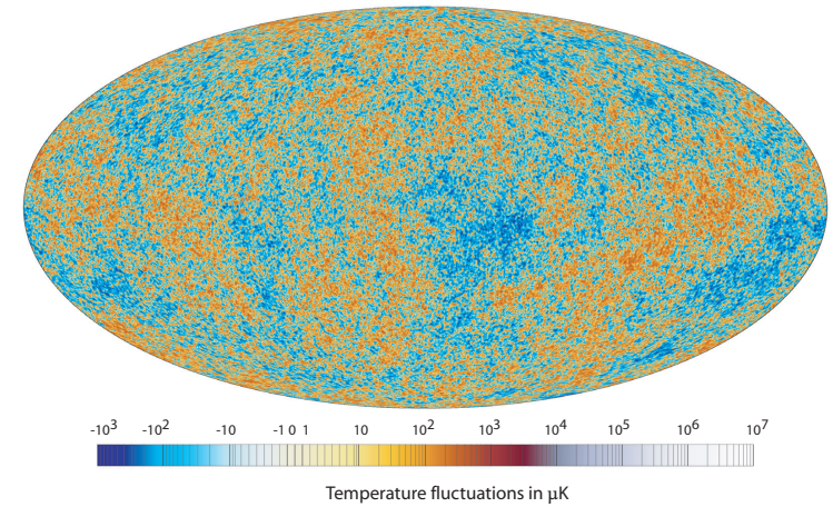
FIGURE 108 A false colour image of the fluctuations of the cosmic background radiation, after the Doppler shift from our local motion and the signals from the Milky Way have been subtracted (© Planck/ESA).
