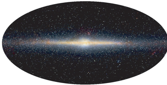
FIGURE 86 A false colour image of how the night sky, and our galaxy in particular, looks in the near infrared (courtesy NASA).
