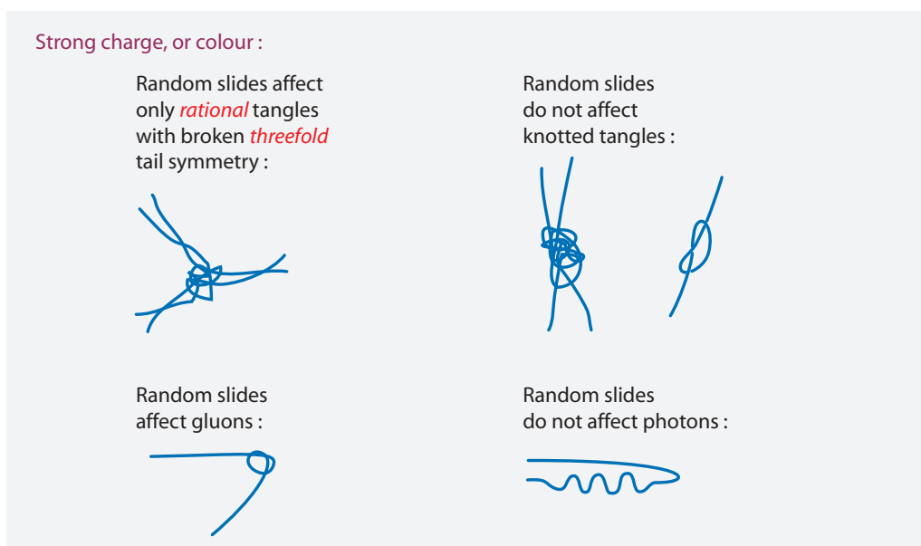
FIGURE 72 Tangles with and without colour charge. (This image needs to be updated: no knotted tangles occur in nature.)
