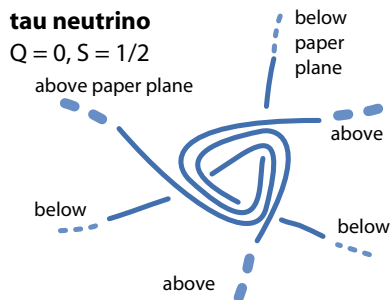
FIGURE 128 The simplest tangle models for the elementary fermions. Elementary fermions are described by rational, i.e., unknotted tangles. Their structures lead to coupling to the Higgs, as illustrated in Figure 130, produce positive mass values, and limit the number of generations to 3. Each fermion is represented by a tangle family , consisting of the simplest member and of tangles with added Higgs braids. The tangles determine the specific fermion propagators, including the values of masses and mixing angles. The tethers of the quark tangles follow the axes of a tetrahedron. The neutrino cores are simpler when seen in three dimensions: they are twisted triples of strands. The tethers of all lepton tangles approach the three coordinate axes at large distances from the core. No additional elementary fermions appear to be possible.
