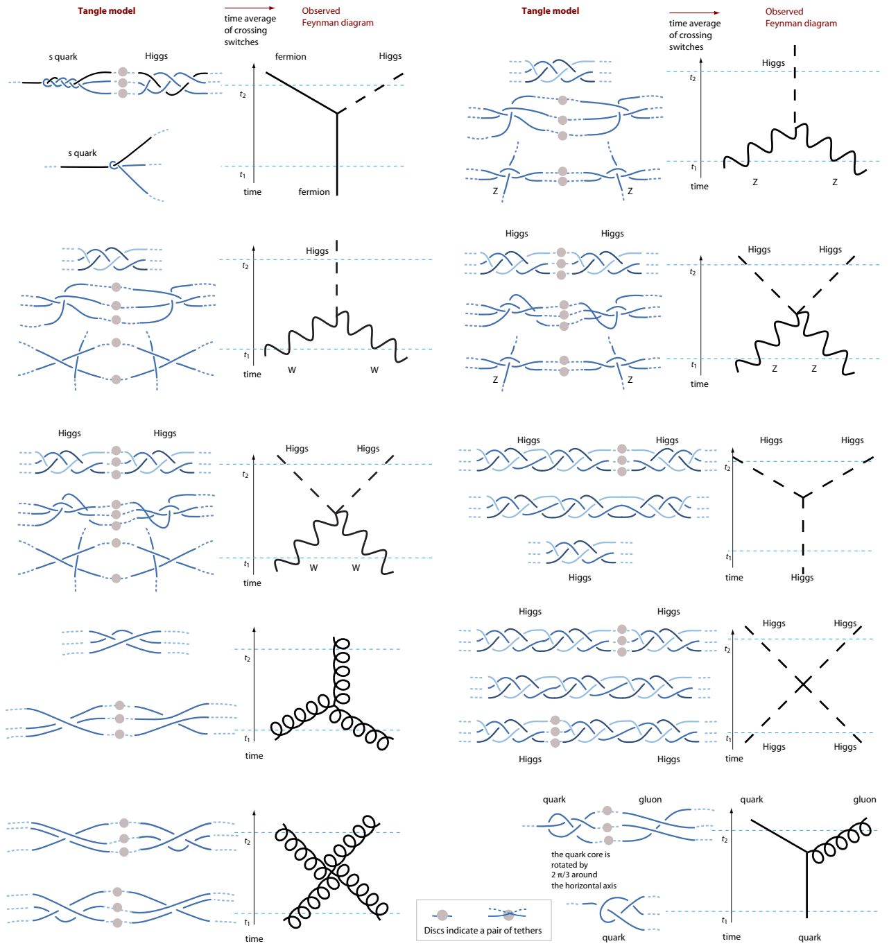
FIGURE 130 The vertices in Feynman diagrams allowed by the topology of the fermion and boson tangles (part two).
