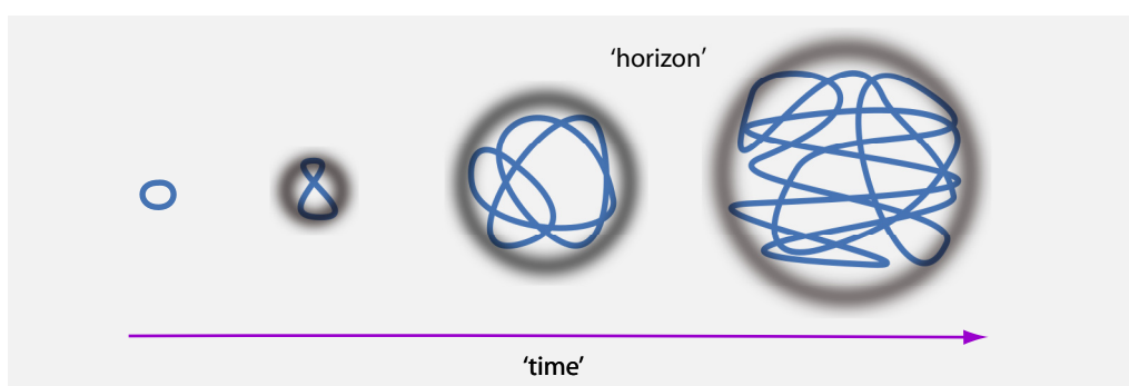
FIGURE 82 An extremely simplified view of how the universe evolved near the big bang. In this evolution, physical time, space and the surrounding horizon are in the process of getting defined.
