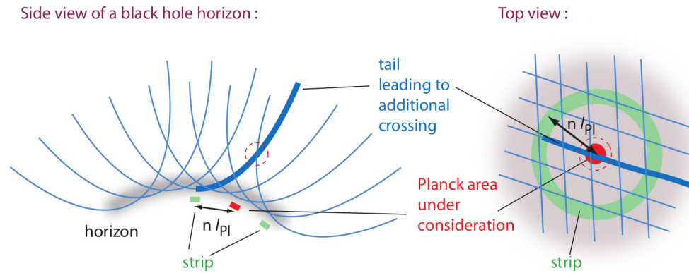
FIGURE 78 The entropy of black holes results from the number of possible crossing states above a Planck area.
