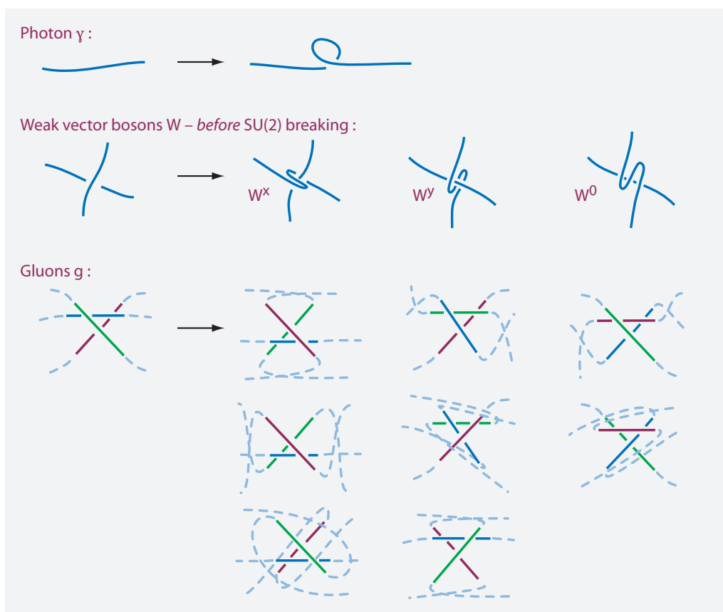
FIGURE 84 The gauge bosons in the strand model. All differ from vacuum by one curved strand – though, for clarity, the gluons are shown here using their complementary two-strand moves.
