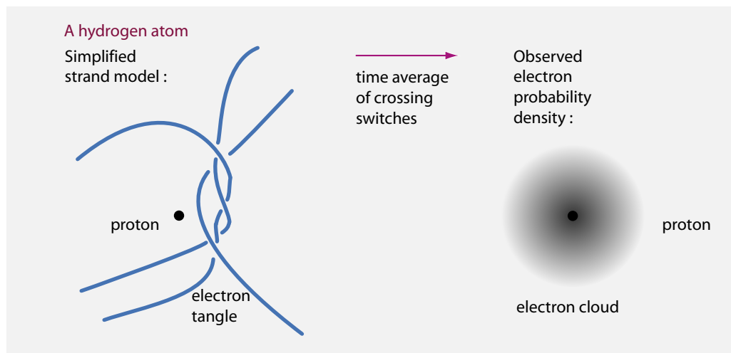
FIGURE 46 A simple, quantum-mechanical view of a hydrogen atom.
