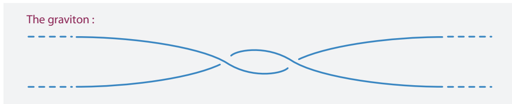
FIGURE 90 The graviton in the strand model.
