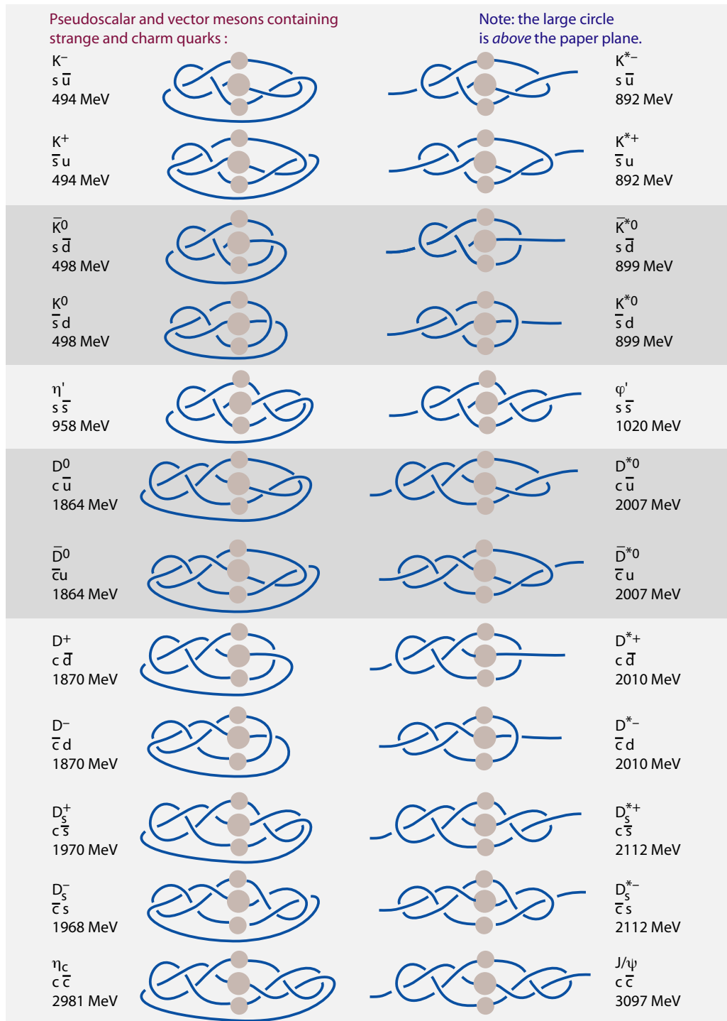
FIGURE 99 The simplest strand models for strange and charmed mesons with vanishing orbital angular momentum. Mesons on the left side have spin 0 and negative parity; mesons on the right side have spin 1 and also negative parity. Circles indicate crossed tail pairs to the border of space; grey boxes indicate tangles that mix with their antiparticles and which are thus predicted to show CP violation.
