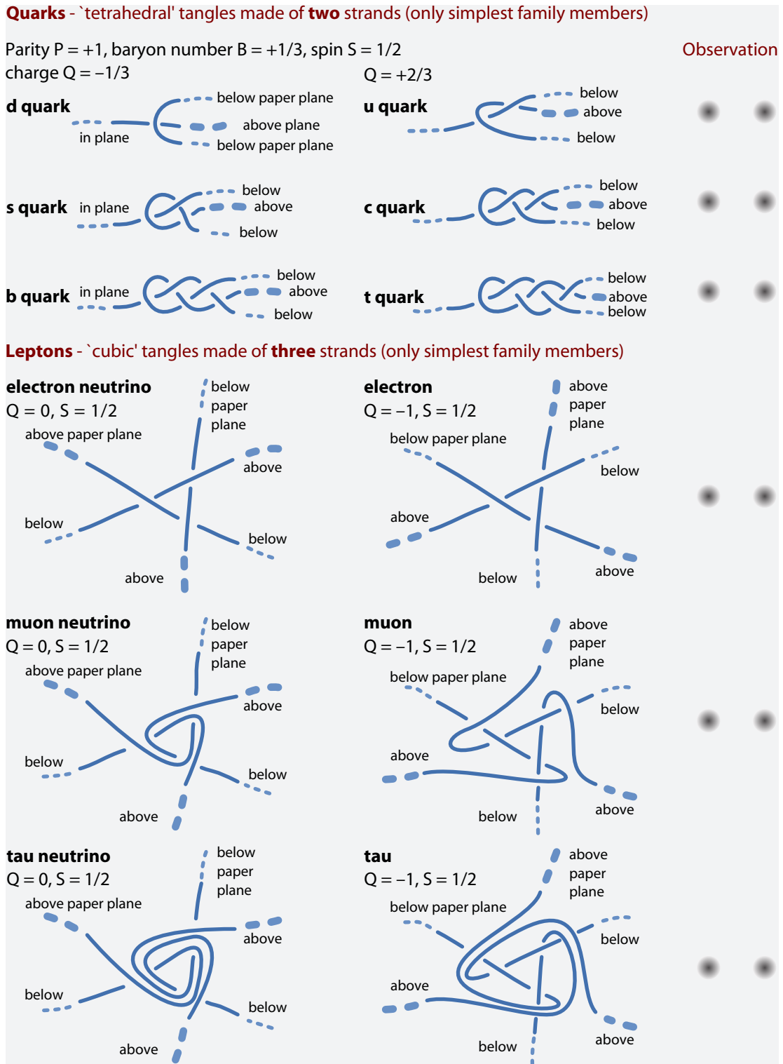
FIGURE 111 Elementary fermions are described by rational, i.e., unknotted tangles. Their structures lead to coupling to the Higgs, as illustrated in Figure 130, produce positive mass values, and limit the number of generations to 3. The tangles determine the specific fermion propagators. The tethers of the quark tangles follow the axes of a tetrahedron. The neutrino cores are simpler when seen in three dimensions: they are simply twisted triples of strands. The tethers of all lepton tangles approach the three coordinate axes at large distances from the core. No additional elementary fermions appear to be possible.
