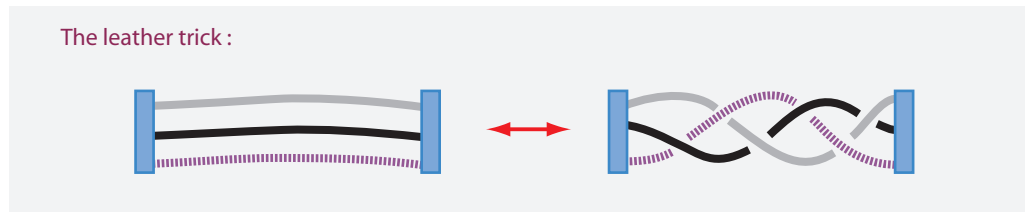
FIGURE 89 The leather trick is the deformation process that changes these two structures into each other. The leather trick limits structures made of three-stranded braids to six basic types.
