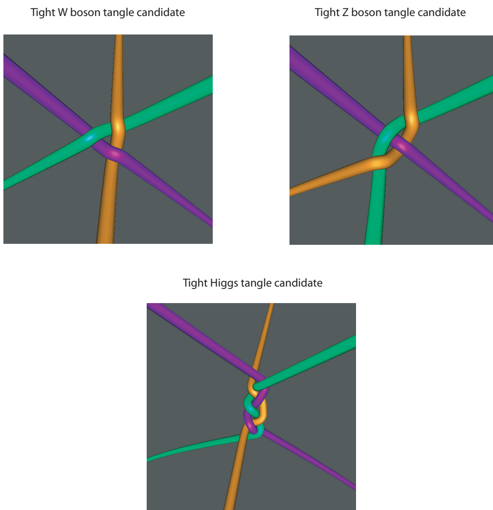
FIGURE 112 Tight tangle candidates (of 2015/2016) for the simplest tangles of the W, the Z and the Higgs bosons. In contrast to the pictures, the W and Z tails lie in a plane.
