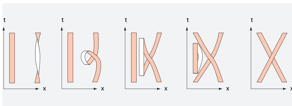
FIGURE 70 Belts in space-time: rotation and antiparticles.
