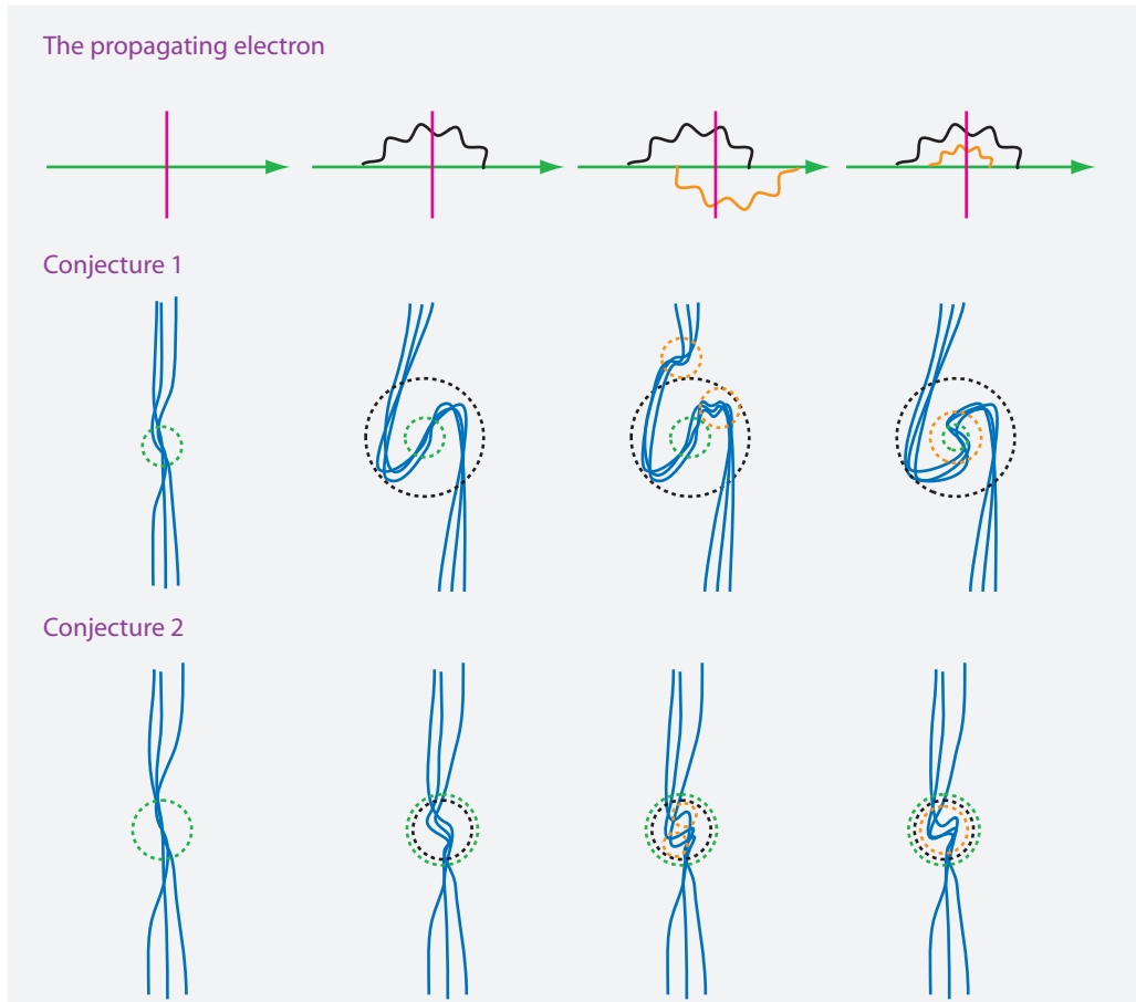
FIGURE 60 Two conjectured correspondences between the Feynman diagrams of quantum electrodynamics and the strand model for a propagating free electron. The lower strand model configurations are shown for a single instant – marked in magenta – of the electron propagator drawn above them. (For simplicity, the external field is not drawn.) In the first conjecture, the loops of the belt trick are conjectured to correspond to the virtual photons in the propagator and to be responsible for the anomalous magnetic moment. In the second conjecture, the deformations of the core correspond to the virtual photons.
