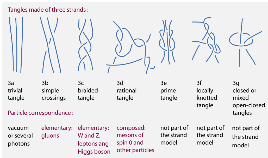
FIGURE 91 Examples for all the classes of tangles made of three strands.
