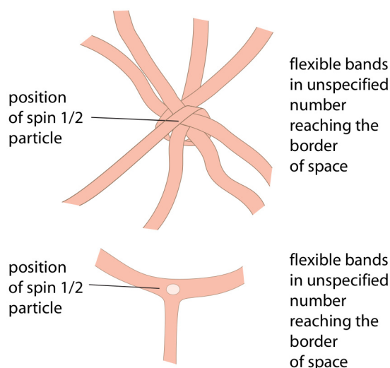
FIGURE 9 Possible models for a spin 1/2 particle.
