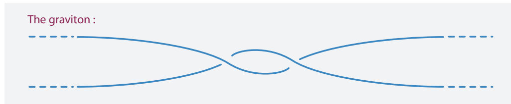
FIGURE 78 The graviton in the strand model: a twist in a pair of tethers.
