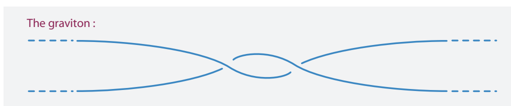
FIGURE 89 The graviton in the strand model.
