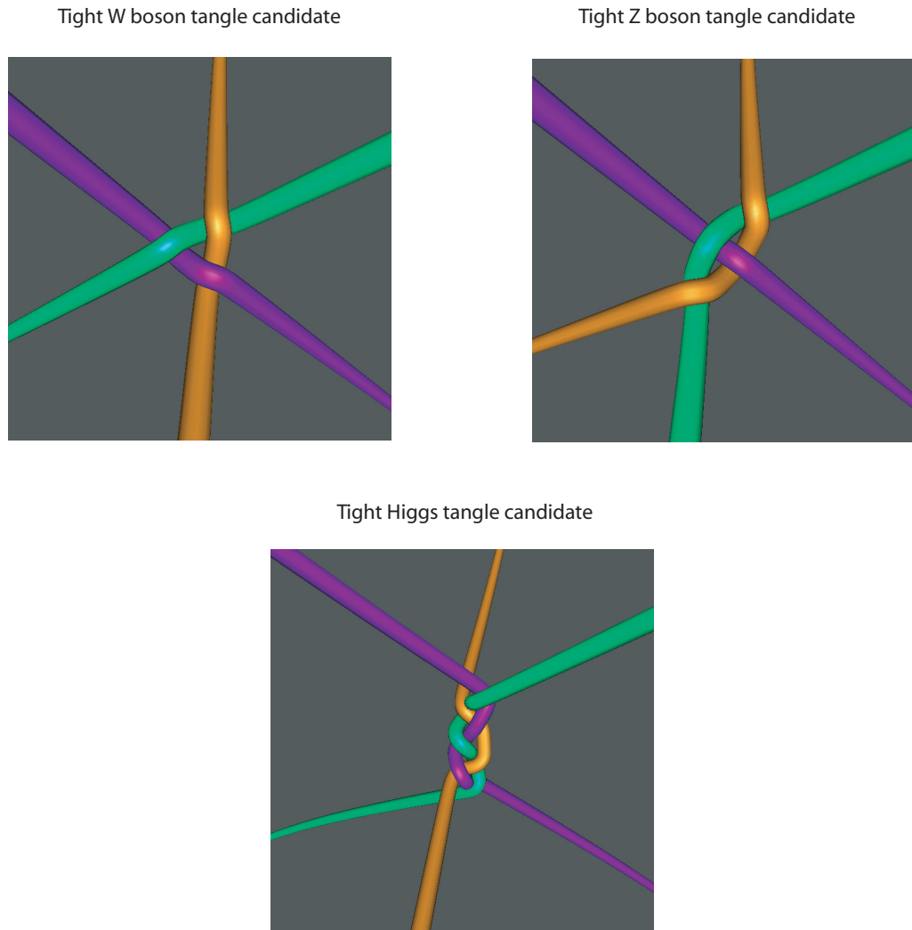
FIGURE 111 Tight tangle candidates (of 2015/2016) for the simplest tangles of the W, the Z and the Higgs bosons. In contrast to the pictures, the W and Z tails lie in a plane.
