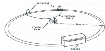
FIGURE 24 The original experimental set-up with which Hanbury Brown and Twiss measured stellar diameters at Narrabri in Australia. The distance between the two light collectors could be changed by moving them on rails. The light detectors are at the end of the poles and each of them, as they wrote, ‘collected light as rain in a bucket.’ (© John Davis).
