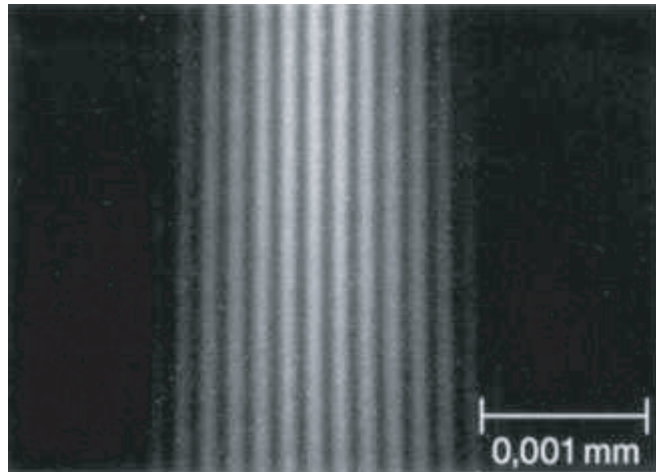
FIGURE 38 Electron beams diffract and interfere at multiple slits (© Claus Jönsson).
